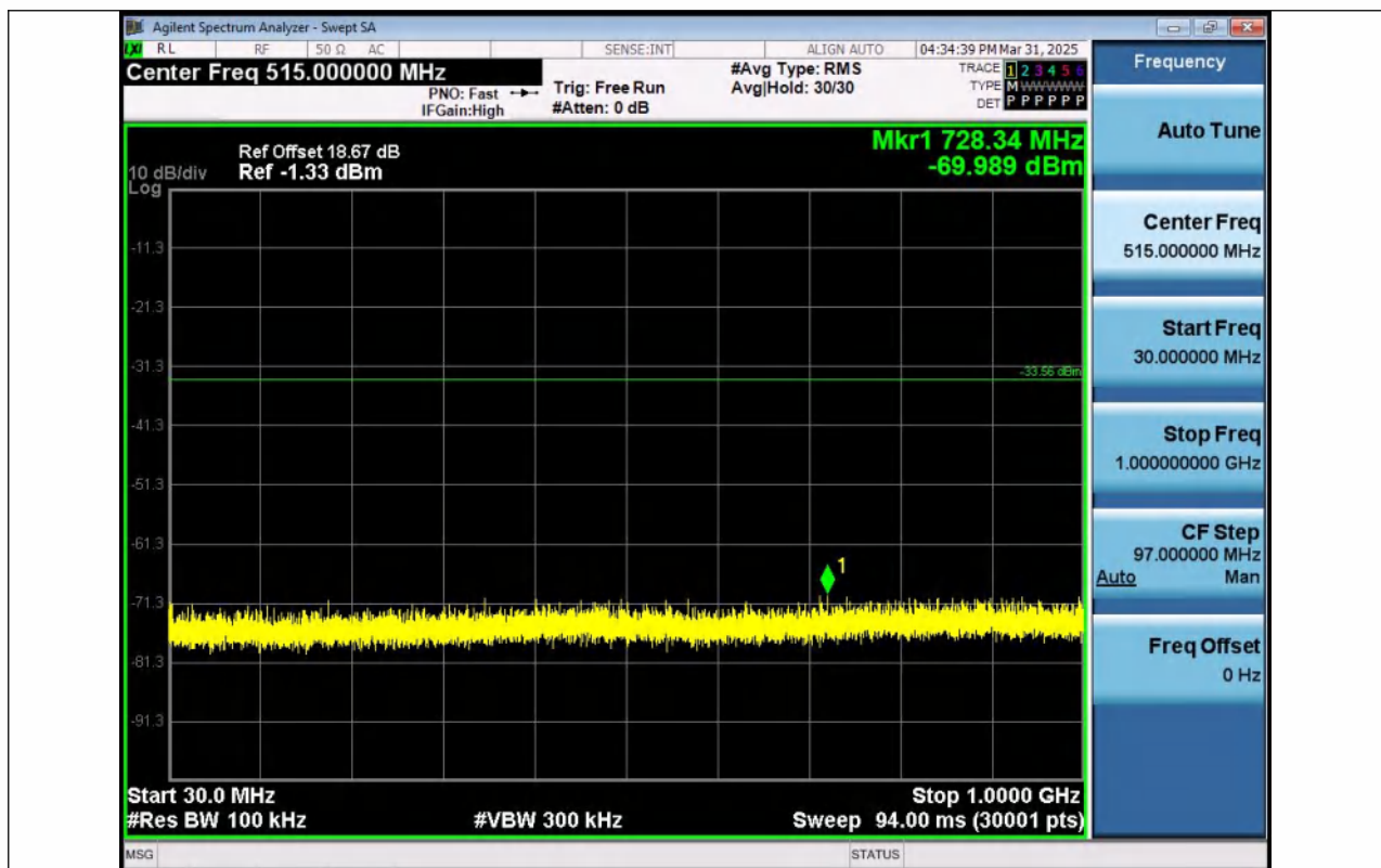
11N40SISO-Ant1-2452-30~1000-PASS
