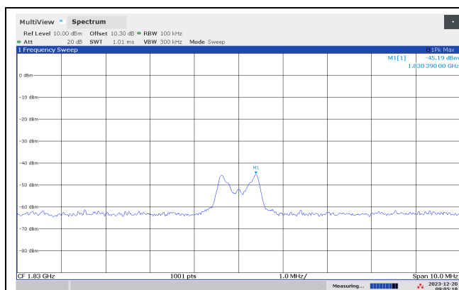
Conducted Emissions 1830 MHz, 915 MHz
