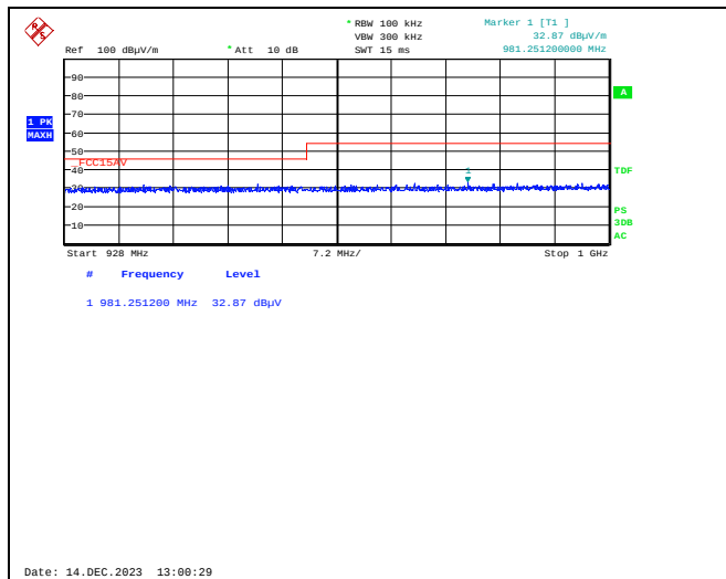
Radiated Emissions 928 - 1000 MHz, 915.00 MHz HP
