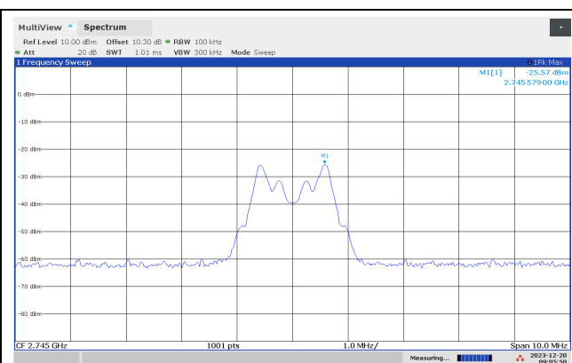
Conducted Emissions 2745 MHz, 915 MHz
