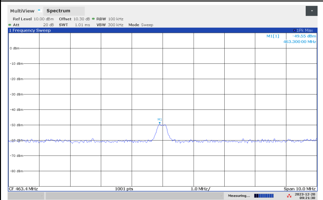
Conducted Emissions 463.4 MHz, 926.75 MHz
