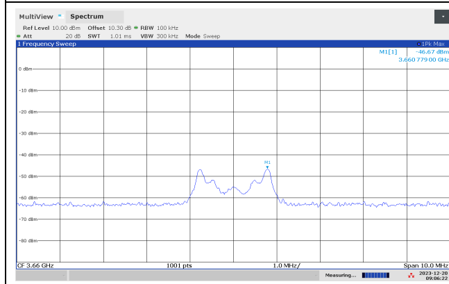
Conducted Emissions 3660 MHz, 915 MHz
