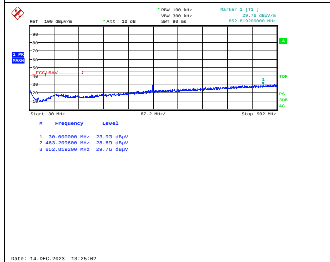
Radiated Emissions 30 - 902 MHz, 926.75 MHz HP
