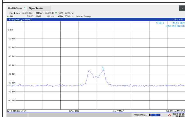
Conducted Emissions 1853.5 MHz, 926.75 MHz
