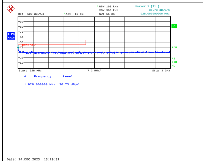
Radiated Emissions 928 - 1000 MHz, 926.75 MHz HP
