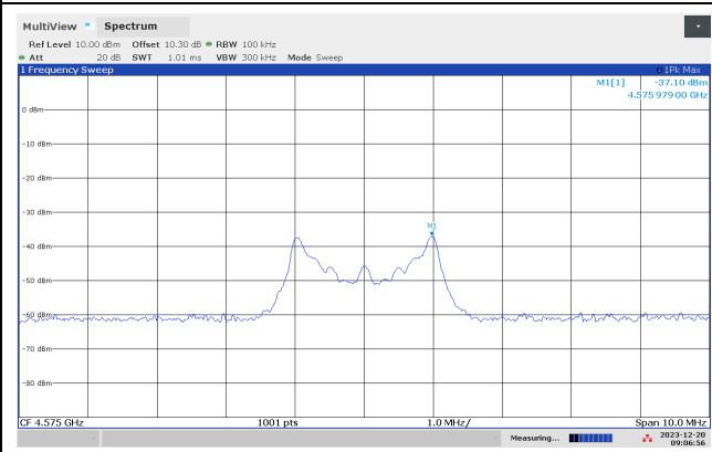
Conducted Emissions 4575 MHz, 915 MHz
