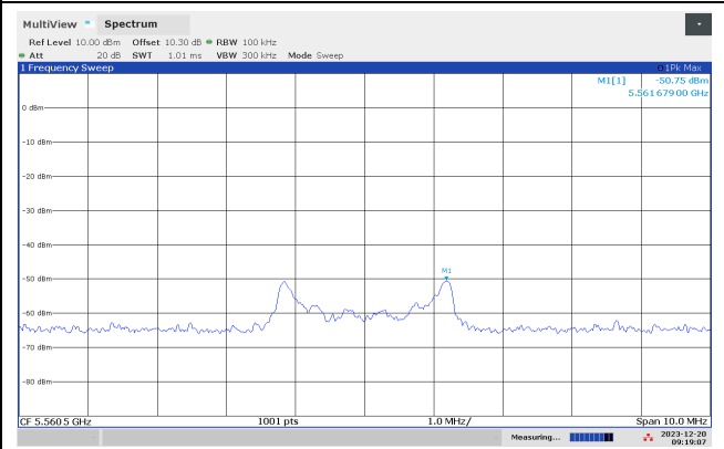
Conducted Emissions 5560.5 MHz, 926.75 MHz
