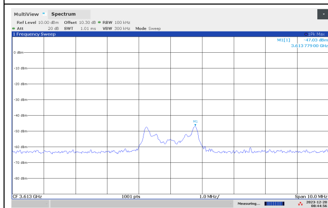
Conducted Emissions 3613 MHz, 903.25 MHz
