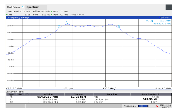
DTS BW, 915.0 MHz
