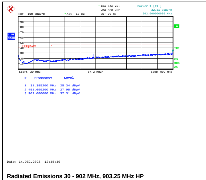
Radiated Emissions 30 - 902 MHz, 903.25 MHz HP
