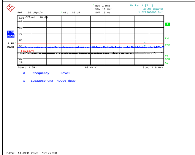
Radiated Emissions 1 - 1.6 GHz, 926.75 MHz, HP
