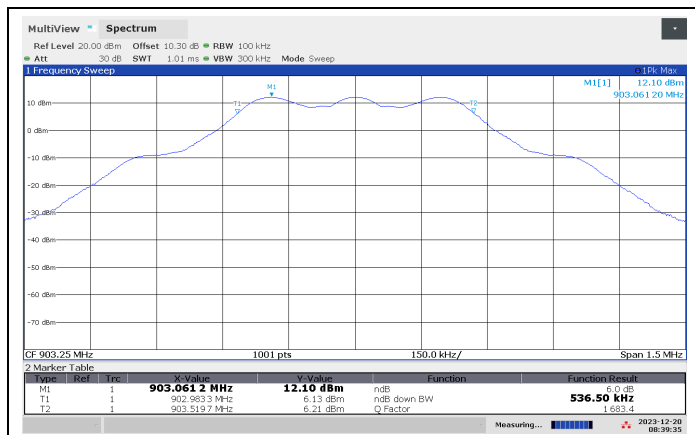
DTS BW, 903.25 MHz
