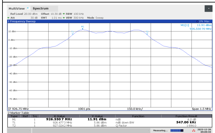
DTS BW, 926.75 MHz
