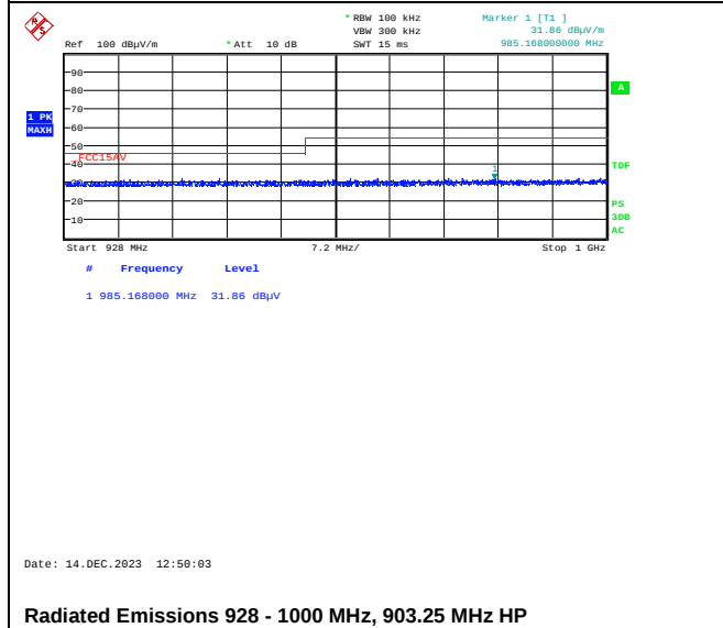
Radiated Emissions 928 - 1000 MHz, 903.25 MHz HP
