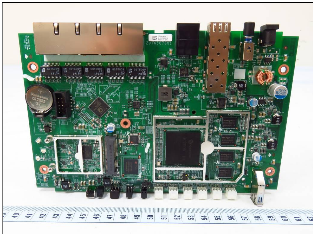
1st DDR
