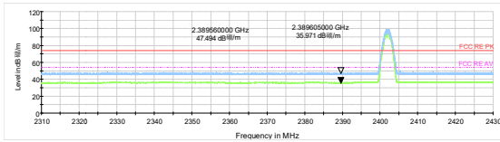
DH5-Channel 0: Peak + Average
