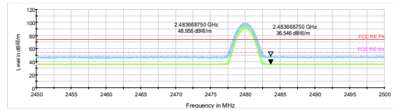
3DH5-Channel 78: Peak + Average
