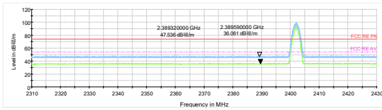
3DH5-Channel 0: Peak + Average
