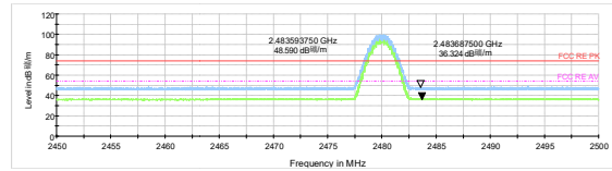
DH5-Channel 78: Peak + Average
