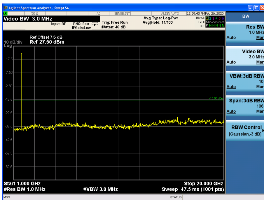
Channel 1412, 1GHz~20GHz
