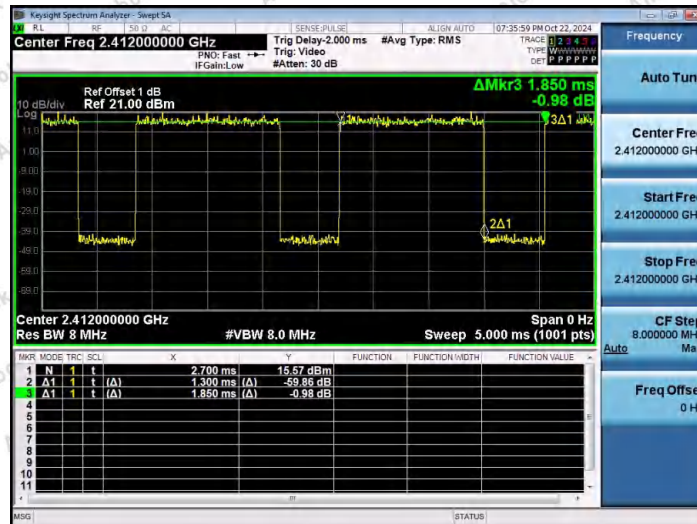
NTVN-11N20SISO-Ant1-2412
