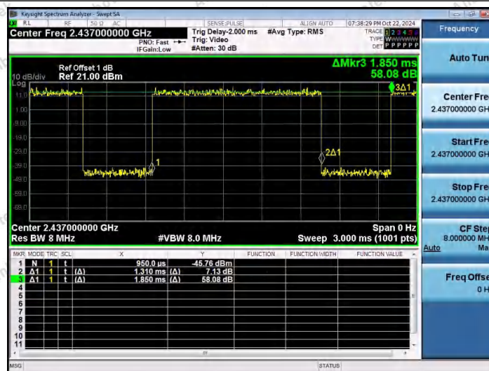
NTVN-11N20SISO-Ant1-2437
