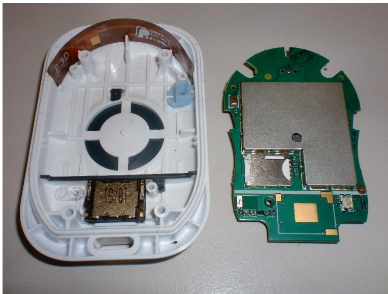
Module removed from enclosure – back side
