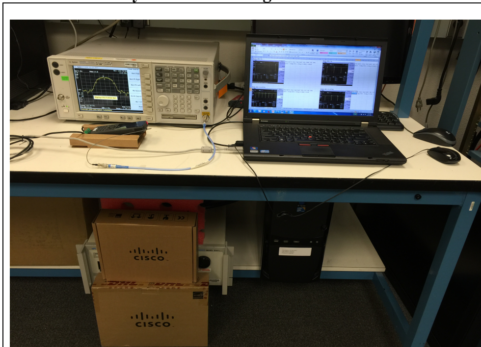
Title: RF Conducted Test Setup
