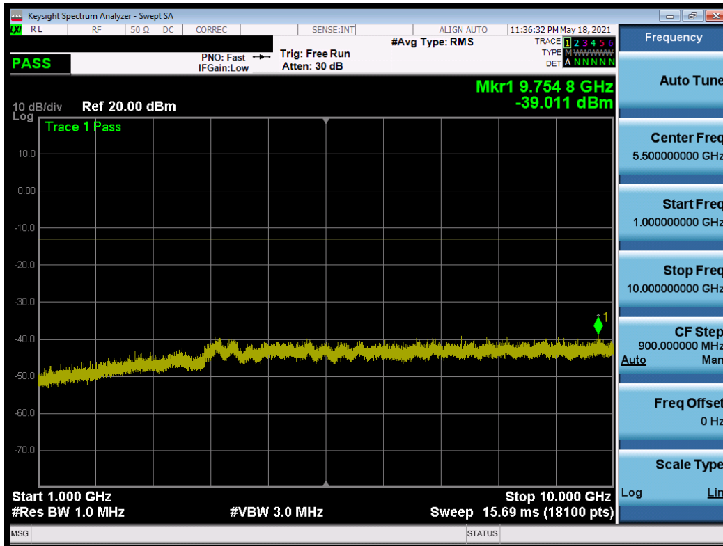
Plot 7-19. Conducted Spurious Plot – Mid Channel (1.4MHz, QPSK, 1RB, RB Offset 0)
