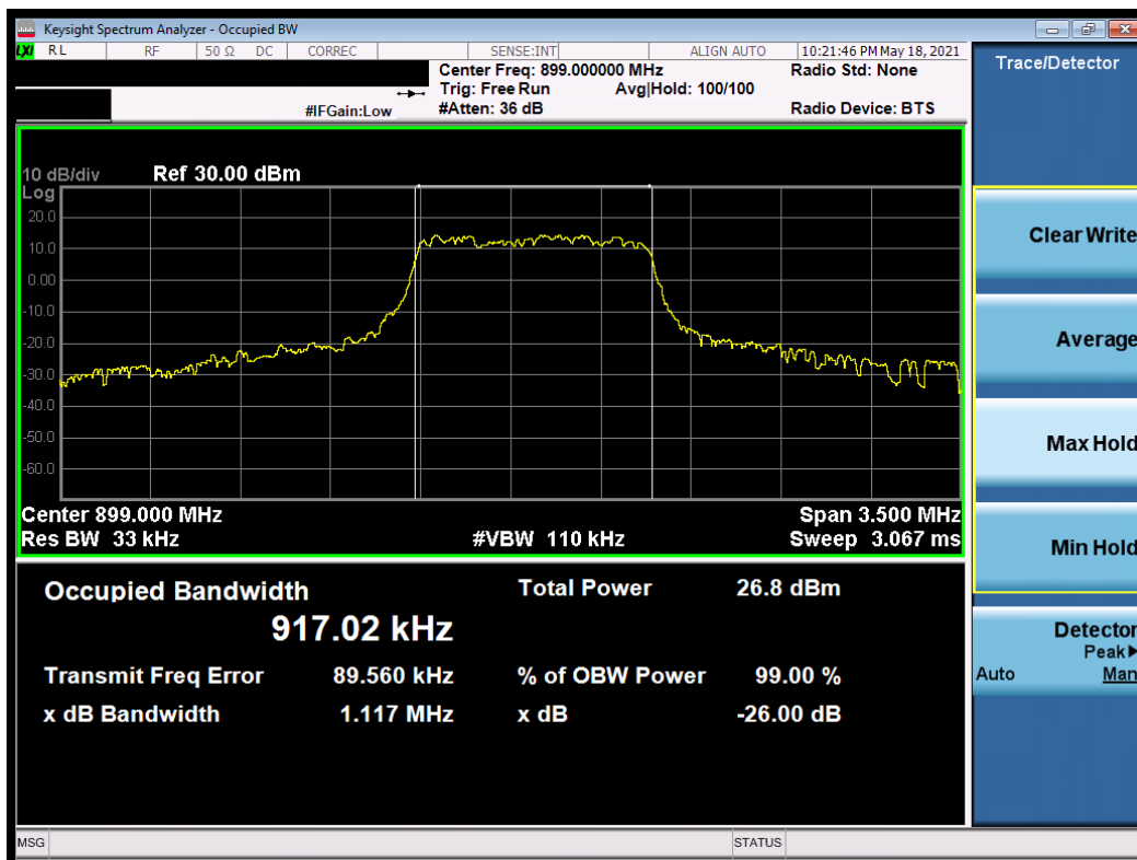
Plot 7-9. Occupied Bandwidth Plot (1.4MHz, 16-QAM, RB 5, RB Offset 1, NB=0)
