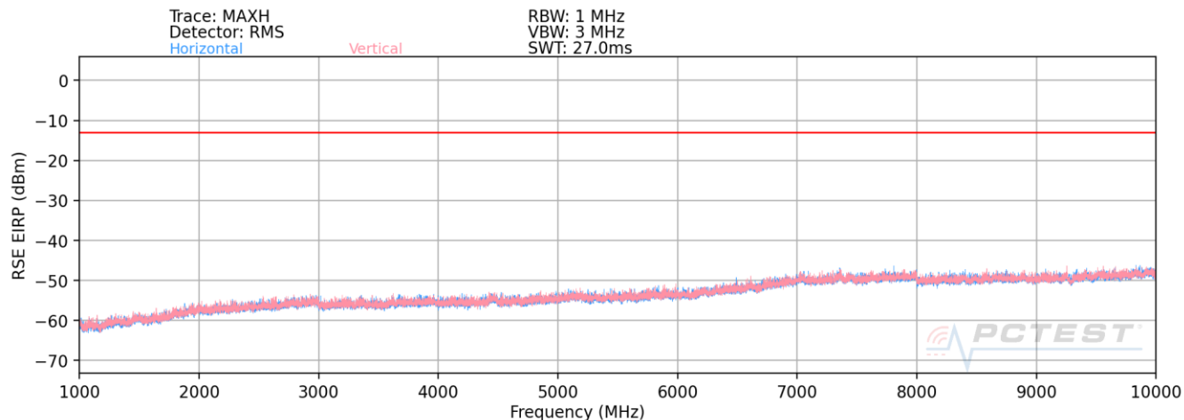
Plot 7-31. Radiated Spurious Plot (LTE Band 8- CAT-M1)
