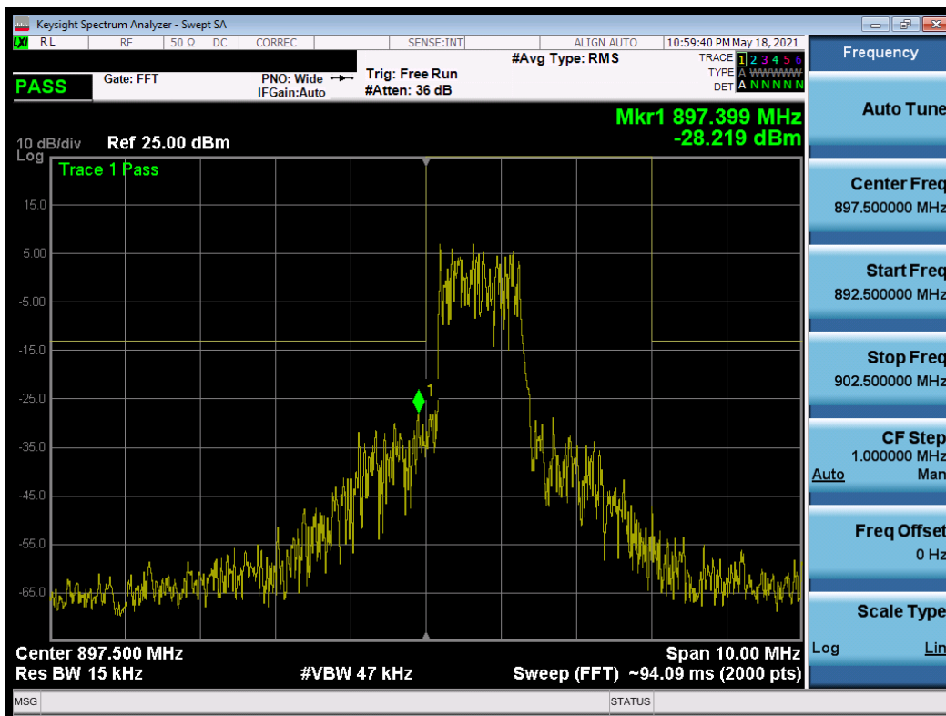
Plot 7-12. Lower Band Edge Plot (1.4MHz, QPSK, 6RB, RB Offset 0, NB=0)
