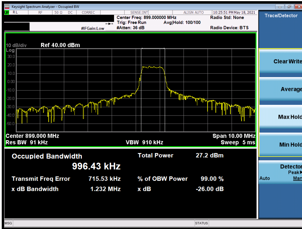
Plot 7-6. Occupied Bandwidth Plot (3MHz, 16-QAM, RB 5, RB Offset 1, NB=1)
