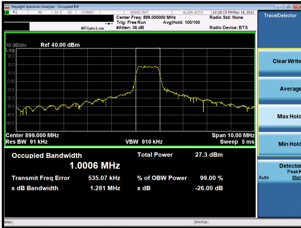
Plot 7-4. Occupied Bandwidth Plot (3MHz, 16-QAM, RB 5, RB Offset 0, NB=1)
