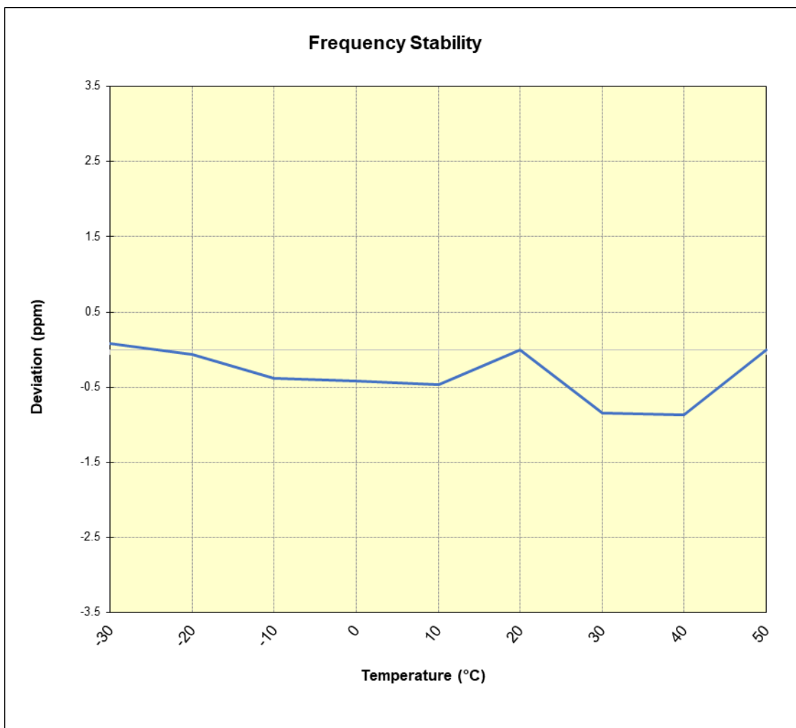
Plot 7-32. LTE Band 8 CAT-M1 Frequency Stability Chart
