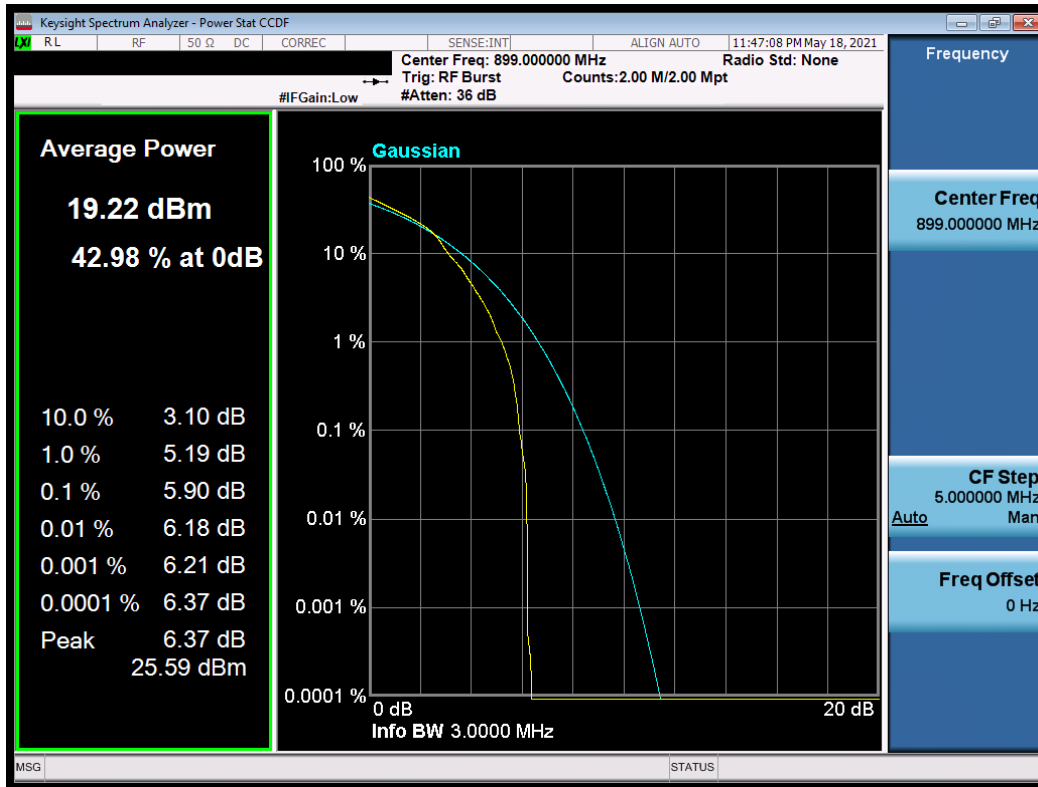
Plot 7-26. Peak to Average Ratio (3MHz, 16-QAM, RB 5, RB Offset 1, NB=0)
