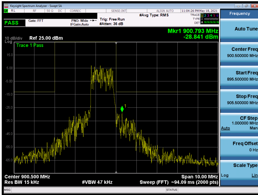
Plot 7-13. Upper Band Edge Plot (1.4MHz, QPSK, 6RB, RB Offset 0, NB=0)
