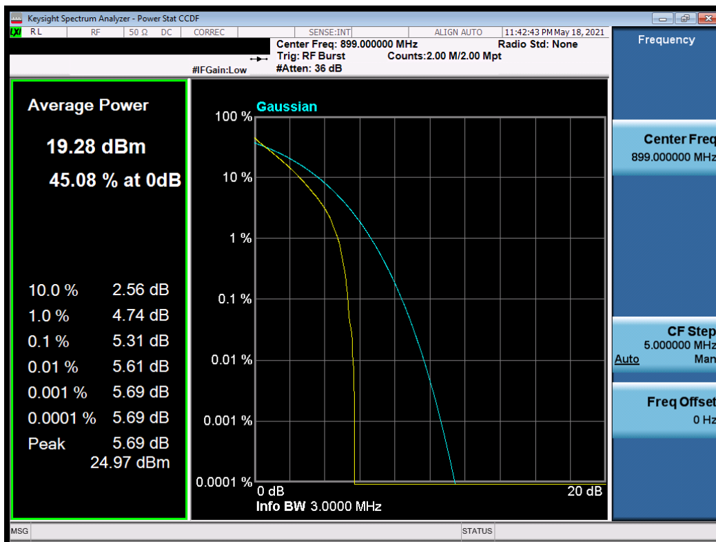
Plot 7-23. Peak to Average Ratio (3MHz, QPSK, RB 6, RB Offset 0, NB=1)
