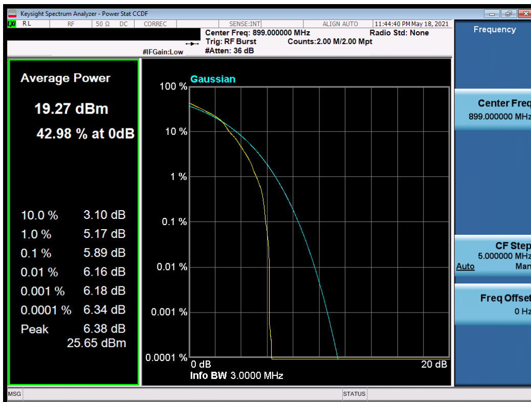
Plot 7-27. Peak to Average Ratio (3MHz, 16-QAM, RB 5, RB Offset 1, NB=1)
