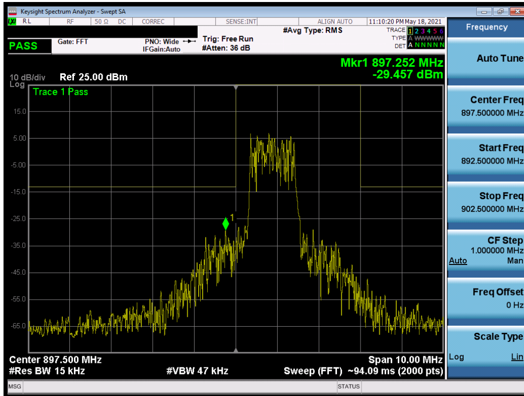
Plot 7-10. Lower Band Edge Plot (3MHz, QPSK, 6RB, RB Offset 0, NB=0)
