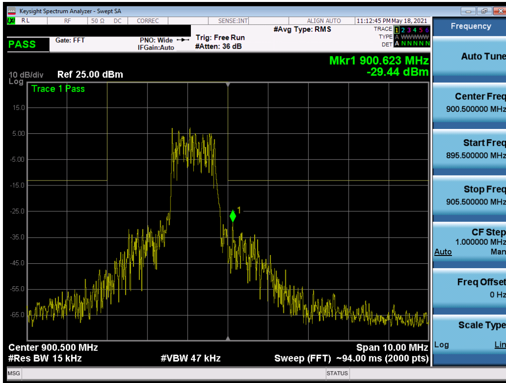
Plot 7-11. Upper Band Edge Plot (3MHz, QPSK, 6RB, RB Offset 0, NB=1)
