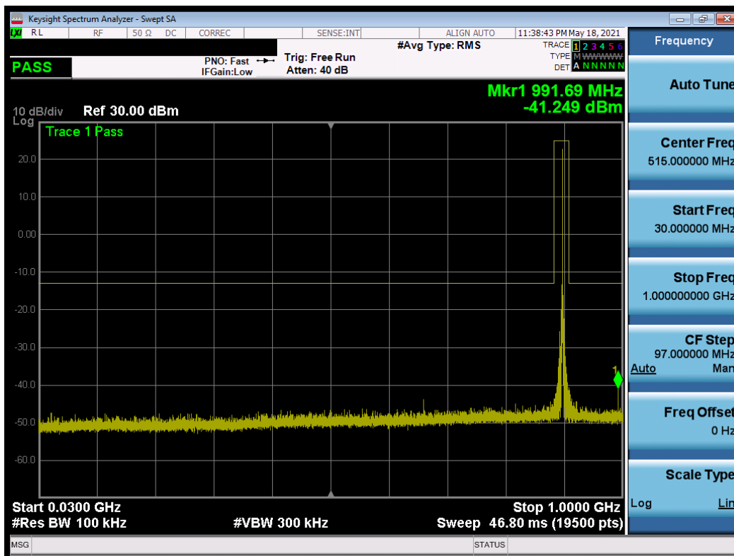
Plot 7-20. Conducted Spurious Plot – High Channel (1.4MHz, QPSK, 1RB, RB Offset 0)
