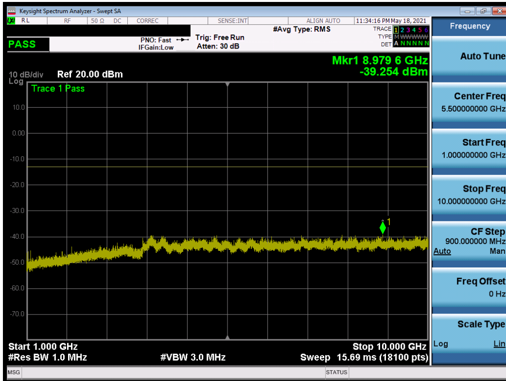
Plot 7-17. Conducted Spurious Plot – Mid Channel (3MHz, QPSK, 1RB, RB Offset 0)
