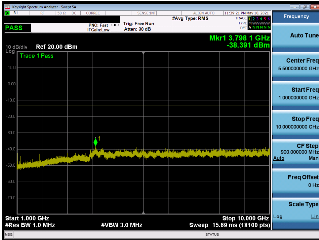
Plot 7-21. Conducted Spurious Plot – High Channel (1.4MHz, QPSK, 1RB, RB Offset 0)
