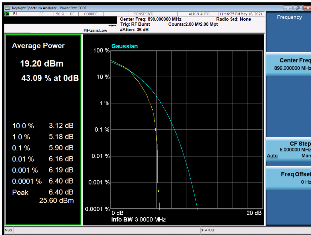
Plot 7-25. Peak to Average Ratio (3MHz, 16-QAM, RB 5, RB Offset 0, NB=1)
