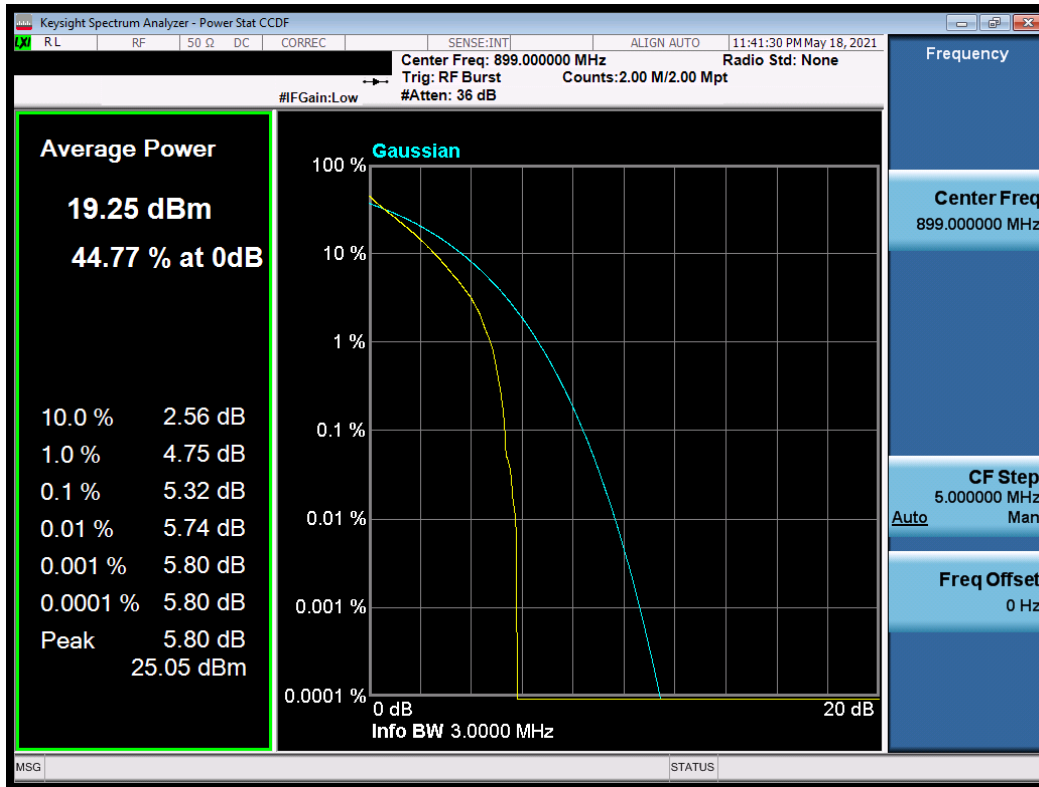
Plot 7-22. Peak to Average Ratio (3MHz, QPSK, RB 6, RB Offset 0, NB=0)
