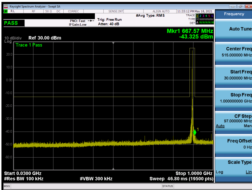
Plot 7-18. Conducted Spurious Plot – Mid Channel (1.4MHz, QPSK, 1RB, RB Offset 0)
