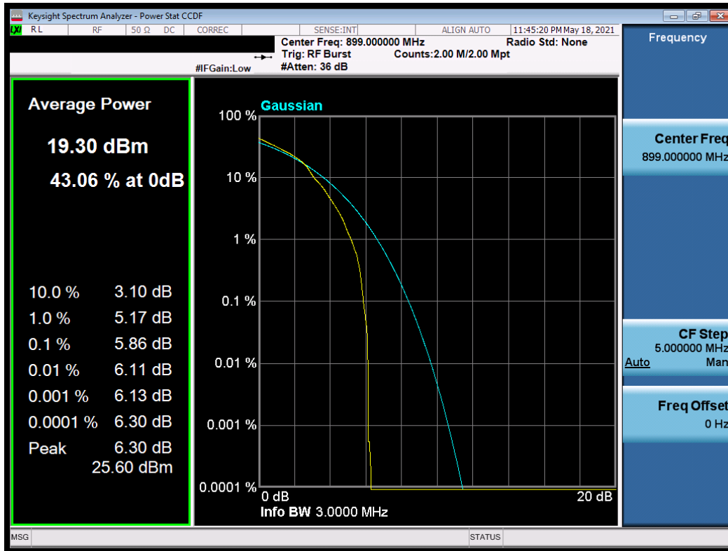
Plot 7-24. Peak to Average Ratio (3MHz, 16-QAM, RB 5, RB Offset 0, NB=0)
