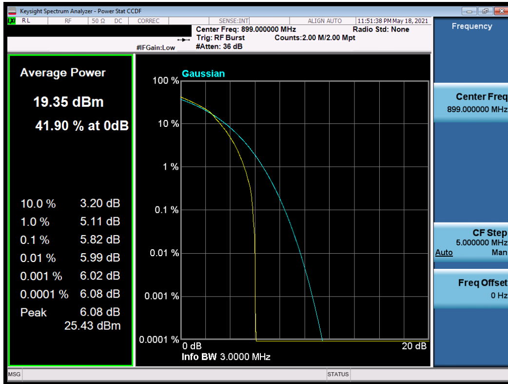
Plot 7-30. Peak to Average Ratio (1.4MHz, 16-QAM, RB 5, RB Offset 1, NB=0)
