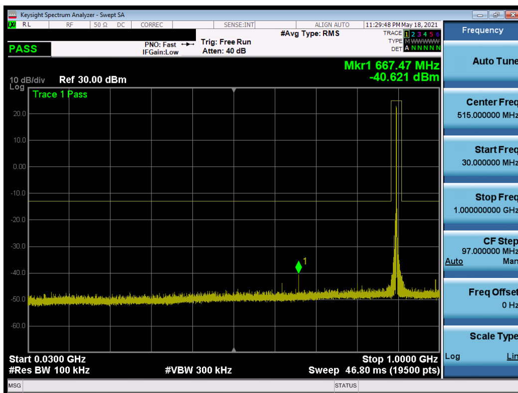
Plot 7-14. Conducted Spurious Plot – Low Channel (1.4MHz, QPSK, 1RB, RB Offset 0)
