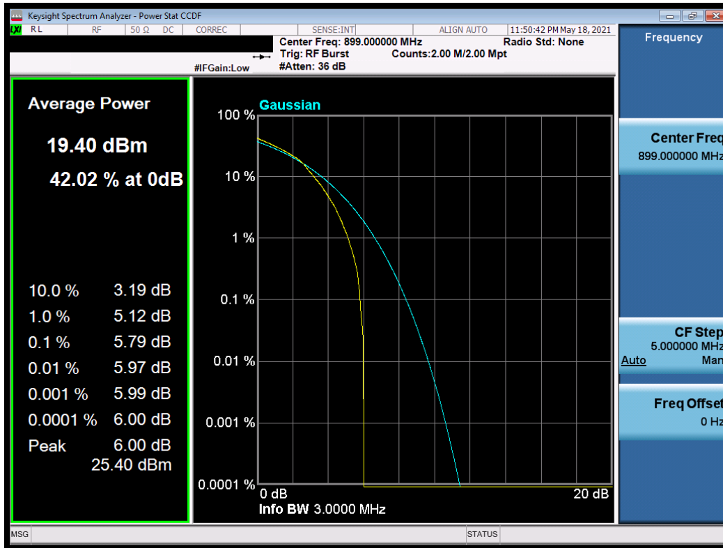
Plot 7-28. Peak to Average Ratio (1.4MHz, QPSK, RB 6, RB Offset 0, NB=0)
