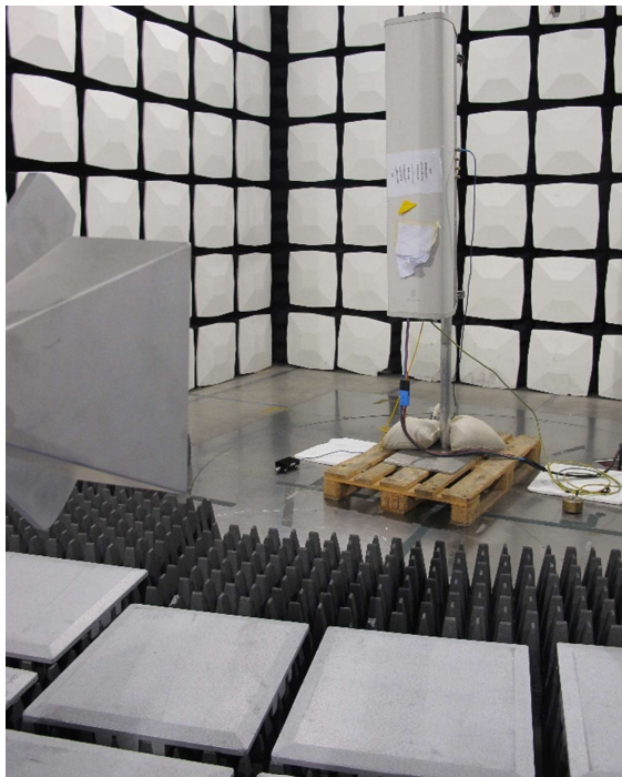
Photos of the test set up
