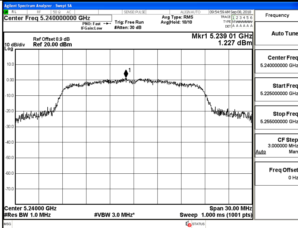
IEEE 802.11a / Channel 48 / 5240 MHz_Ant1
