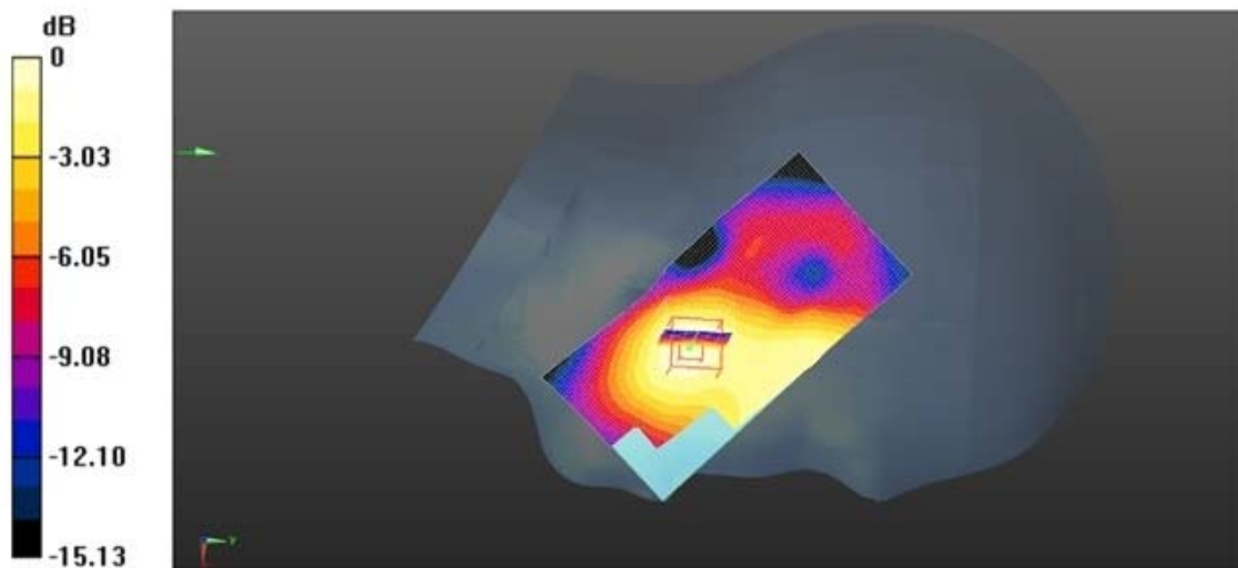
Left Head Cheek (WLAN middle Channel)
