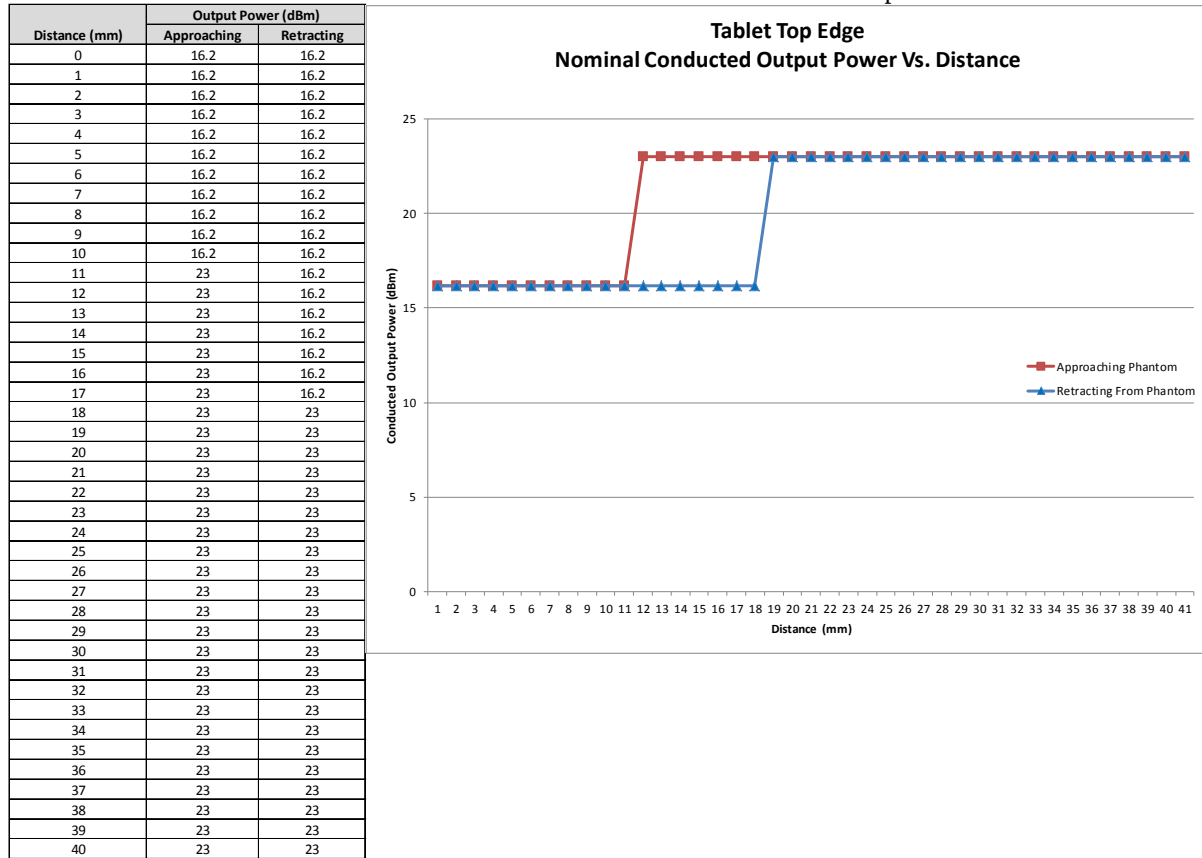
Figure 6: Nominal Output Power vs Trigger Distance – Tablet Top Edge
