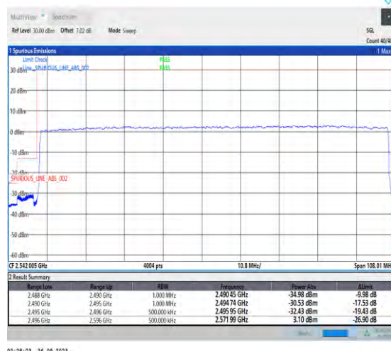
1-N41-PC3-30-100-L-3-DFT-PI2BPSK-Outer_Full-270@0-Ant5-1--PASS-see graph
