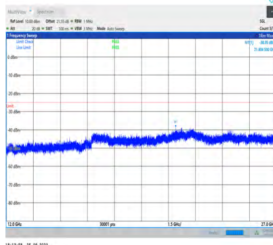
1-N41-PC3-30-100-H-1-DFT-PI2BPSK-Inner_1RB_ Left-1@1-12000-27000-Ant5-21404.50--38.95--25-PA SS
