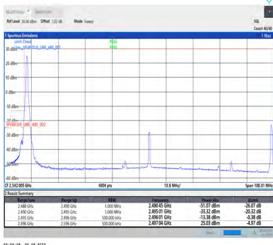
1-N41-PC3-30-100-L-1-DFT-PI2BPSK-Edge_1RB_Left-1@0-Ant5-1--PASS-see graph
