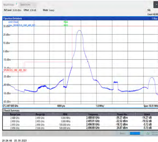
1-N41-PC3-30-10-L-1-DFT-PI2BPSK-Edge_1RB_Left-1@0-Ant5-1--PASS-see graph
