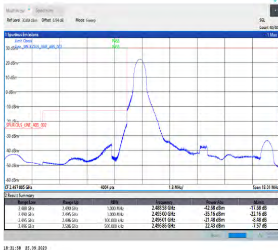
1-N41-PC3-30-10-L-4-CP-QPSK-Edge_1RB_Left-1@0-Ant5-1--PASS-see graph
