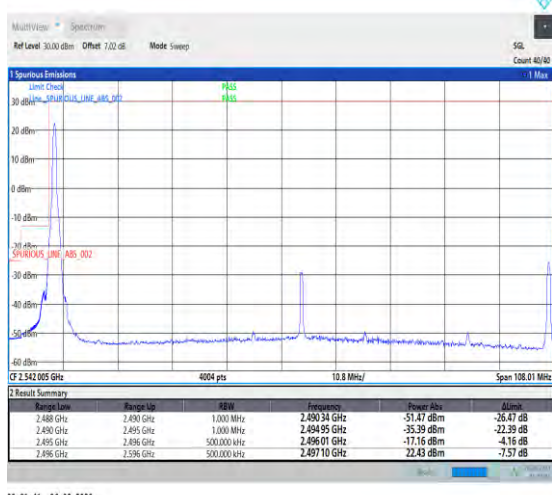
1-N41-PC3-30-100-L-4-CP-QPSK-Edge_1RB_Left-1@0-Ant5-1--PASS-see graph
