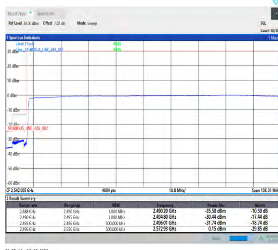
1-N41-PC3-30-100-L-6-CP-QPSK-Outer_Full-273@0-Ant5-1--PASS-see graph
