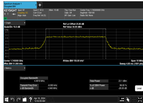
N66(5M)_CP-OFDM_256 QAM_Outer_Full_Mid_CH
