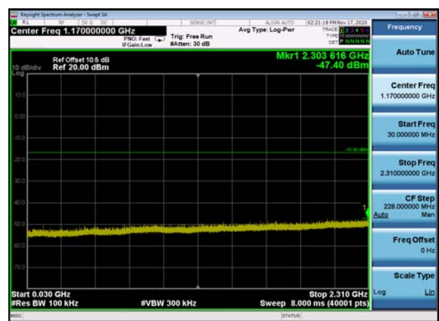
,Plot 3,30MHz~2310MHz-802.11g,2462MHz
