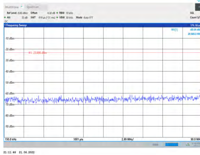
Band26-15MHz-QPSK-26865-1RB#0-Range2:0.15~30MHz
