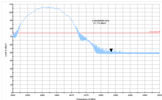
802.11b-Channel 11 Peak
