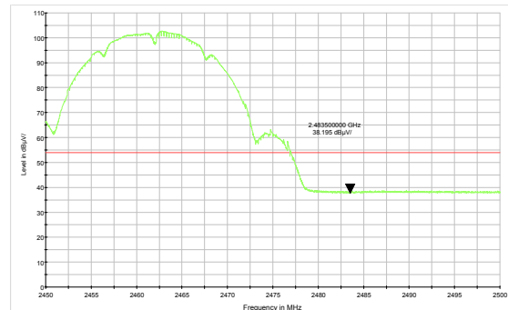
802.11b-Channel 11 Average
