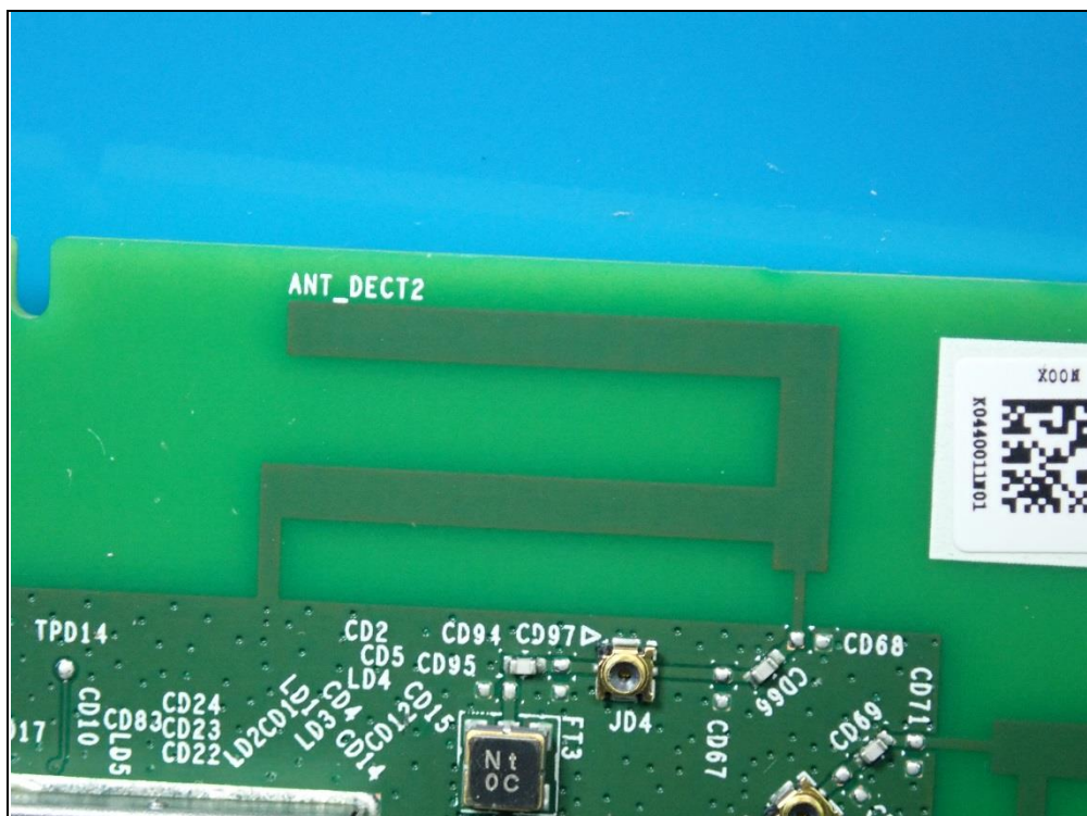
Antenna - DECT 2
