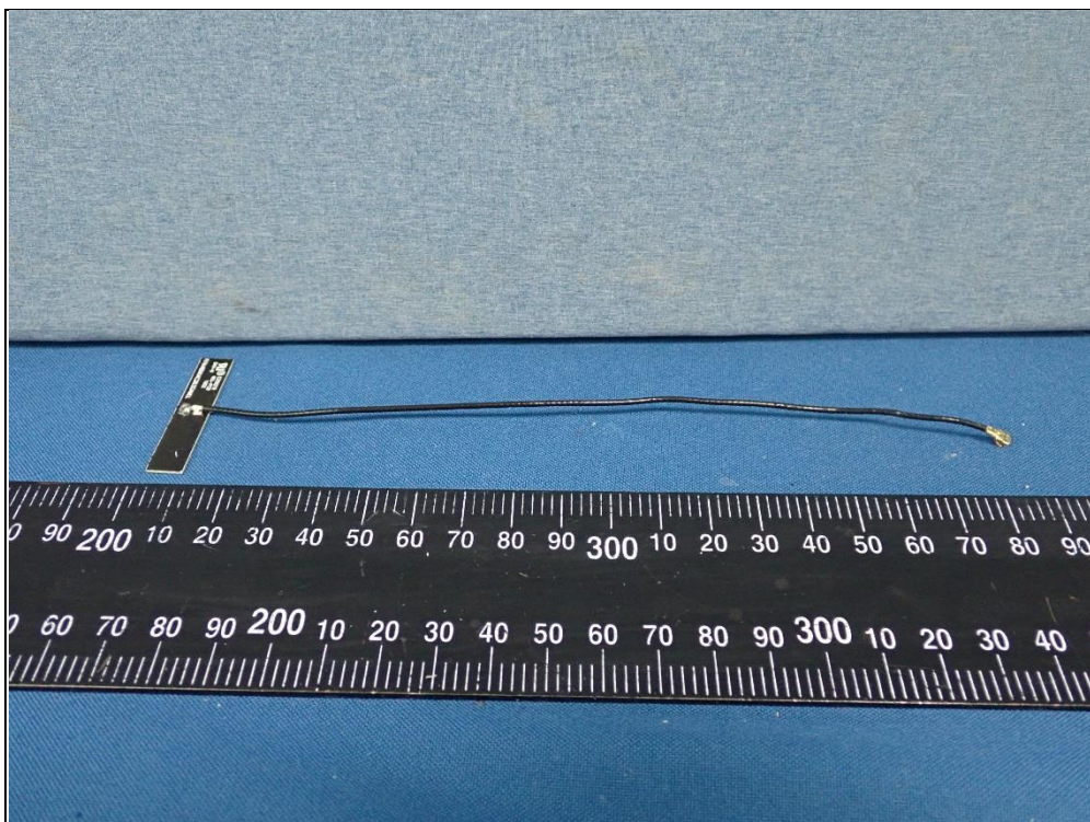
Antenna – WiFi 2.4G Chain 1
