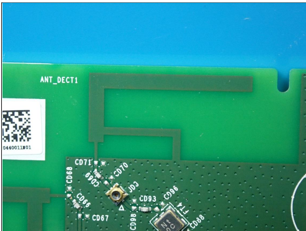
Antenna - DECT 1
