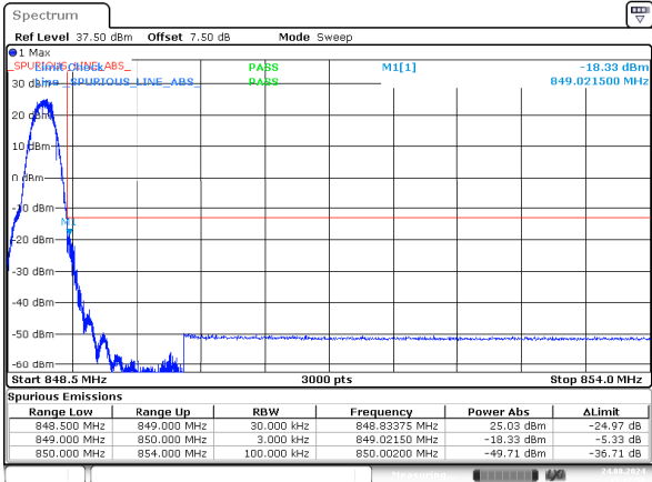
GSM_High -18.33dBm
