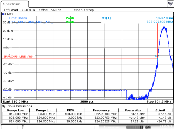
GSM_Low -14.47dBm
