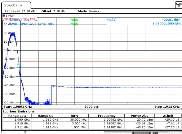
GSM_High -20.61dBm
