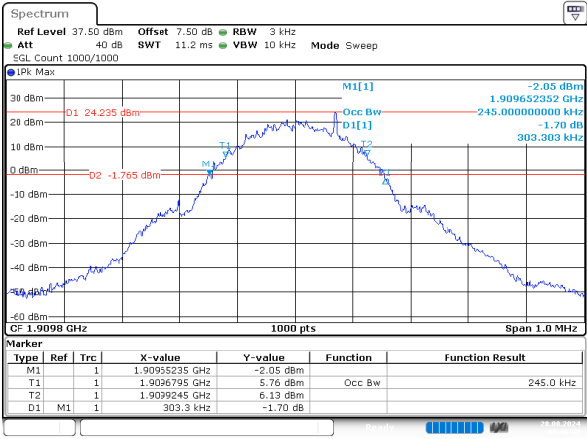
GSM_High 0.245MHz
