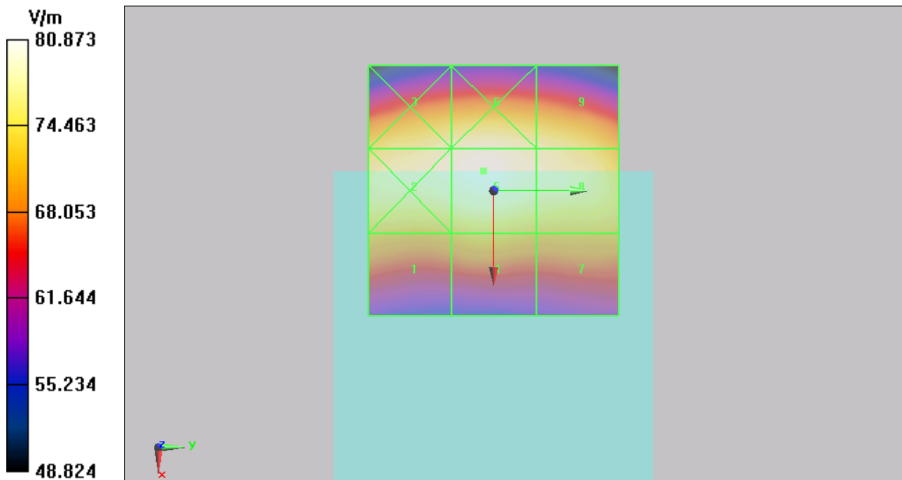
Figure 14 HAC RF E-Field GSM 1900 Channel 810
