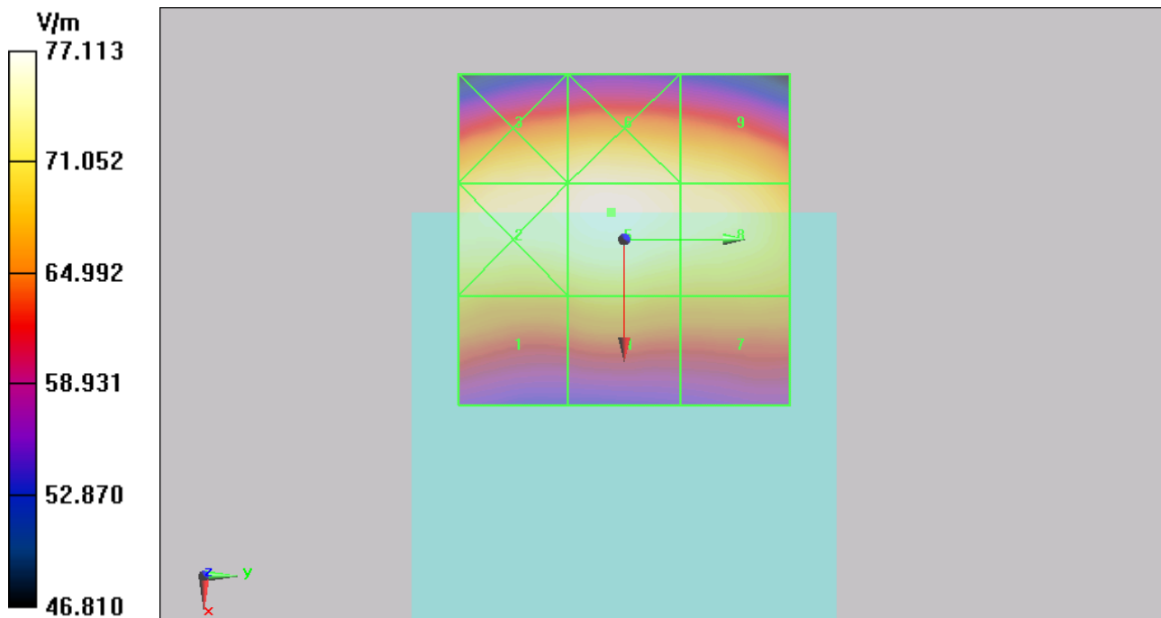
Figure 10 HAC RF E-Field GSM 850 Channel 128
