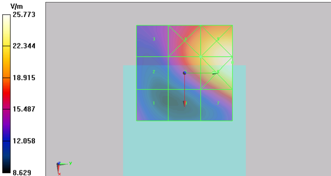
Figure 18 HAC RF E-Field GSM 1900 Channel 661
