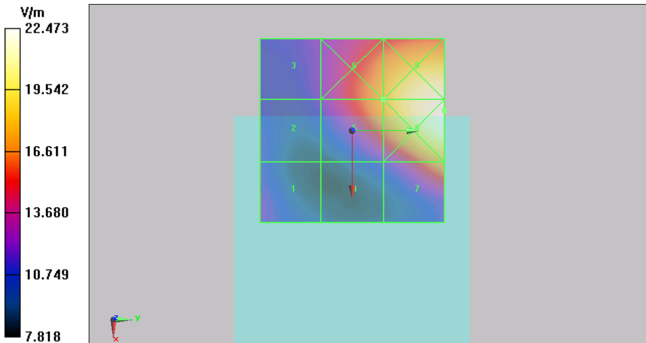
Figure 17 HAC RF E-Field GSM 1900 Channel 810
