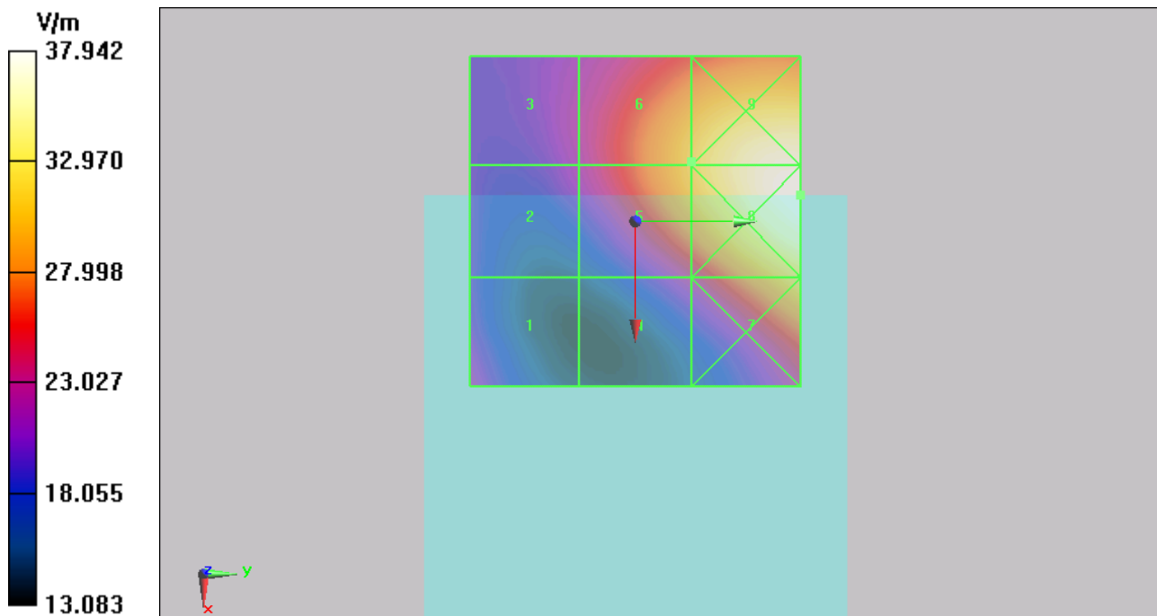
Figure 16 HAC RF E-Field GSM 1900 Channel 512
