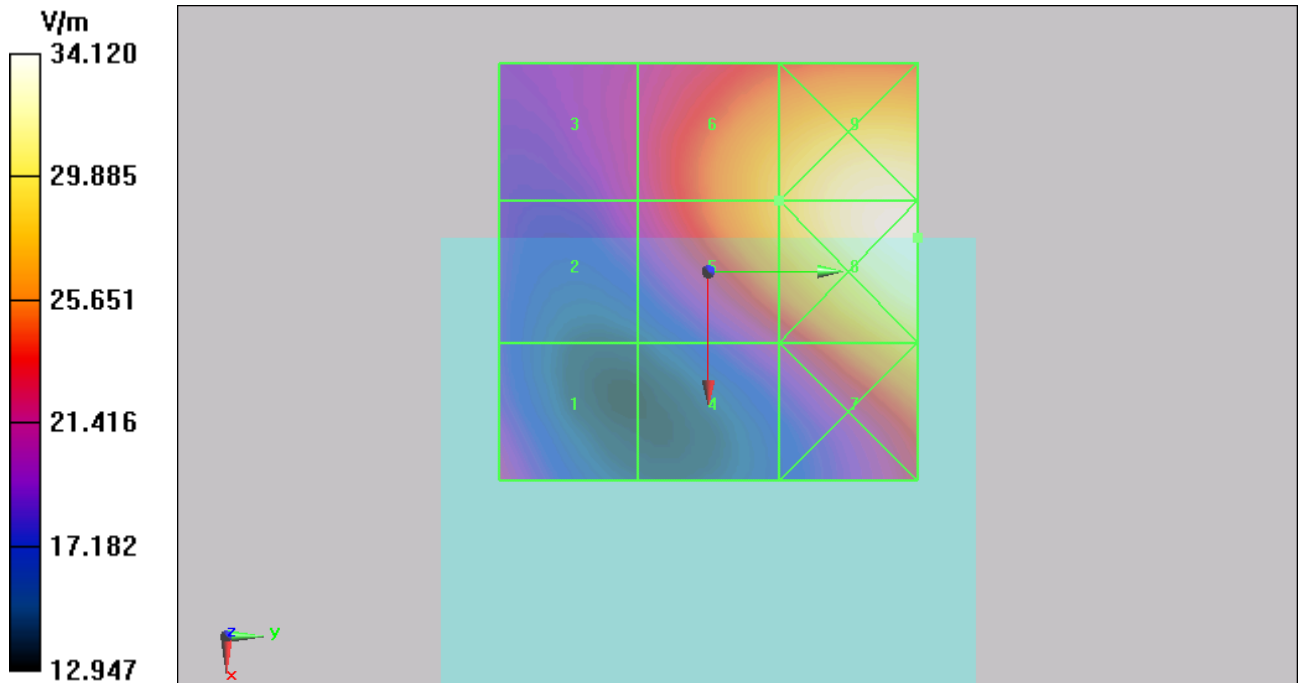
Figure 15 HAC RF E-Field GSM 1900 Channel 661
