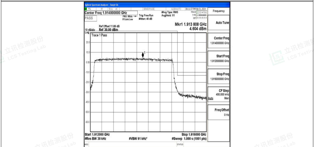
Band25_3MHz_16QAM_26675_15RB#0
