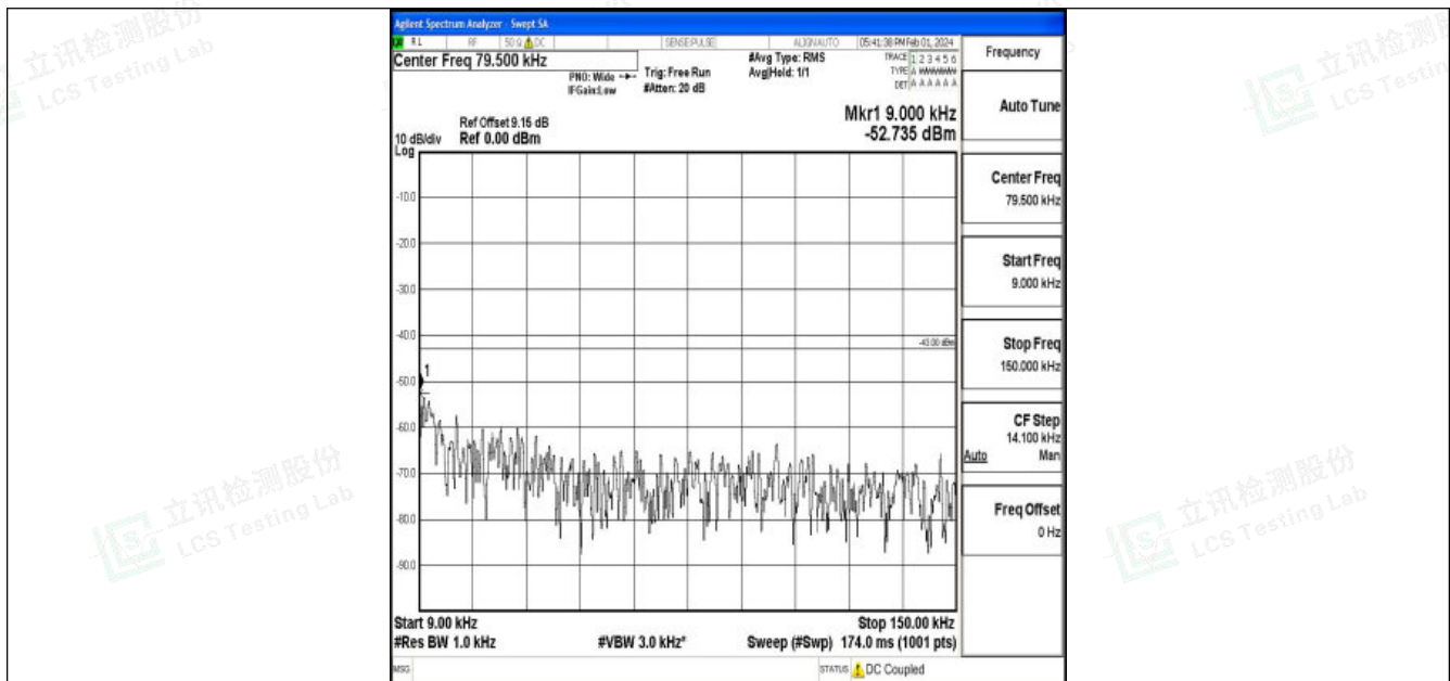
Band25_1.4MHz_QPSK_26365_1RB#0_0.009~0.15_0.009~0.15
