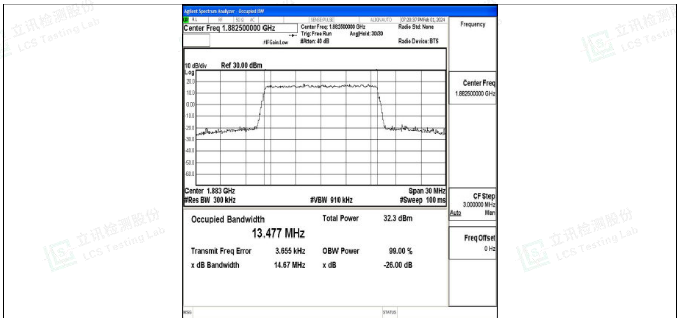
Band25-15MHz-QPSK-26365-75RB#0-PASS
