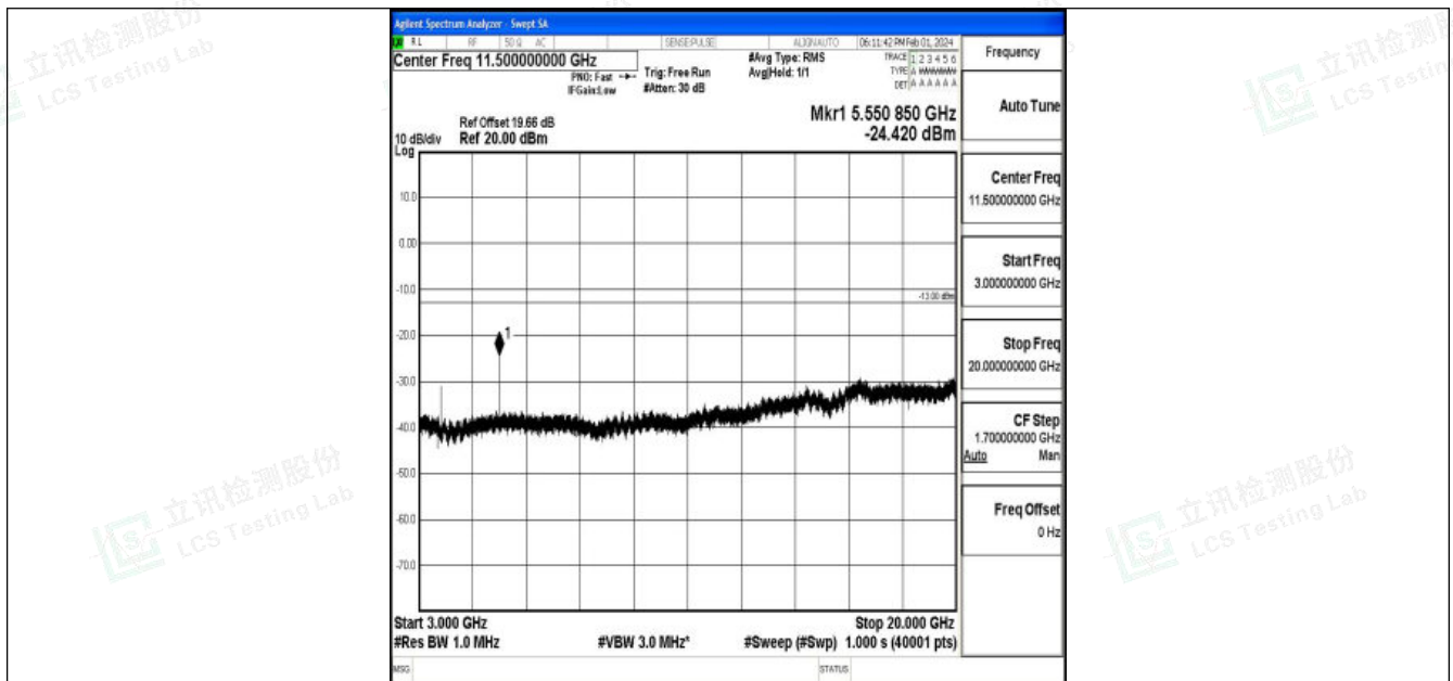
Band25_3MHz_QPSK_26055_1RB#0_3000~20000_3000~20000
