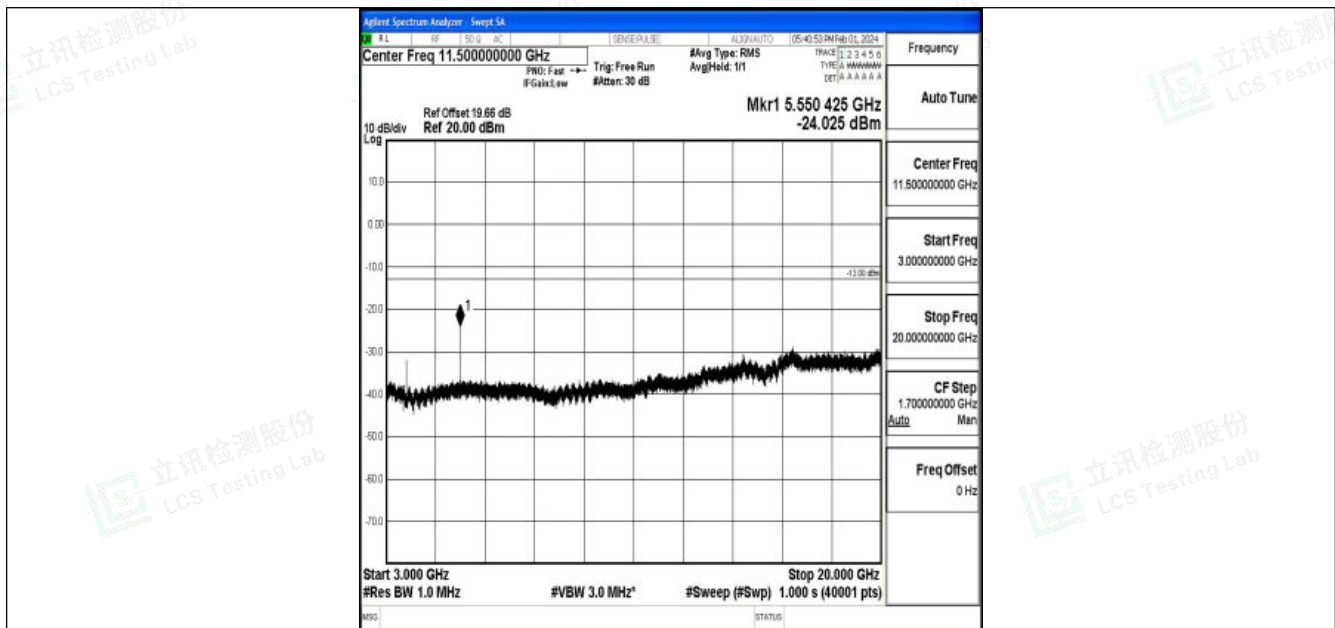
Band25_1.4MHz_QPSK_26047_1RB#0_3000~20000_3000~20000
