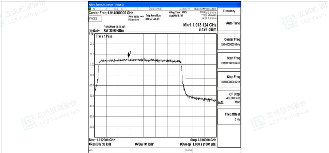
Band25_3MHz_QPSK_26675_15RB#0
