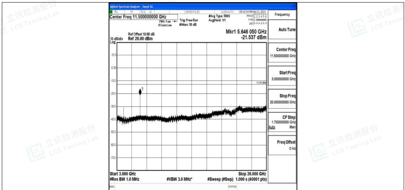
Band25_1.4MHz_QPSK_26365_1RB#0_3000~20000_3000~20000
