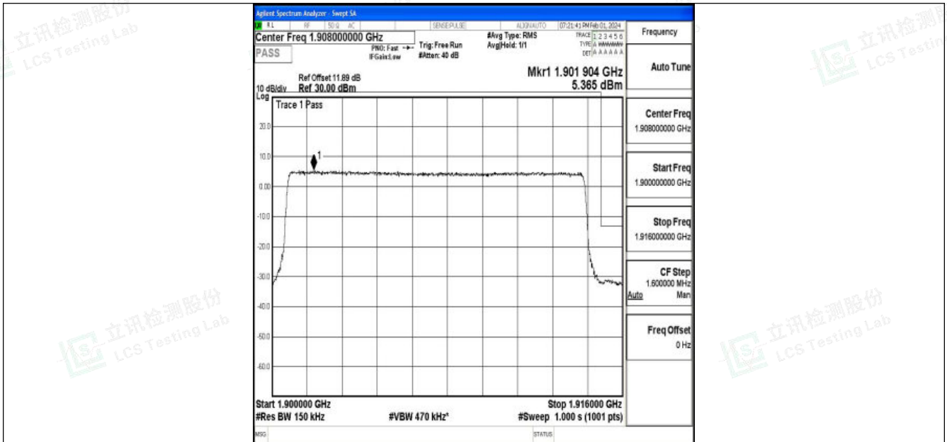
Band25_15MHz_QPSK_26615_75RB#0
