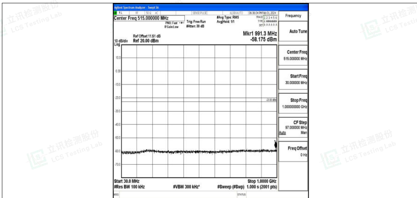
Band25_5MHz_QPSK_26065_1RB#0_30~1000_30~1000
