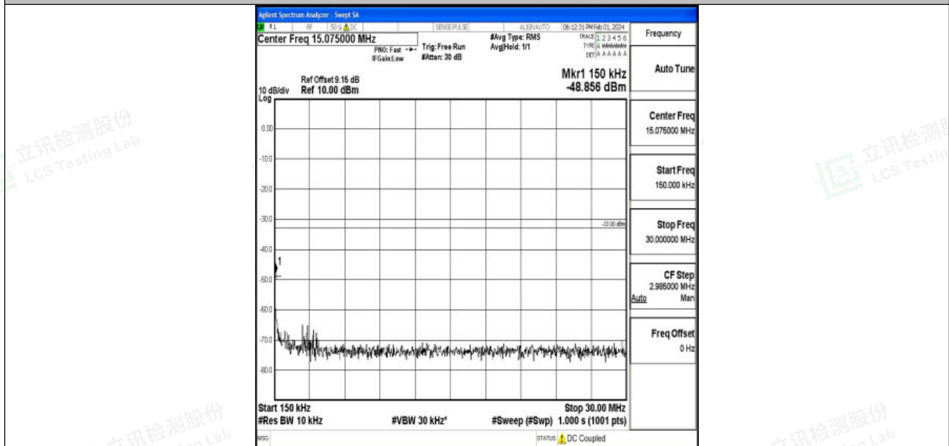
Band25_3MHz_QPSK_26365_1RB#0_0.15~30_0.15~30
