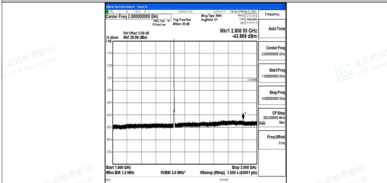
Band25_5MHz_QPSK_26065_1RB#0_1000~3000_1000~3000
