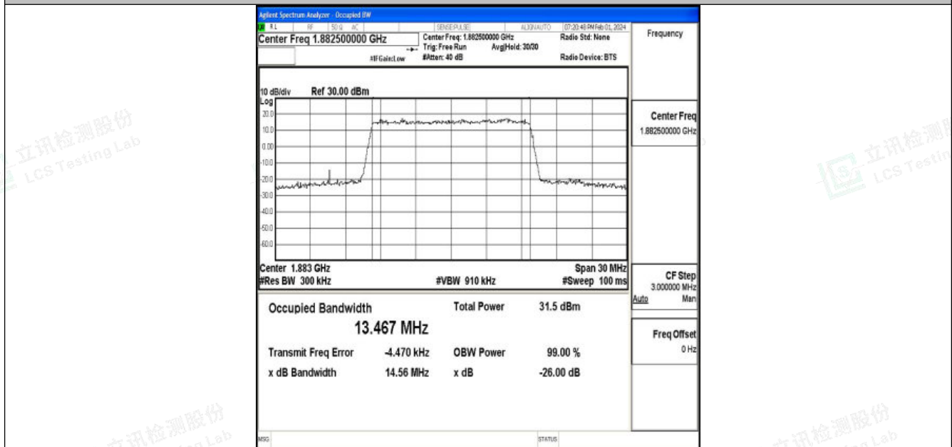
Band25-15MHz-16QAM-26365-75RB#0-PASS
