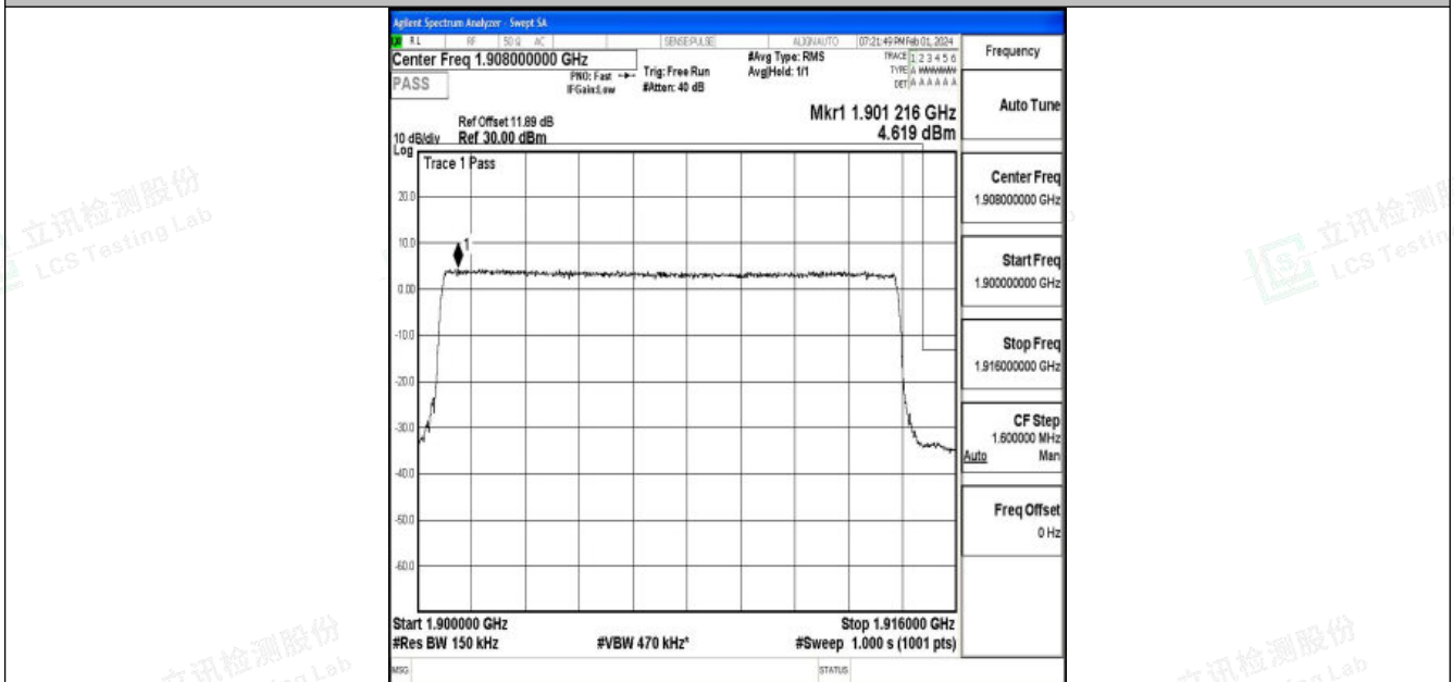
Band25_15MHz_16QAM_26615_75RB#0
