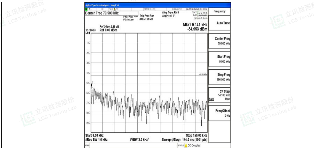
Band25_5MHz_QPSK_26365_1RB#0_0.009~0.15_0.009~0.15
