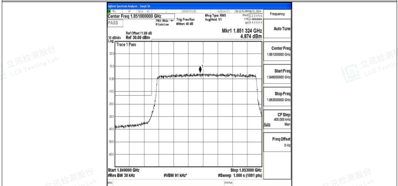
Band25_3MHz_16QAM_26055_15RB#0
