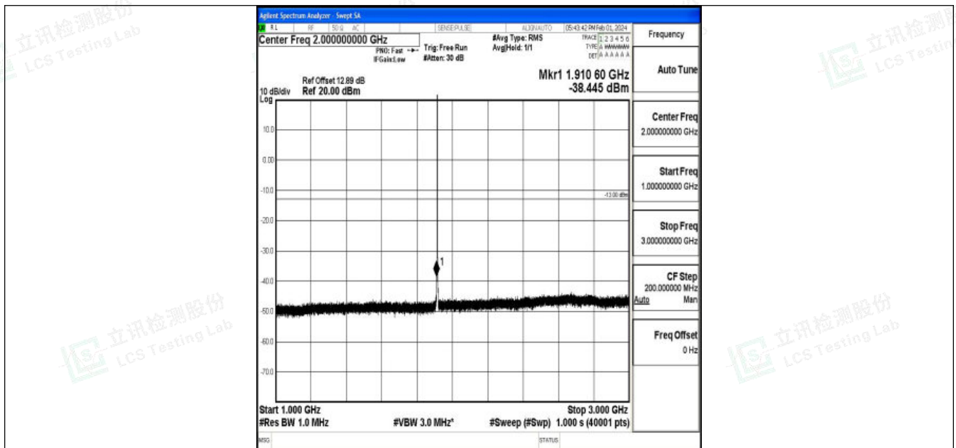
Band25_1.4MHz_16QAM_26683_1RB#0_1000~3000_1000~3000
