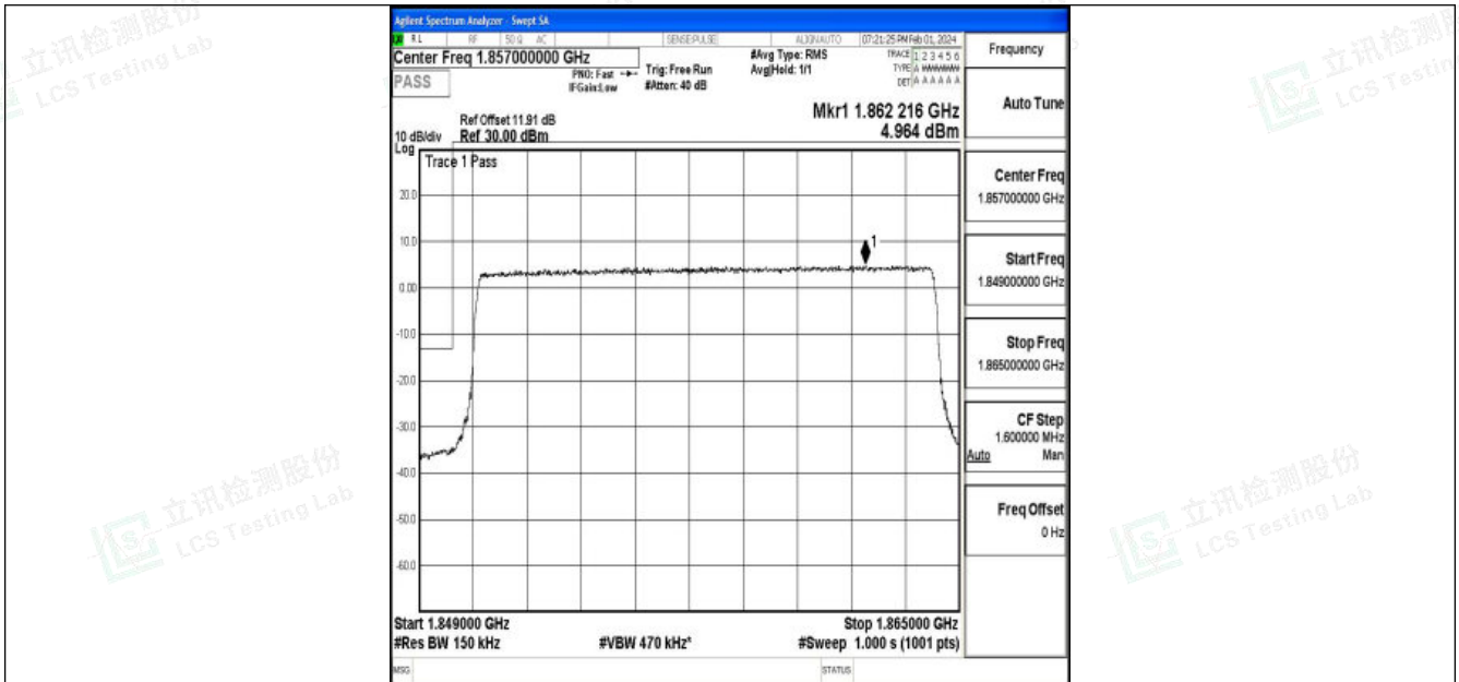
Band25_15MHz_QPSK_26115_75RB#0
