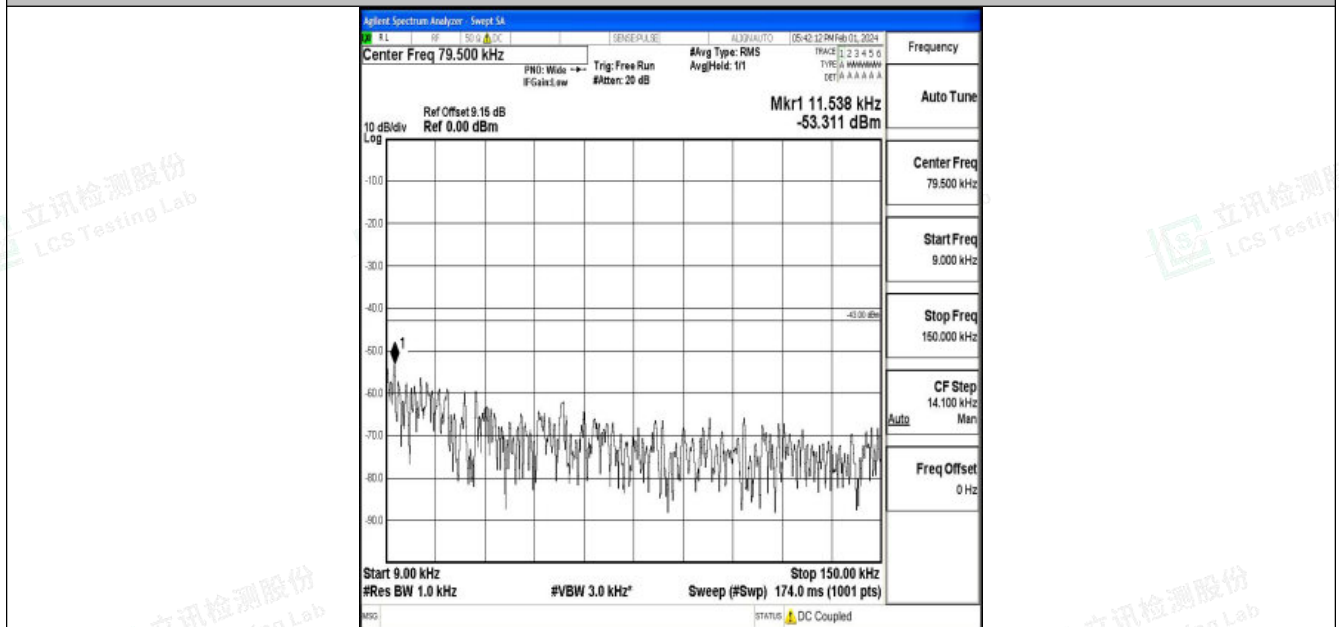
Band25_1.4MHz_16QAM_26365_1RB#0_0.009~0.15_0.009~0.15
