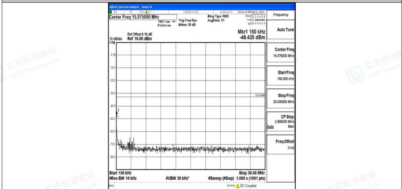
Band25_1.4MHz_QPSK_26365_1RB#0_0.15~30_0.15~30
