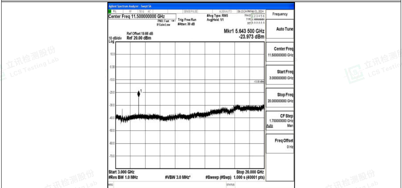
Band25_3MHz_16QAM_26365_1RB#0_3000~20000_3000~20000
