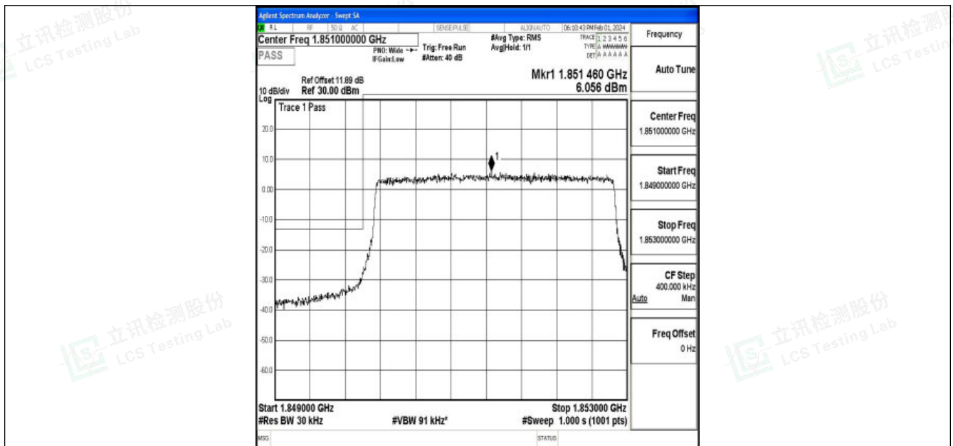
Band25_3MHz_QPSK_26055_15RB#0
