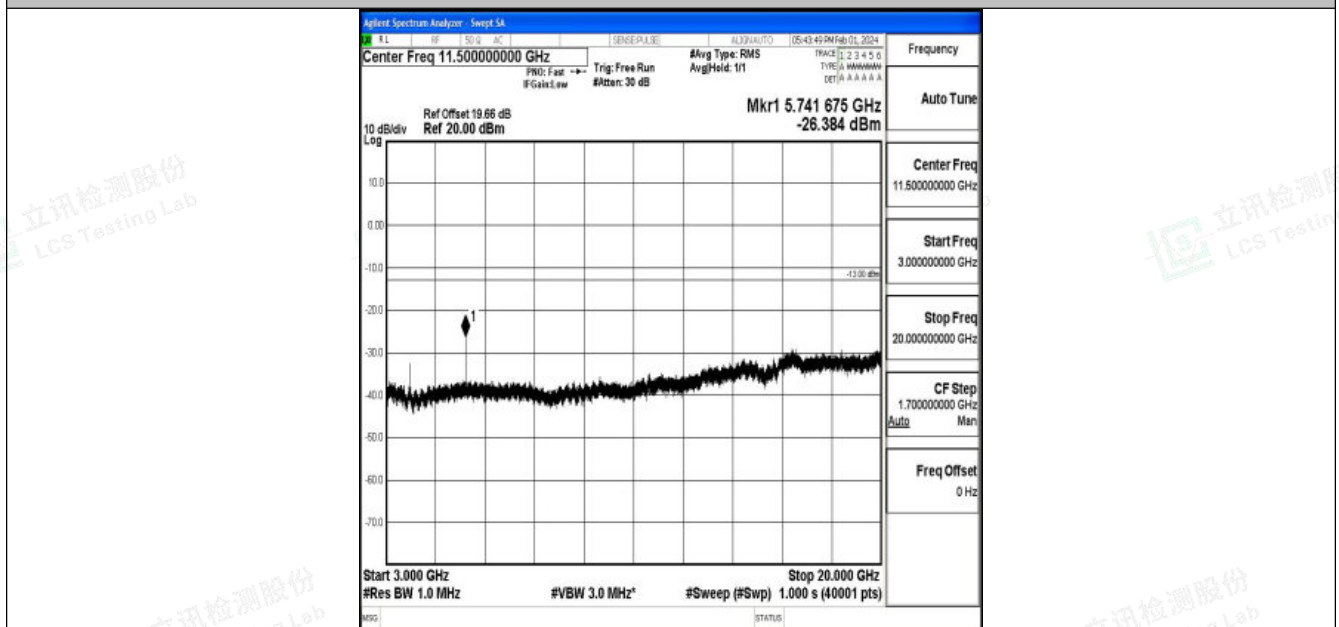
Band25_1.4MHz_16QAM_26683_1RB#0_3000~20000_3000~20000
