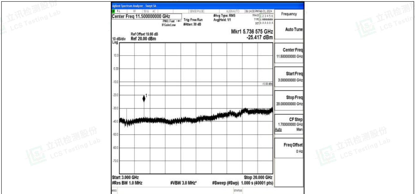
Band25_3MHz_QPSK_26675_1RB#0_3000~20000_3000~20000
