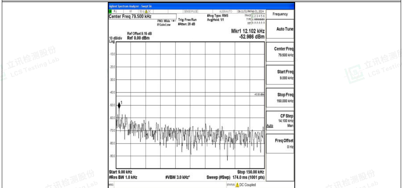
Band25_3MHz_16QAM_26055_1RB#0_0.009~0.15_0.009~0.15
