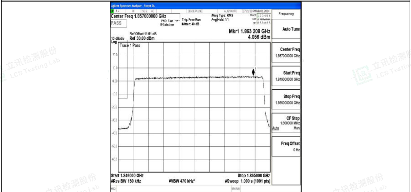
Band25_15MHz_16QAM_26115_75RB#0
