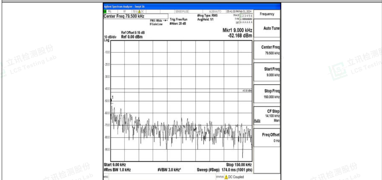
Band25_1.4MHz_16QAM_26047_1RB#0_0.009~0.15_0.009~0.15
