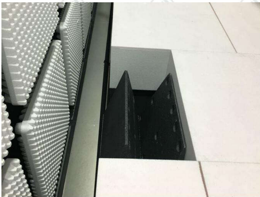
Radiated spurious emission Test Setup-4(Above 1GHz) There are absorbing materials under the ground.
