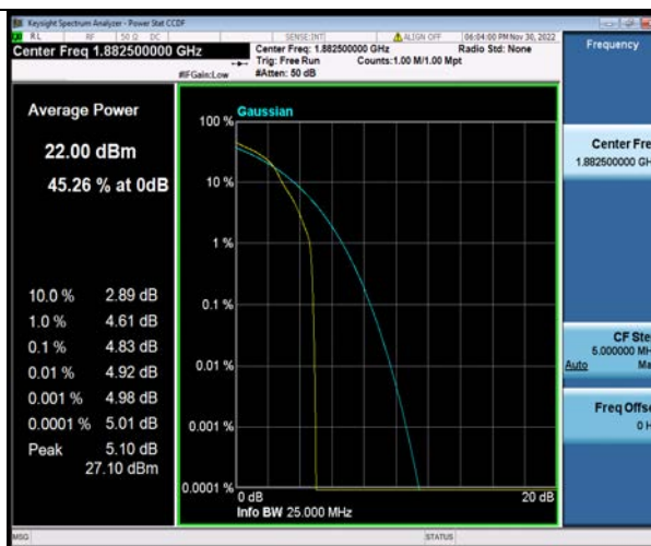
Band25-15MHz-16QAM-26365-75RB#0
