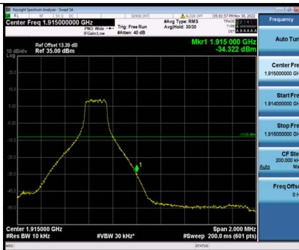
Band25-5MHz-64QAM-26665-25RB#0
