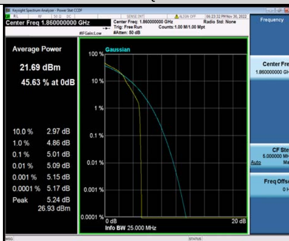
Band25-20MHz-16QAM-26140-100RB#0
