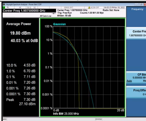
Band25-15MHz-16QAM-26615-75RB#0
