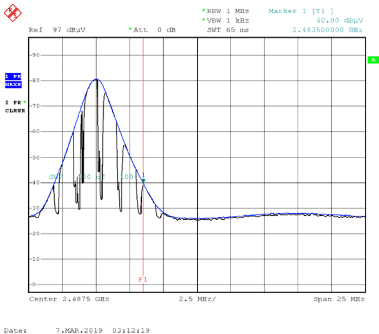
Radiated Restricted Band Edges plot – Average Reading (GFSK, Ch.78)
