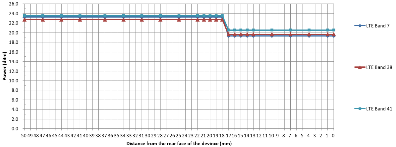
Right Sensor Near/Far Detection threshold (moving toward phantom)
