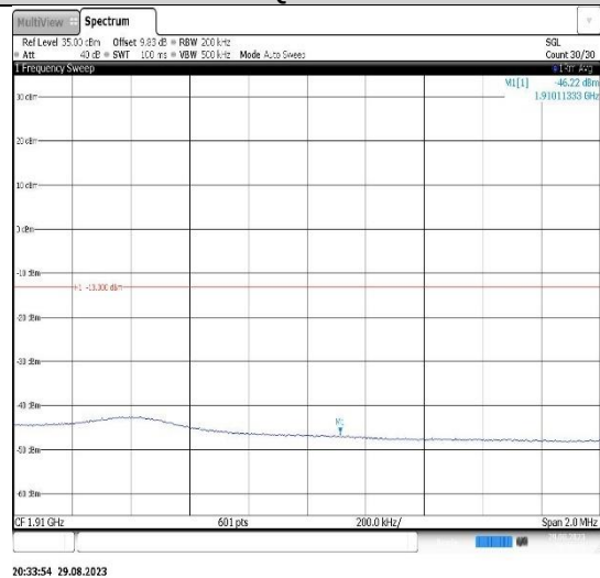
Band2-10MHz-QPSK-19150-50RB#0
