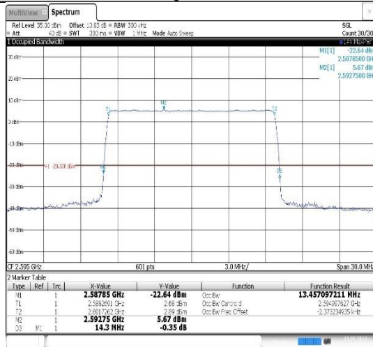
Band38-15MHz-QPSK-38000-75RB#0
