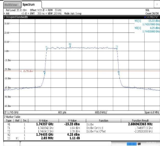
Band66-3MHz-16QAM-132322-15RB#0
