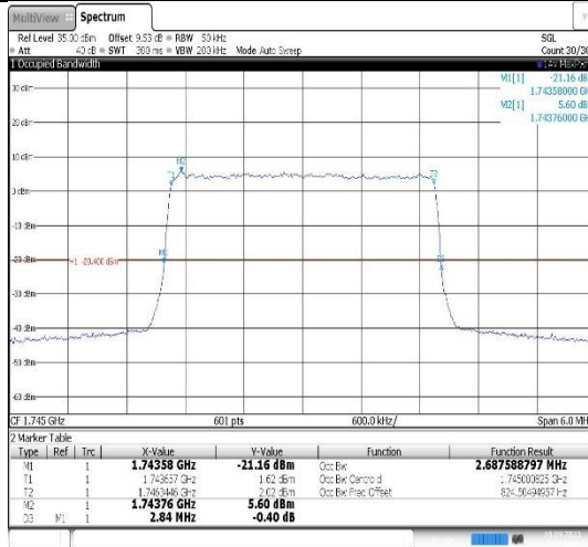
Band66-3MHz-QPSK-132322-15RB#0
