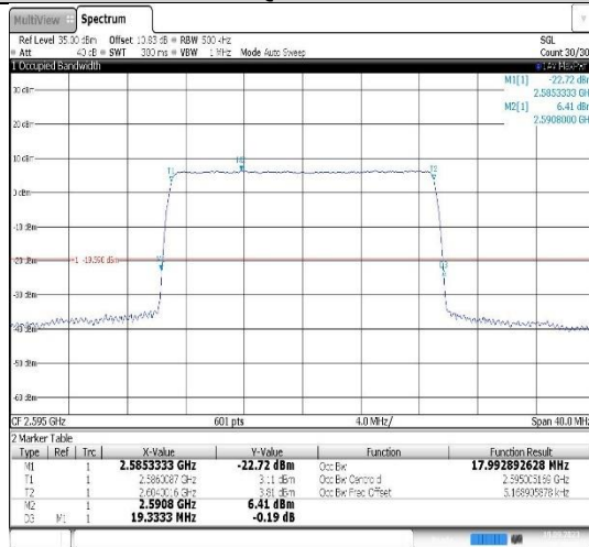
Band38-20MHz-QPSK-38000-100RB#0
