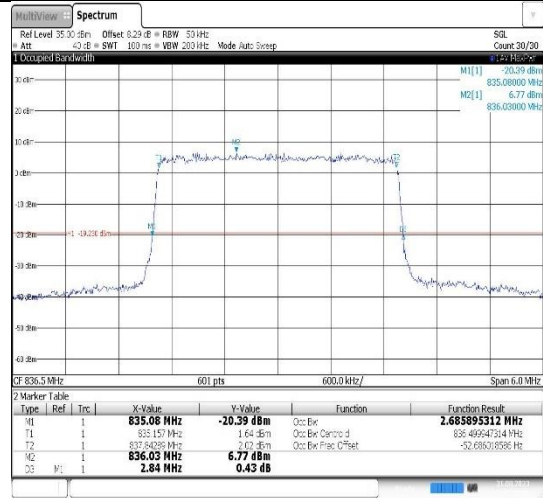
Band26(824-849)-3MHz-16QAM-26915-15RB#0
