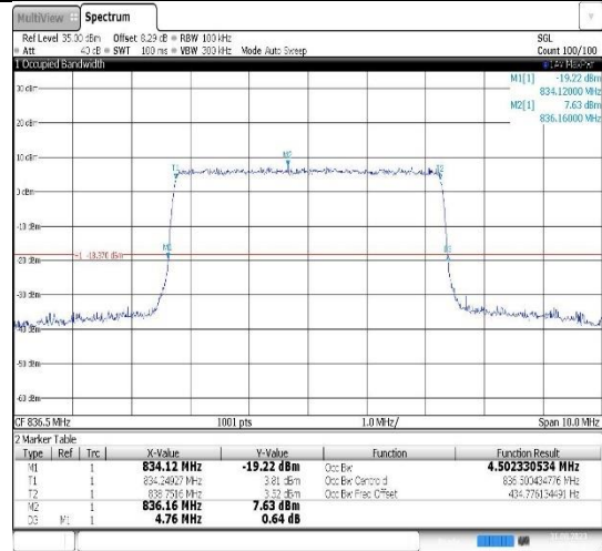
Band26(824-849)-5MHz-16QAM-26915-25RB#0
