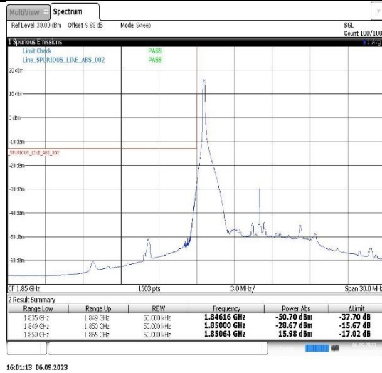
Band2-10MHz-16QAM-18650-50RB#0
