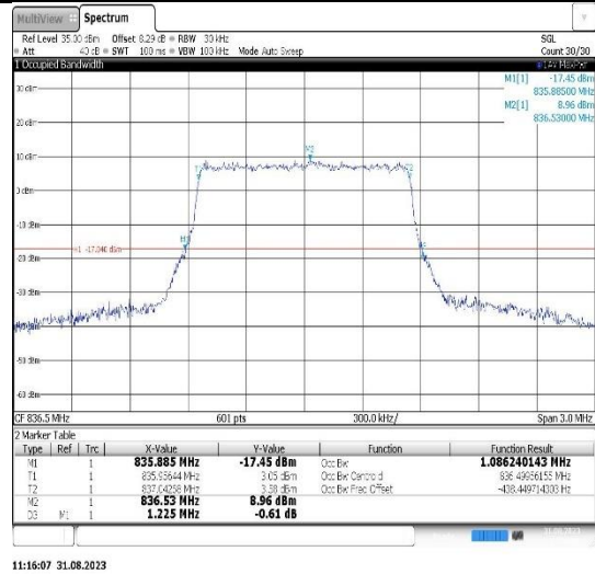
Band26(824-849)-3MHz-16QAM-26915-15RB#0
