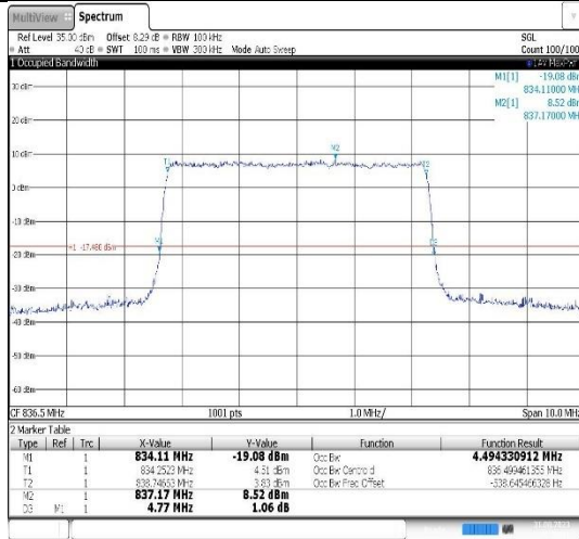
Band26(824-849)-5MHz-QPSK-26915-25RB#0
