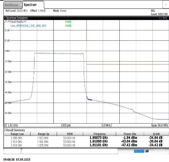
Band2-15MHz-QPSK-18675-75RB#0
