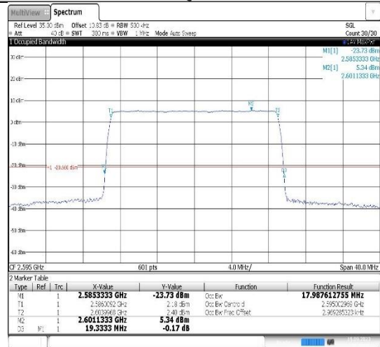
Band38-20MHz-16QAM-38000-100RB#0
