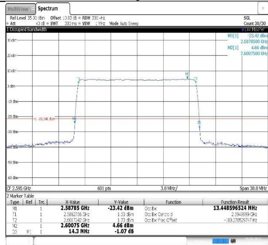
Band38-15MHz-16QAM-38000-75RB#0
