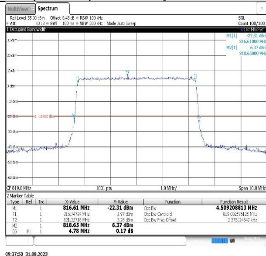
Band26(814-824)-10MHz-16QAM-26740-50RB#0
