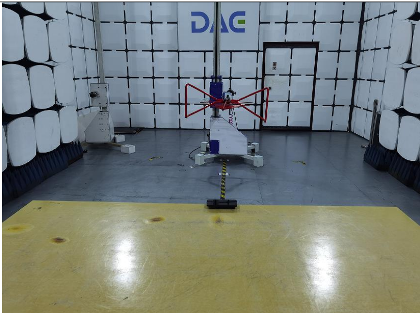
Emissions in frequency bands (30MHz - 1GHz) -TM4
