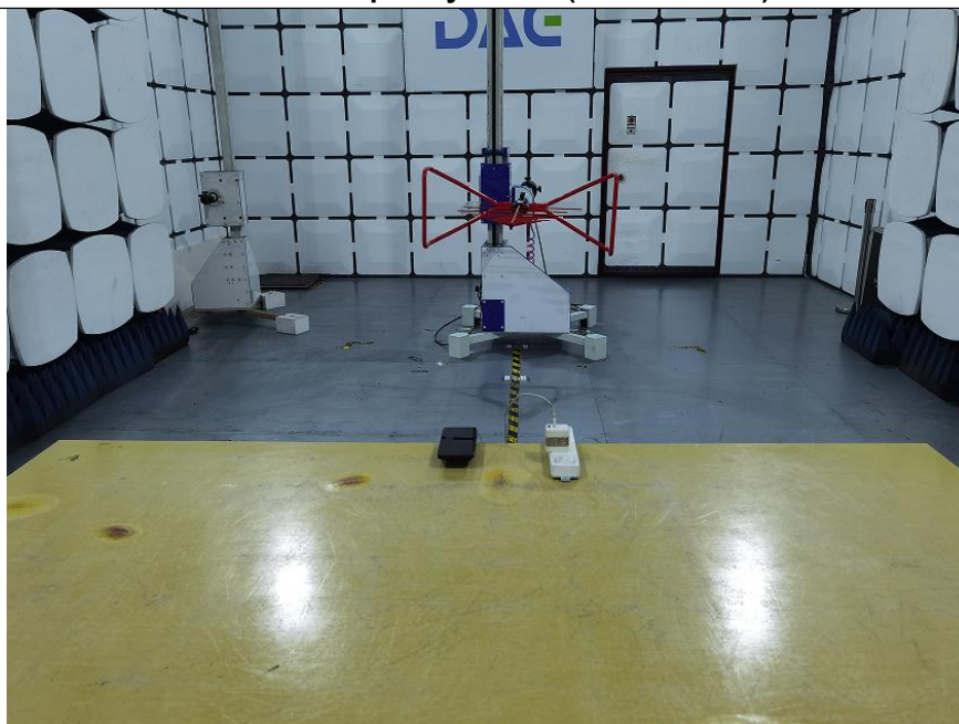
Emissions in frequency bands (below 30MHz) -TM1
