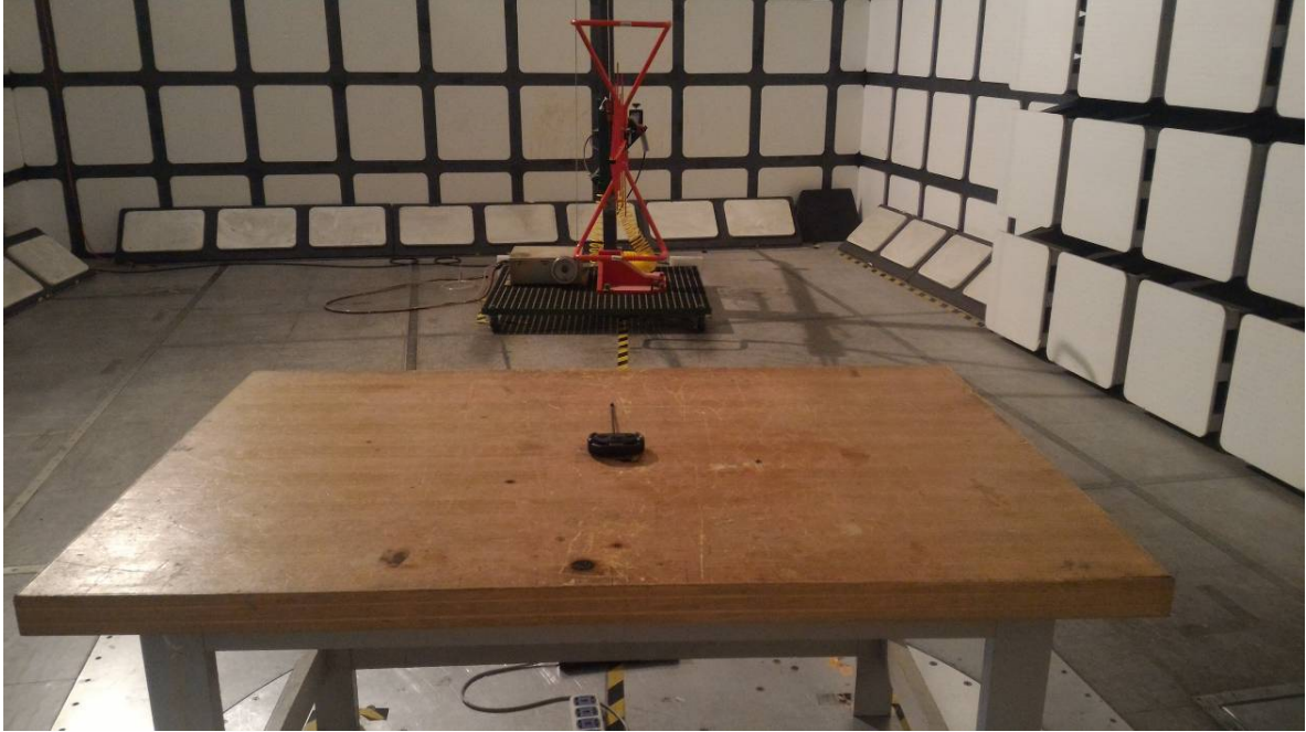
Radiated Emissions View (30 MHz~1 GHz)
