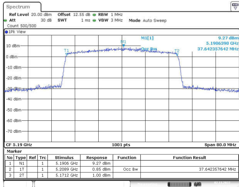
Fig. 47 99% Occupied Bandwidth (802.11ax-HE40, 5190MHz)
