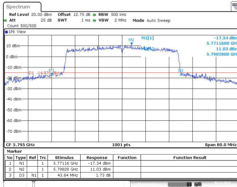
Fig. 21 Occupied 26dB Bandwidth (802.11ax-HE40, 5795MHz)
