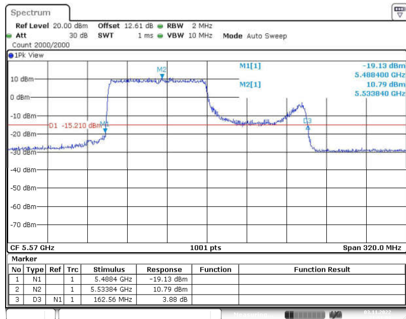
Fig. 28 Occupied 26dB Bandwidth (802.11ax-HE160, 5570MHz)
