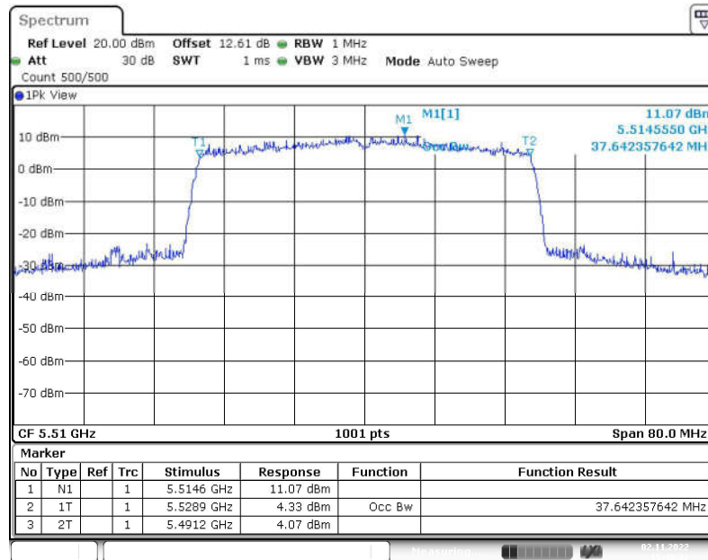
Fig. 51 99% Occupied Bandwidth (802.11ax-HE40, 5510MHz)
