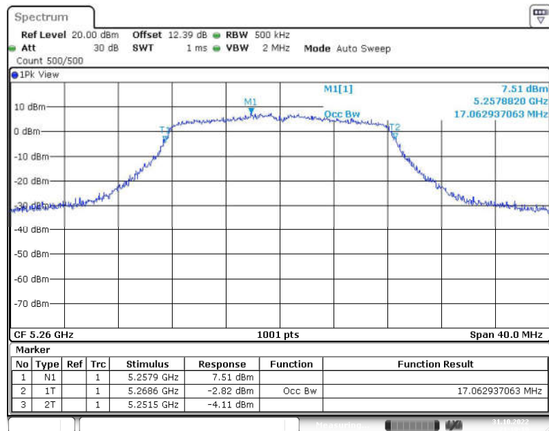
Fig. 38 99% Occupied Bandwidth (802.11a, 5260MHz)
