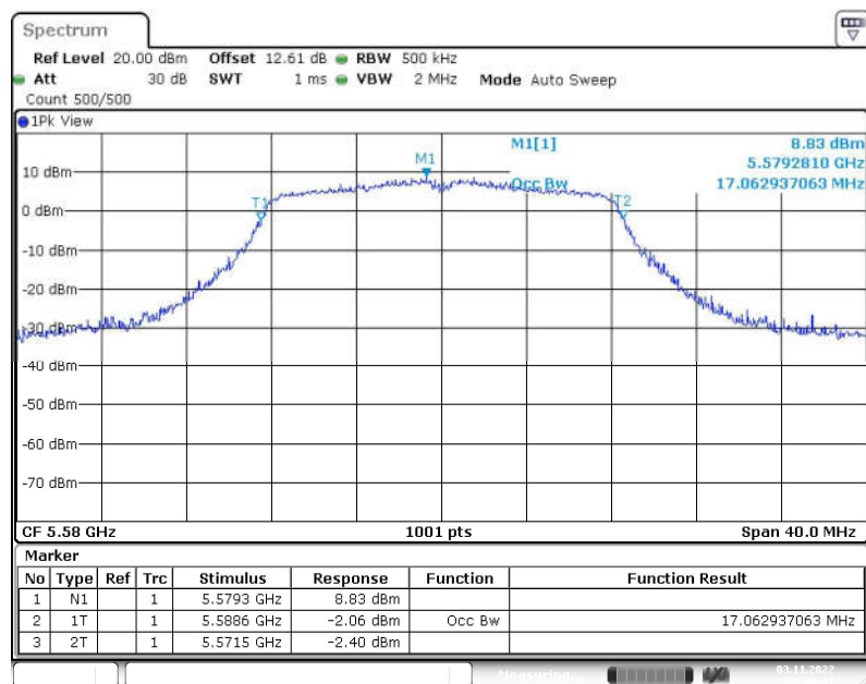
Fig. 42 99% Occupied Bandwidth (802.11a, 5580MHz)
