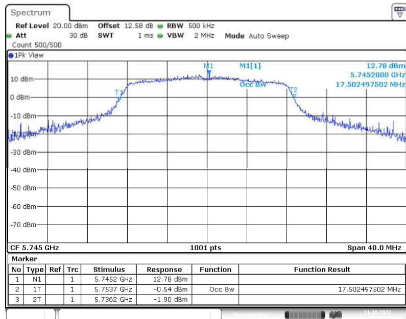
Fig. 44 99% Occupied Bandwidth (802.11a, 5745MHz)
