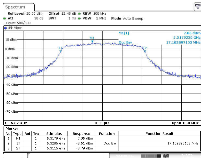
Fig. 40 99% Occupied Bandwidth (802.11a, 5320MHz)
