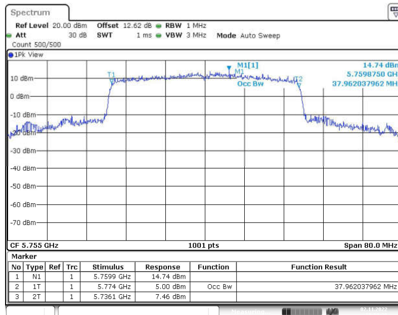
Fig. 54 99% Occupied Bandwidth (802.11ax-HE40, 5755MHz)
