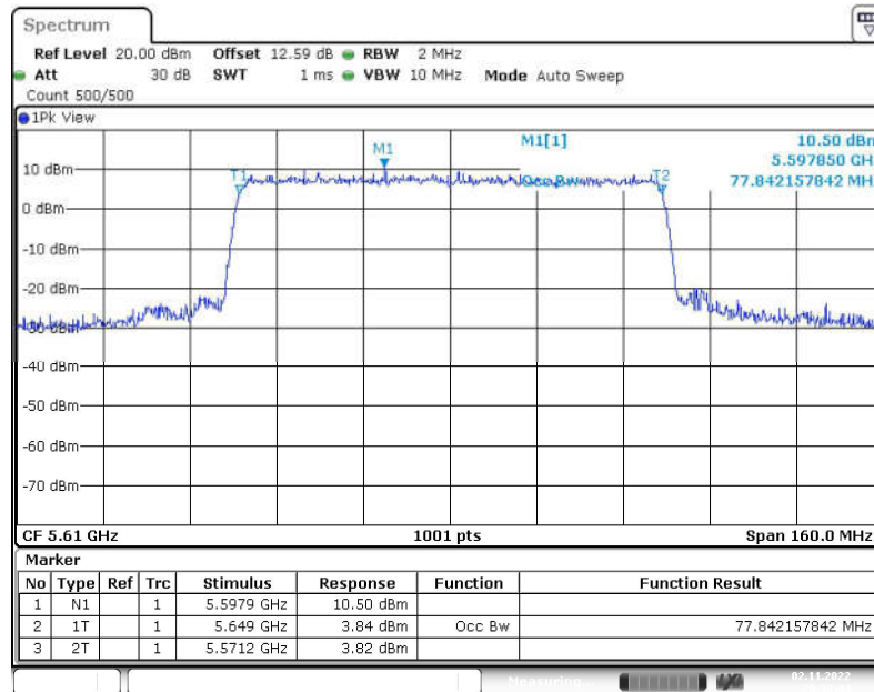
Fig. 59 99% Occupied Bandwidth (802.11ax-HE80, 5610MHz)
