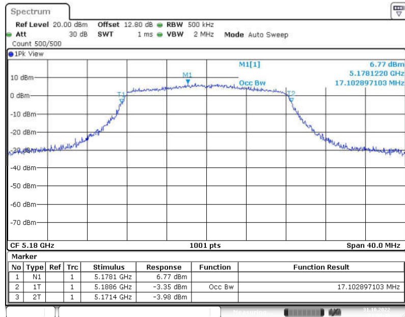
Fig. 35 99% Occupied Bandwidth (802.11a, 5180MHz)
