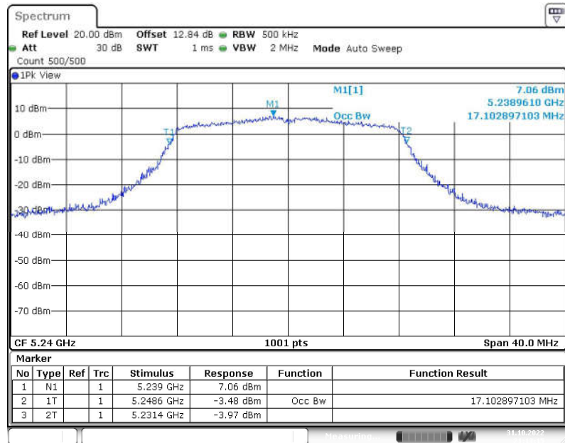
Fig. 37 99% Occupied Bandwidth (802.11a, 5240MHz)
