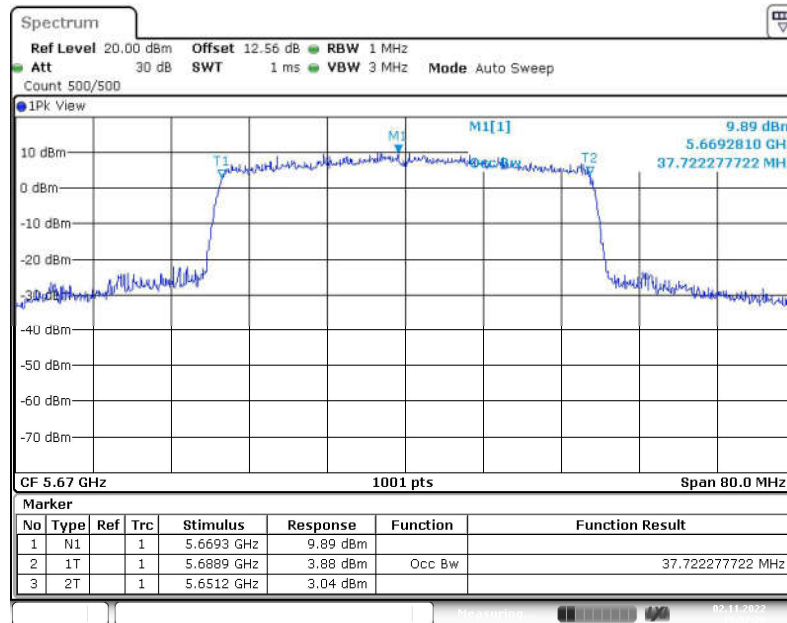
Fig. 53 99% Occupied Bandwidth (802.11ax-HE40, 5670MHz)
