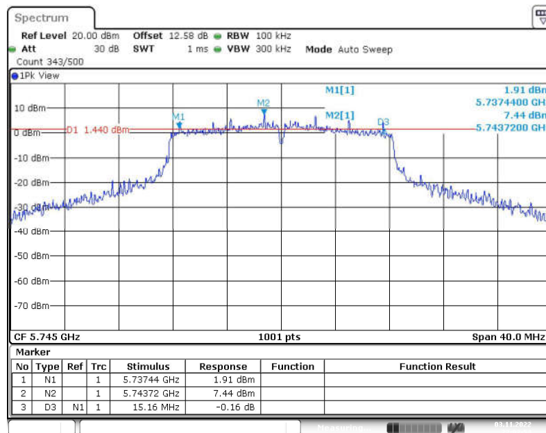
Fig. 29 Occupied 6dB Bandwidth (802.11a, 5745MHz)
