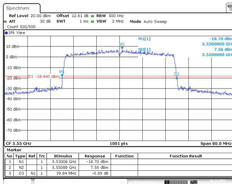
Fig. 18 Occupied 26dB Bandwidth (802.11ax-HE40, 5550MHz)
