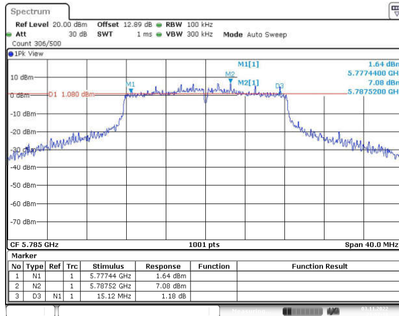
Fig. 30 Occupied 6dB Bandwidth (802.11a, 5785MHz)
