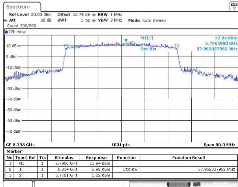
Fig. 55 99% Occupied Bandwidth (802.11ax-HE40, 5795MHz)
