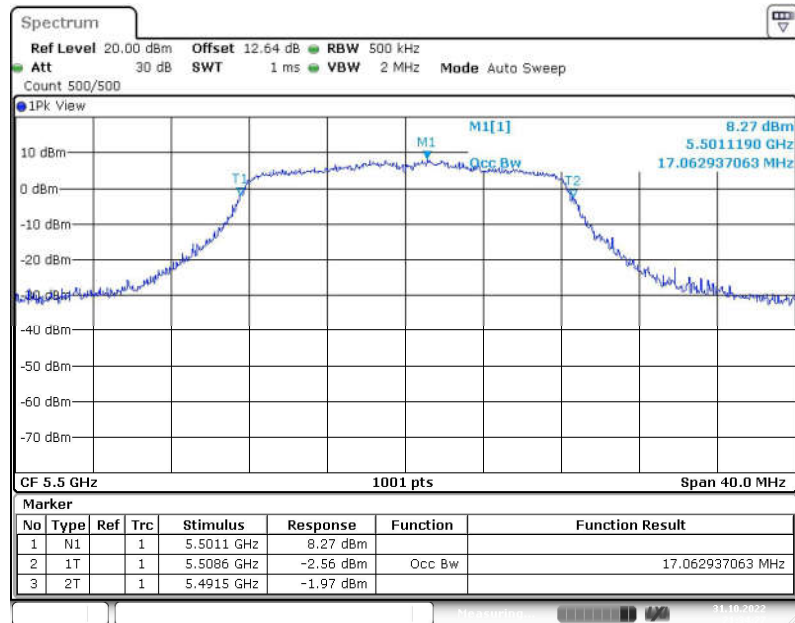
Fig. 41 99% Occupied Bandwidth (802.11a, 5500MHz)
