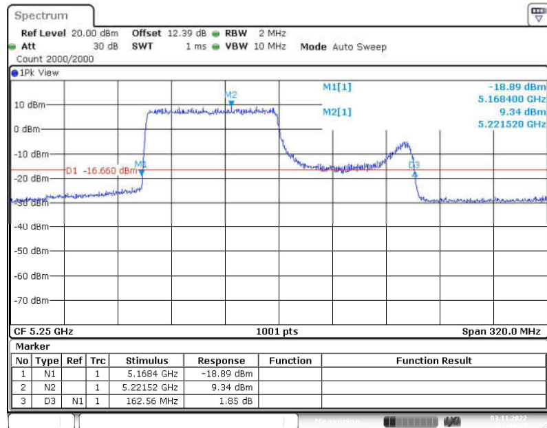
Fig. 27 Occupied 26dB Bandwidth (802.11ax-HE160, 5250MHz)
