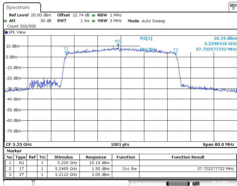
Fig. 48 99% Occupied Bandwidth (802.11ax-HE40, 5230MHz)
