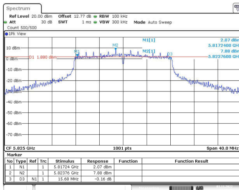
Fig. 31 Occupied 6dB Bandwidth (802.11a, 5825MHz)
