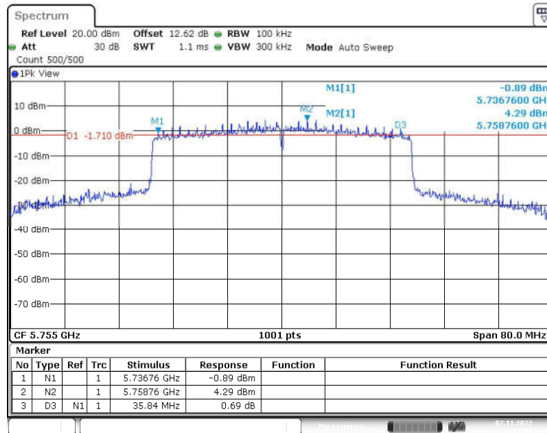
Fig. 32 Occupied 6dB Bandwidth (802.11ax-HE40, 5755MHz)
