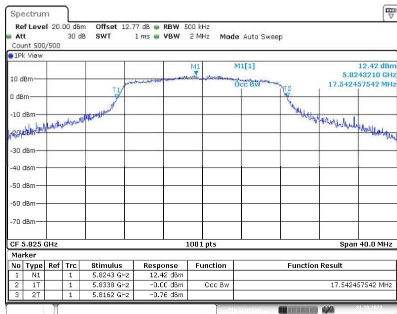
Fig. 46 99% Occupied Bandwidth (802.11a, 5825MHz)
