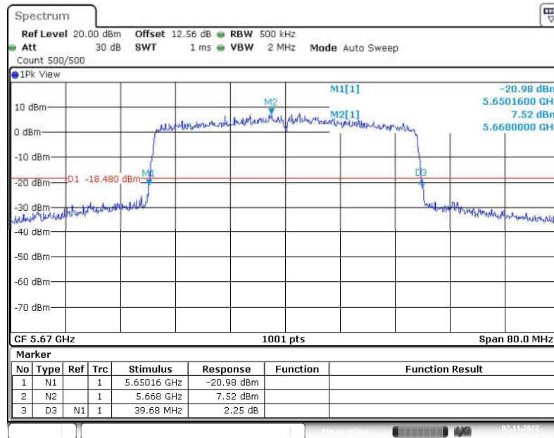
Fig. 19 Occupied 26dB Bandwidth (802.11ax-HE40, 5670MHz)
