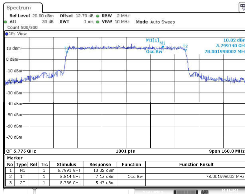
Fig. 60 99% Occupied Bandwidth (802.11ax-HE80, 5775MHz)
