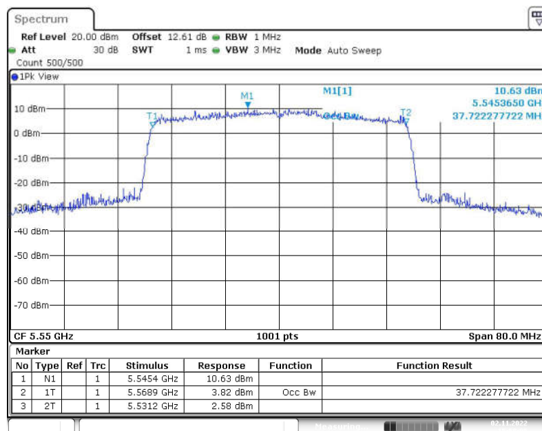
Fig. 52 99% Occupied Bandwidth (802.11ax-HE40, 5550MHz)
