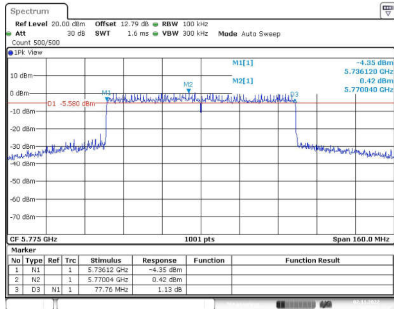
Fig. 34 Occupied 6dB Bandwidth (802.11ax-HE80, 5775MHz)
