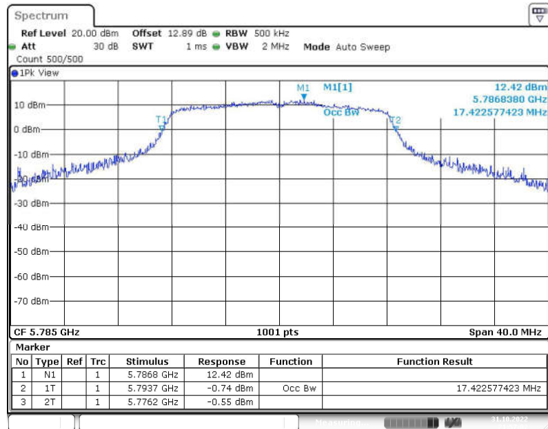
Fig. 45 99% Occupied Bandwidth (802.11a, 5785MHz)
