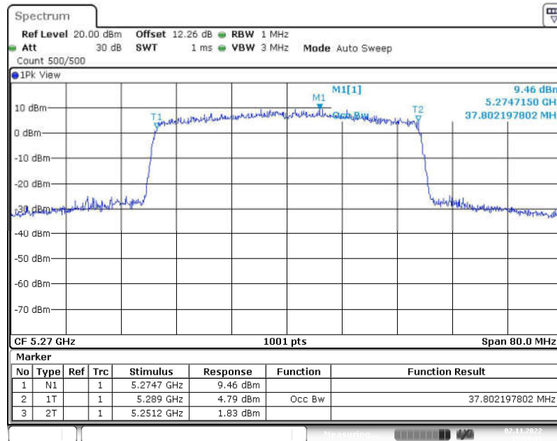
Fig. 49 99% Occupied Bandwidth (802.11ax-HE40, 5270MHz)
