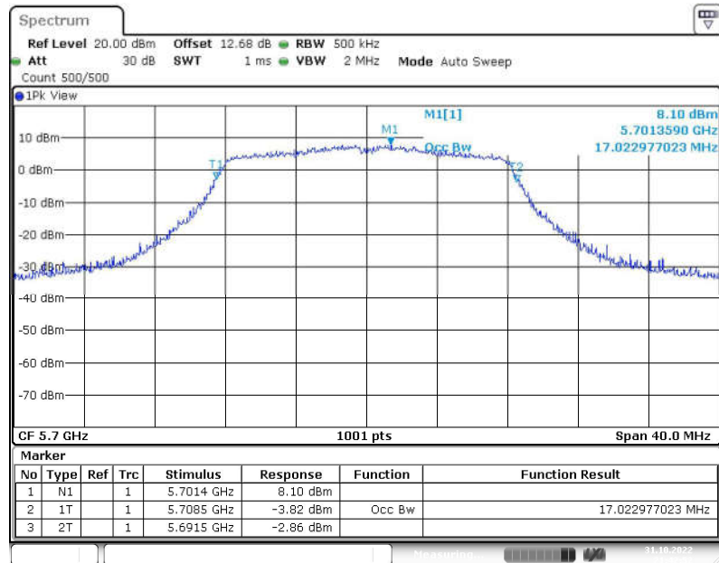
Fig. 43 99% Occupied Bandwidth (802.11a, 5700MHz)
