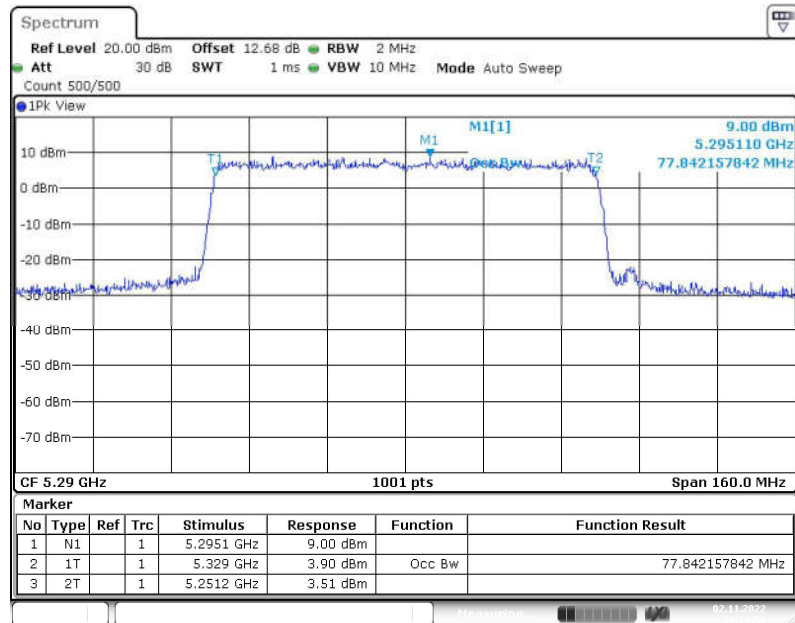
Fig. 57 99% Occupied Bandwidth (802.11ax-HE80, 5290MHz)
