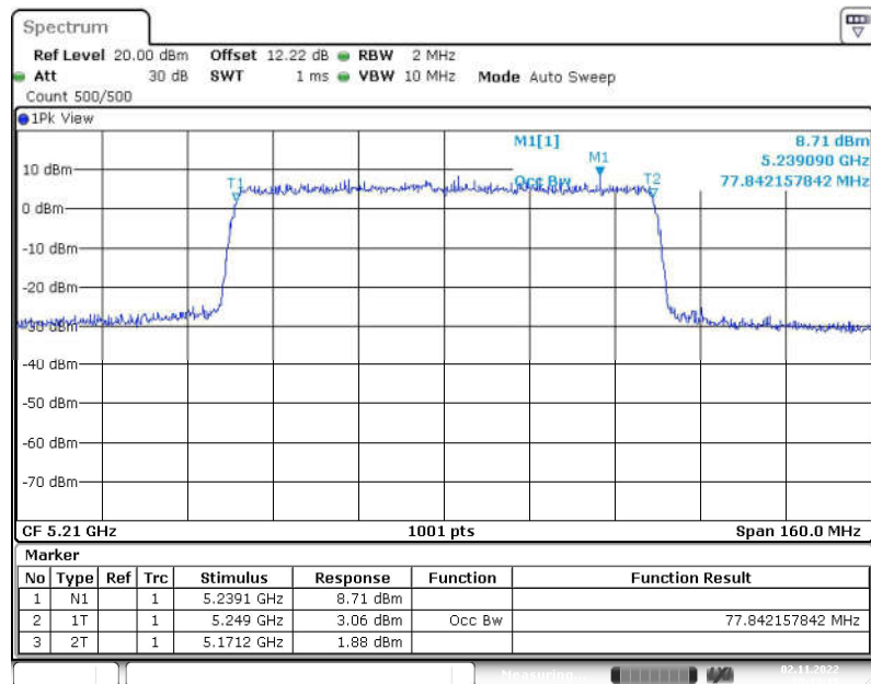
Fig. 56 99% Occupied Bandwidth (802.11ax-HE80, 5210MHz)
