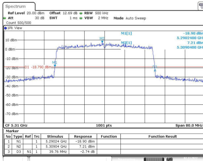
Fig. 16 Occupied 26dB Bandwidth (802.11ax-HE40, 5310MHz)
