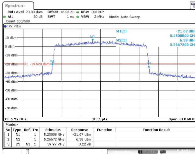
Fig. 15 Occupied 26dB Bandwidth (802.11ax-HE40, 5270MHz)
