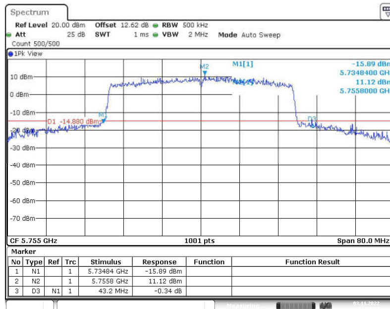
Fig. 20 Occupied 26dB Bandwidth (802.11ax-HE40, 5755MHz)
