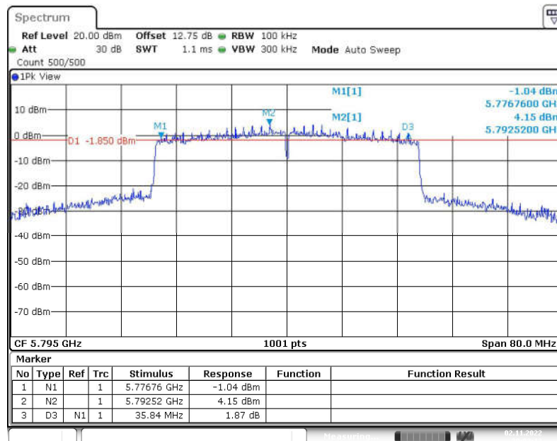
Fig. 33 Occupied 6dB Bandwidth (802.11ax-HE40, 5795MHz)
