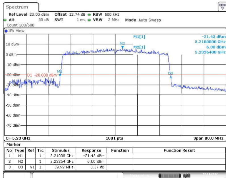
Fig. 14 Occupied 26dB Bandwidth (802.11ax-HE40, 5230MHz)
