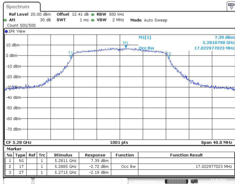
Fig. 39 99% Occupied Bandwidth (802.11a, 5280MHz)
