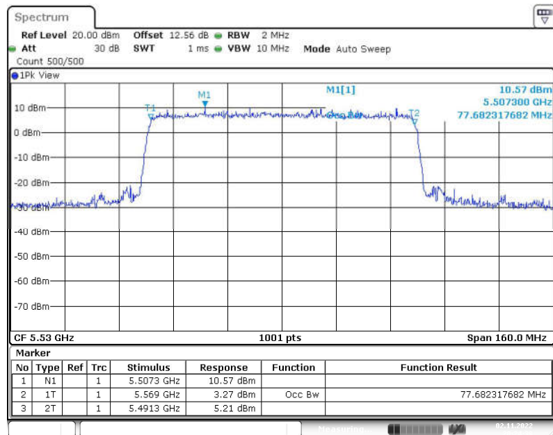
Fig. 58 99% Occupied Bandwidth (802.11ax-HE80, 5530MHz)
