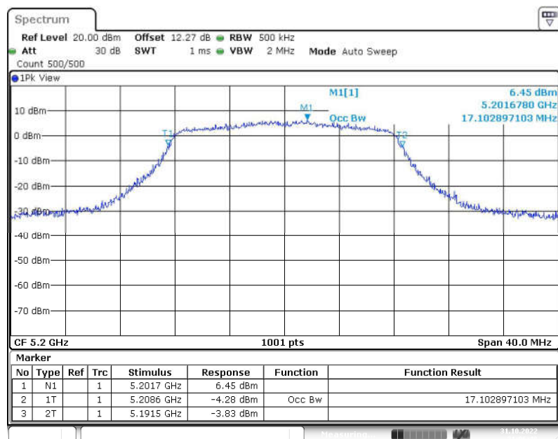
Fig. 36 99% Occupied Bandwidth (802.11a, 5200MHz)
