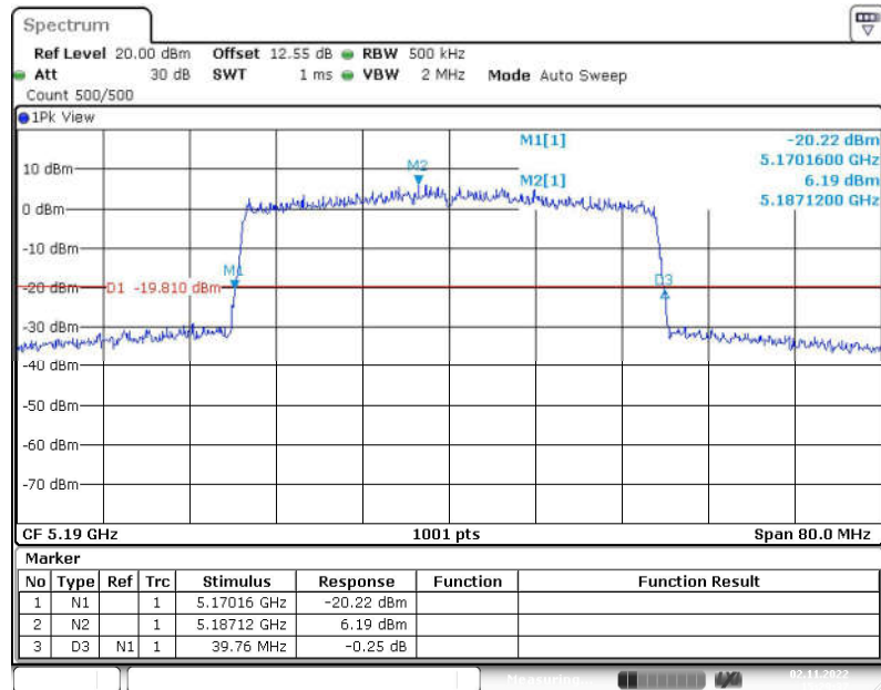
Fig. 13 Occupied 26dB Bandwidth (802.11ax-HE40, 5190MHz)
