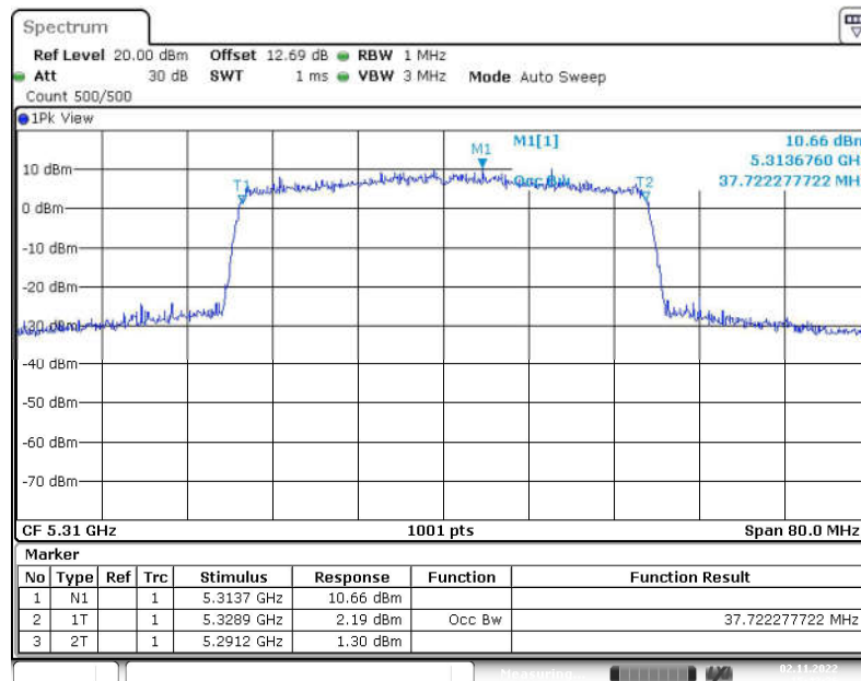
Fig. 50 99% Occupied Bandwidth (802.11ax-HE40, 5310MHz)
