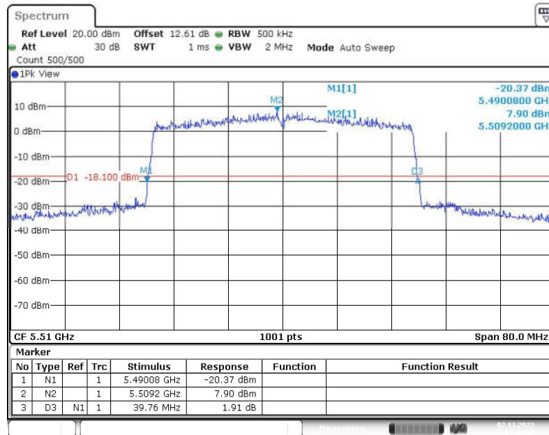
Fig. 17 Occupied 26dB Bandwidth (802.11ax-HE40, 5510MHz)
