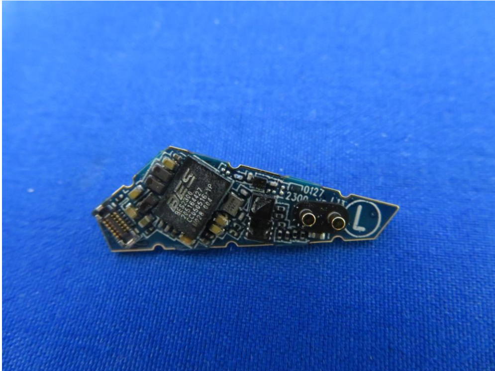
(21) EUT Photo (Left Earbud)
