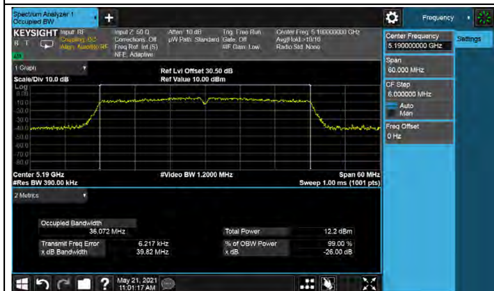
802.11ac-VHT40-5190MHz
