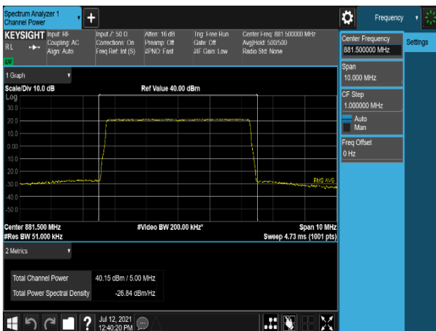
Plot 7-118. Conducted Average Output Power Plot (LTE_B5_5M_1C_QPSK - Mid Channel, Port 0)
