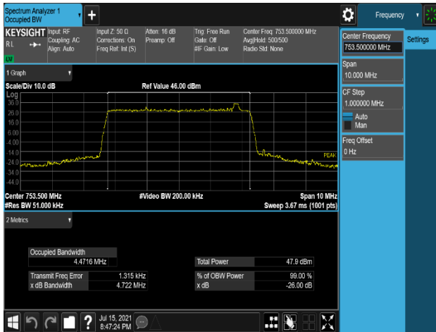
Plot 7-75. Occupied Bandwidth Plot (LTE_B13_5M+NB-lot(IB)_1C_QPSK - High Channel, Port 0)
