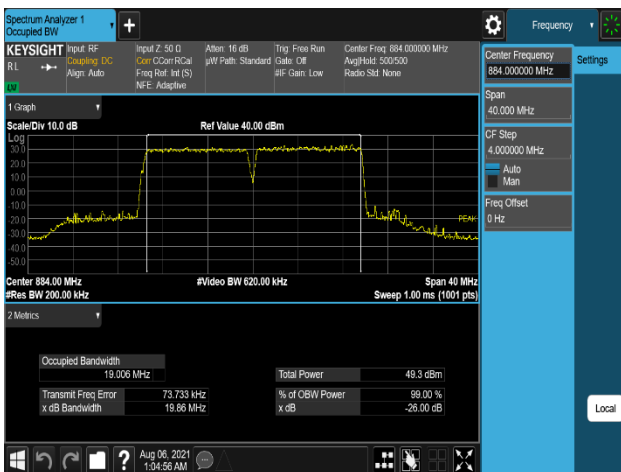
Plot 7-108. Occupied Bandwidth Plot (DSS_B5_10M+10M_2C_64QAM - High Channel, Port 0)
