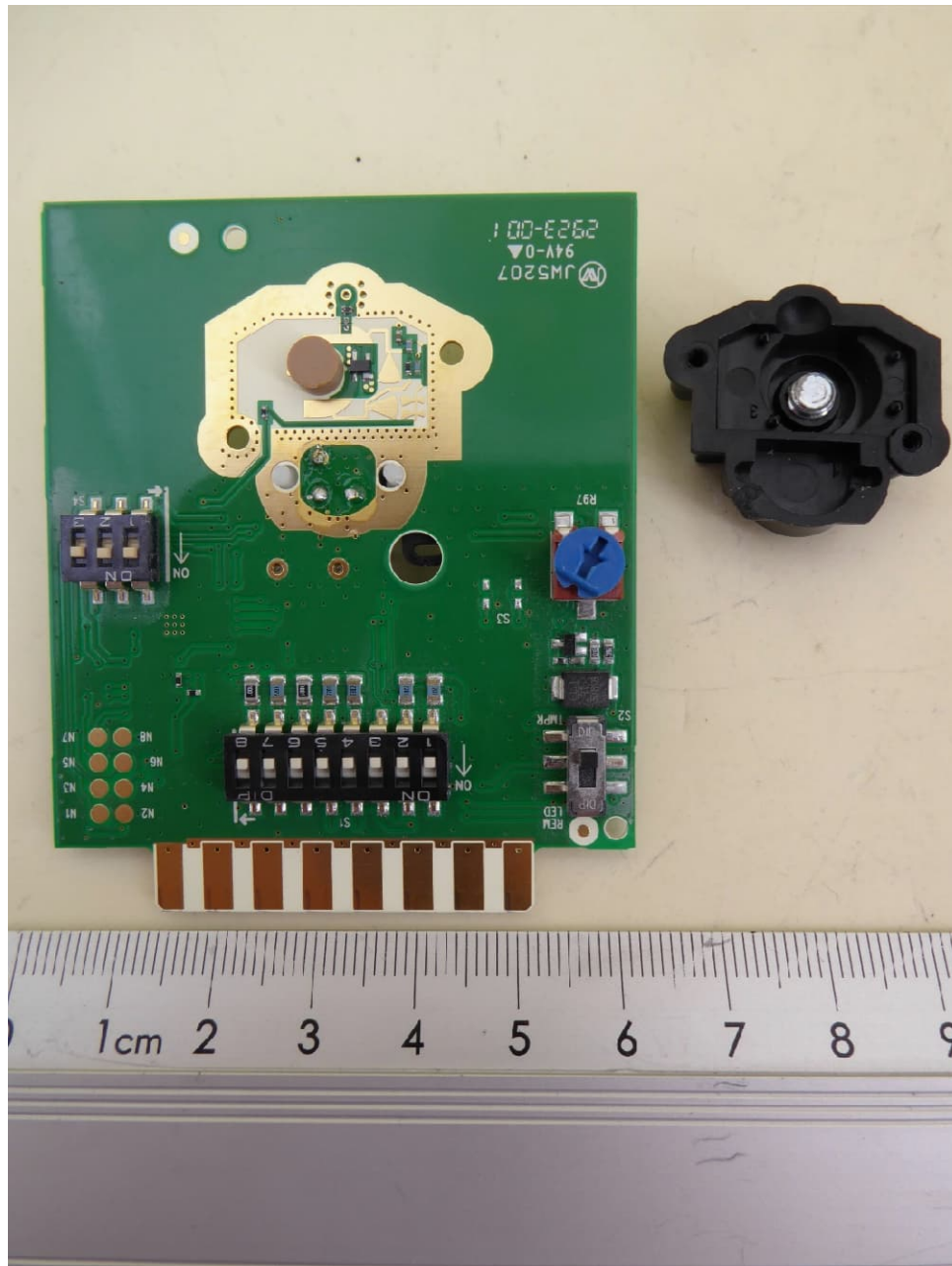
PCB, top view (PCB cover removed)
