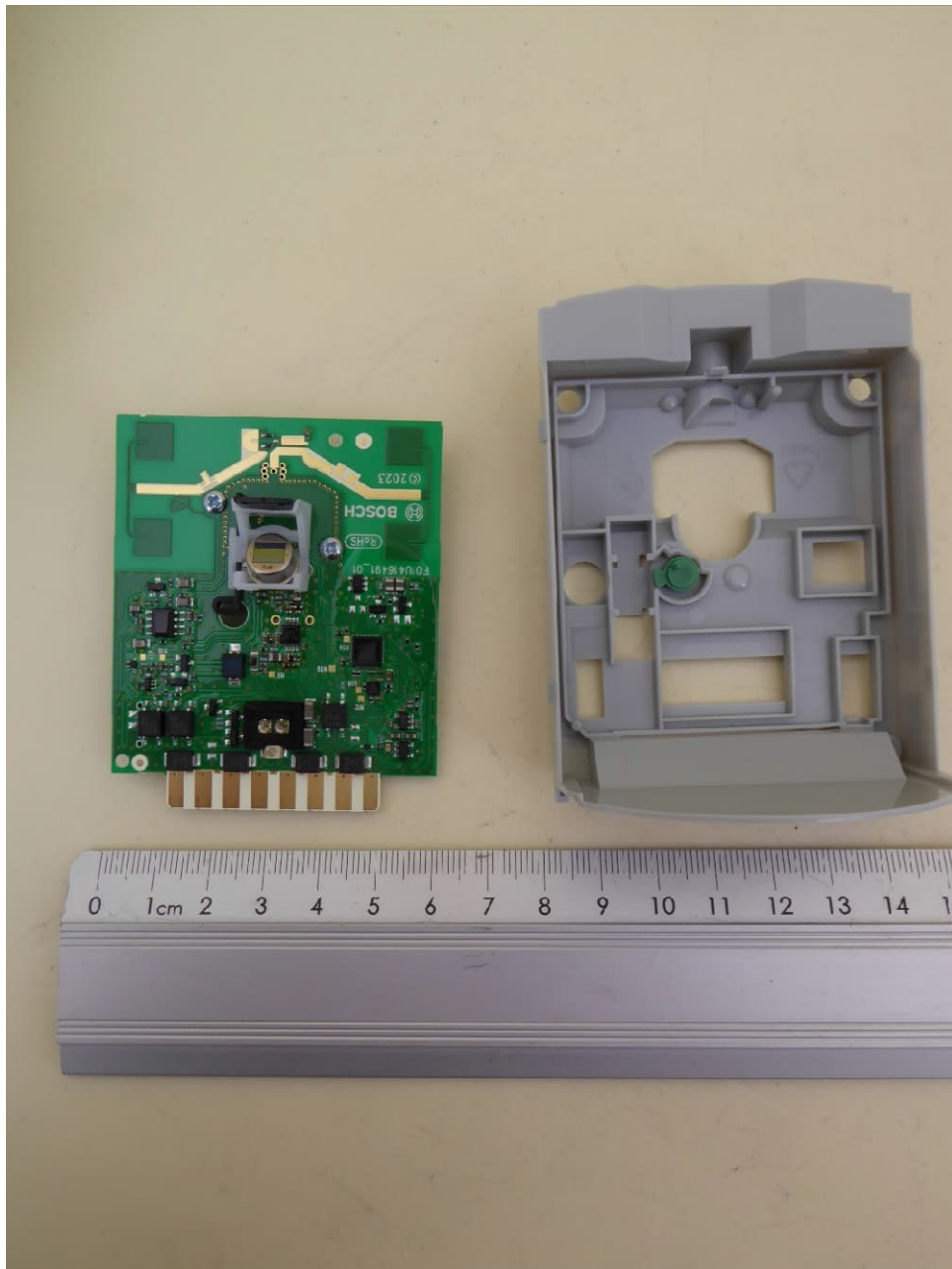
Internal view, PCB removed
