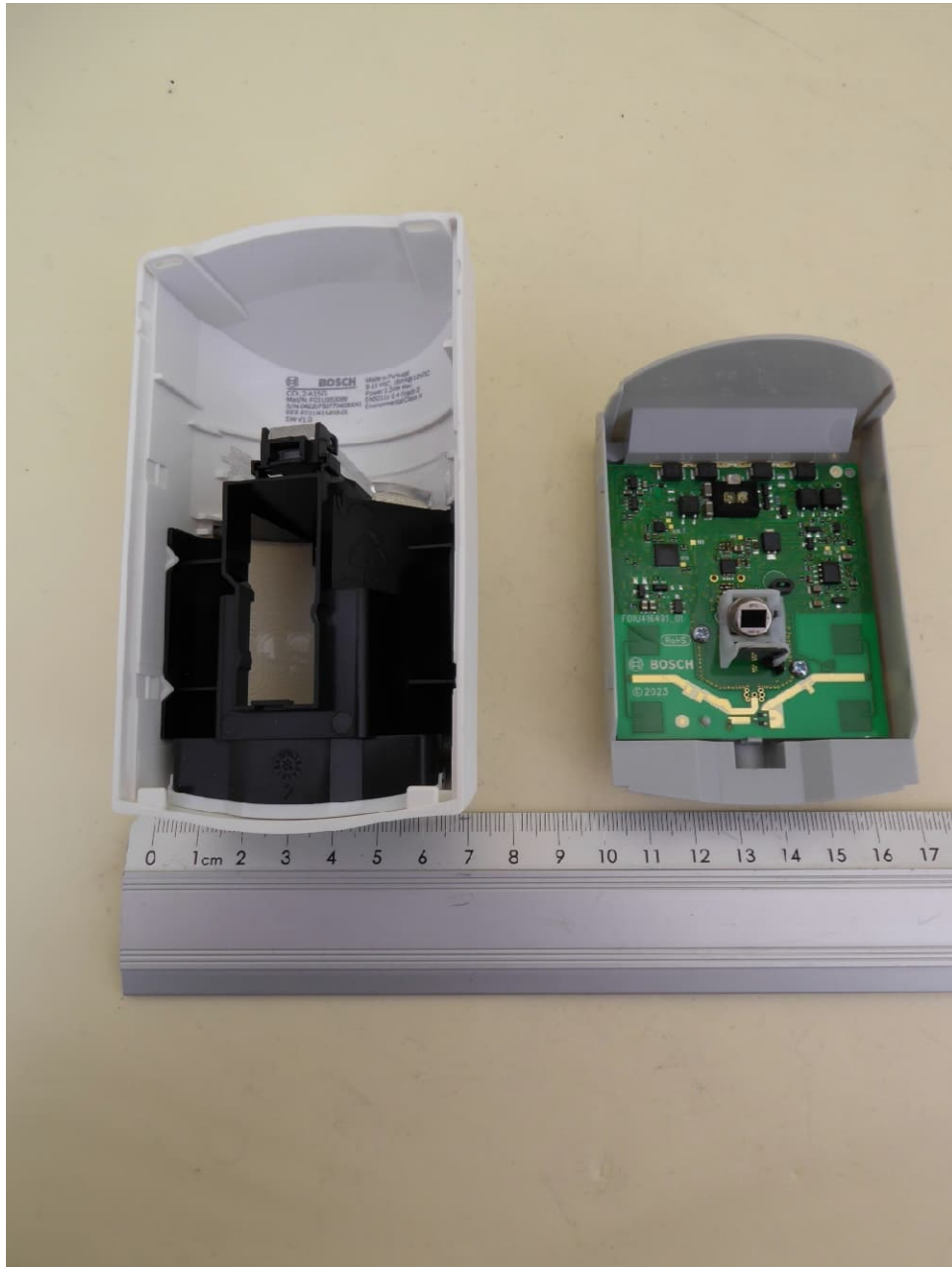
Internal view (cover removed)
