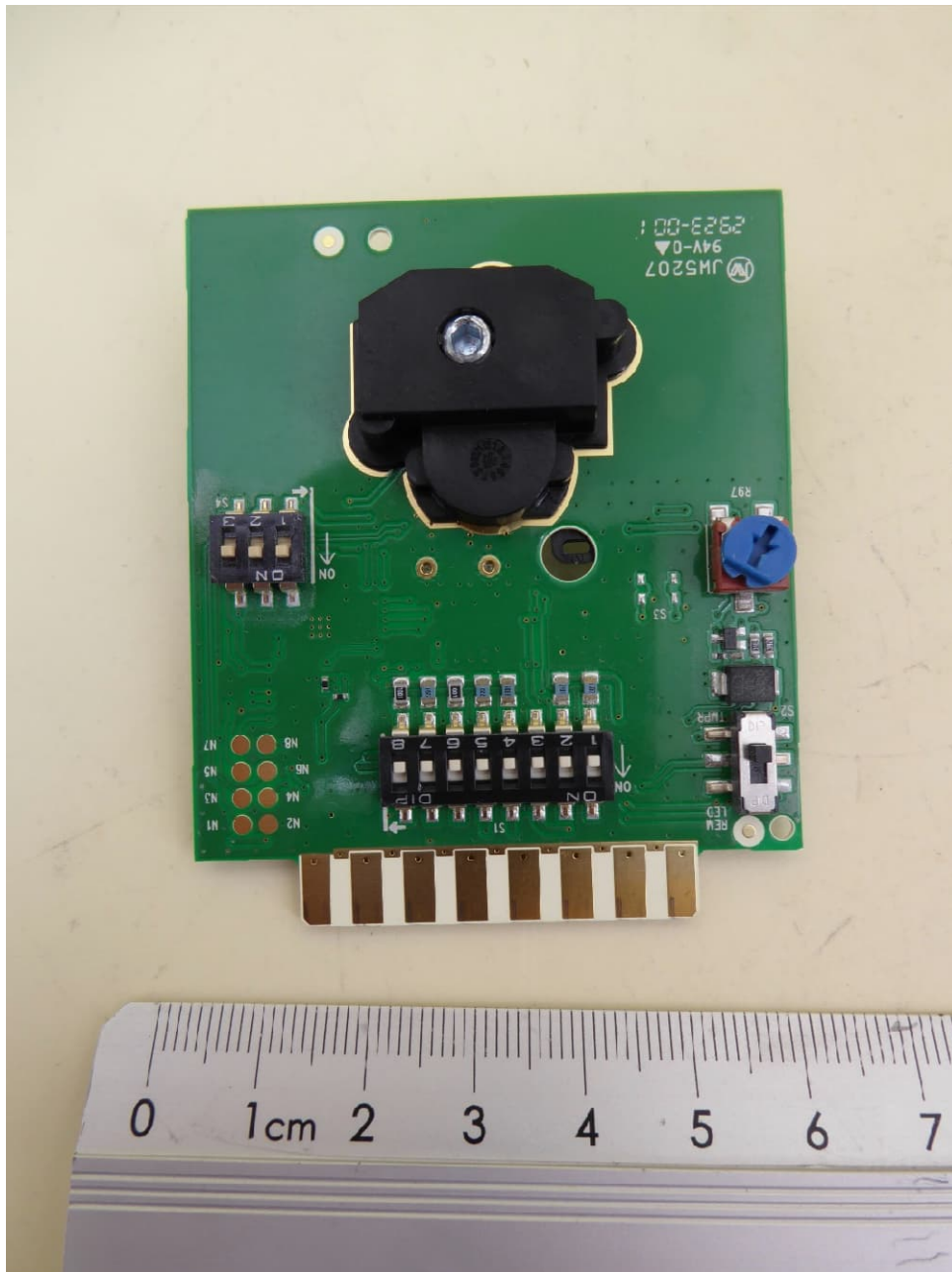
PCB, top view
