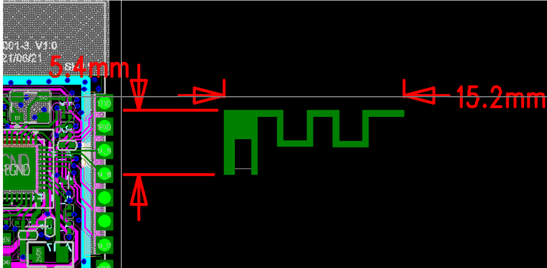
4.2.2 WIFI Antennatype: PCBantenna
