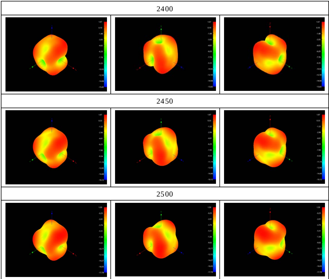
4.2.3 Bluetooth antenna pattern pictuter
