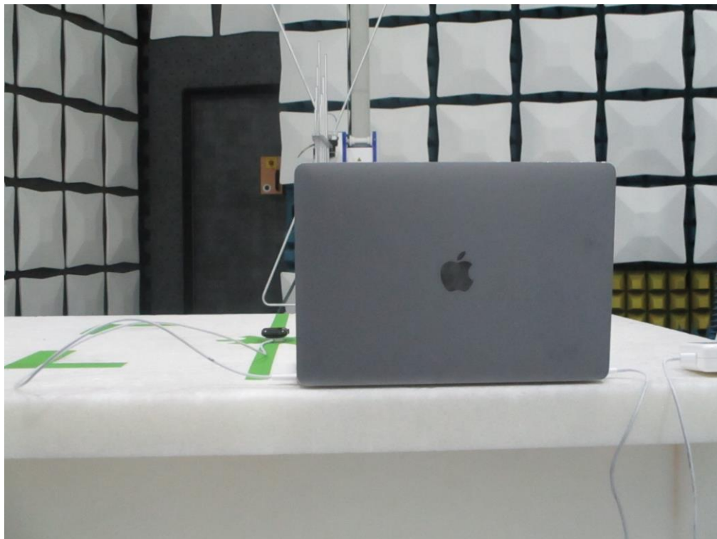
Figure 18: 30MHz-1GHz Test Setup (Rear View)
