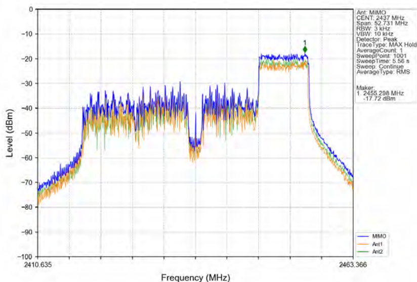
802.11ax(HE40) MCH 2437MHz RU106 Right MIMO NTN
