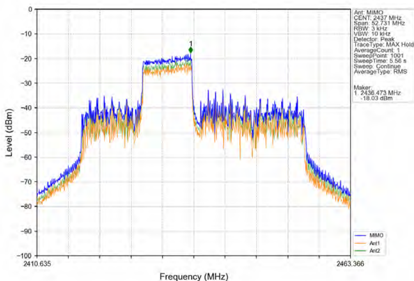
802.11ax(HE40) MCH 2437MHz RU106 Right Ant1 (MIMO) NTN
