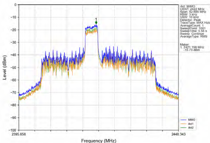
802.11ax(HE40) LCH_2422MHz_RU52_Mid_MIMO NTN
