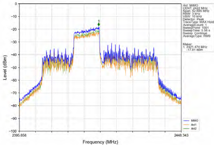
802.11ax(HE40) LCH 2422MHz RU106 Right Ant1 (MIMO) NTN
