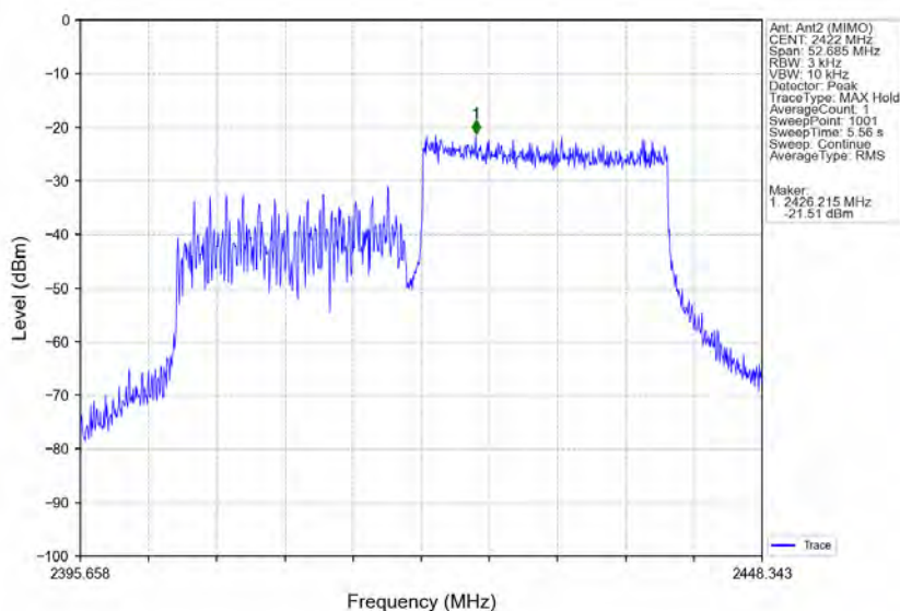
802.11ax(HE40) LCH 2422MHz RU242 Right MIMO NTN
