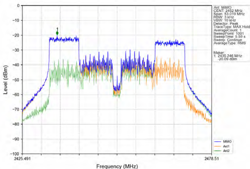
802.11ax(HE40) HCH 2452MHz RU106 Right MIMO NTN
