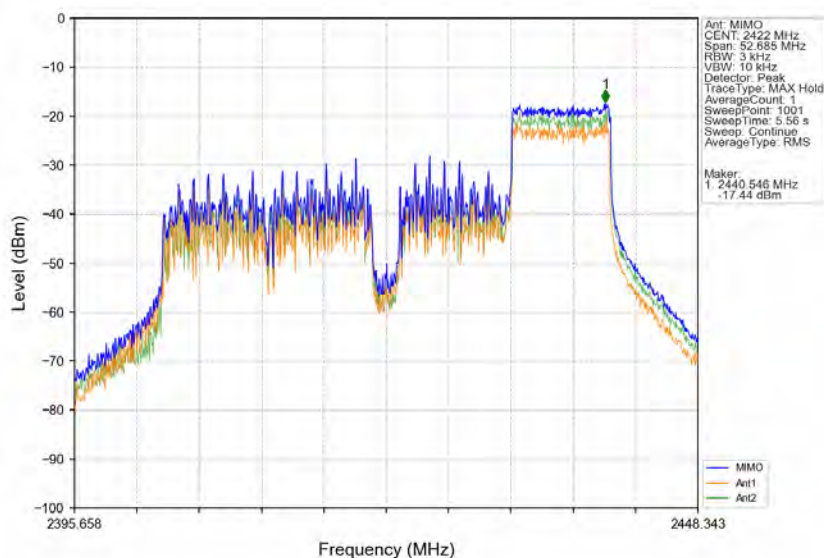
802.11ax(HE40) LCH_2422MHz_RU106_Right MIMO NTN
