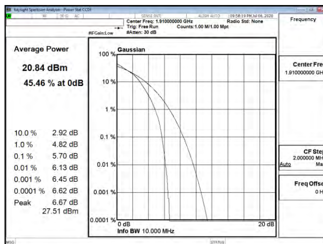
PTAR B25 10M CH26640 16QAM
