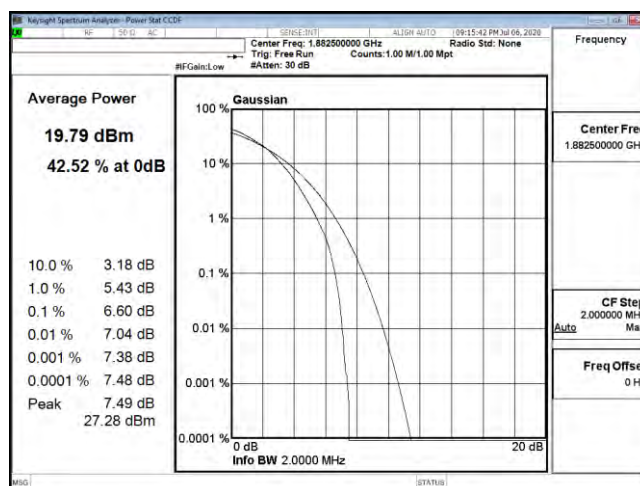
PTAR B25 1.4M CH26365 64QAM
