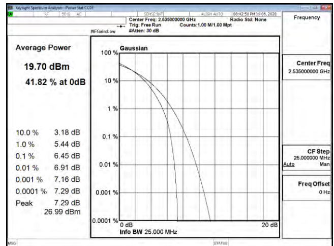
PTAR B7 15M CH21100 64QAM
