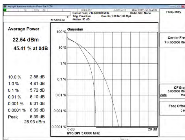
PTAR B12 3M CH23165 16QAM
