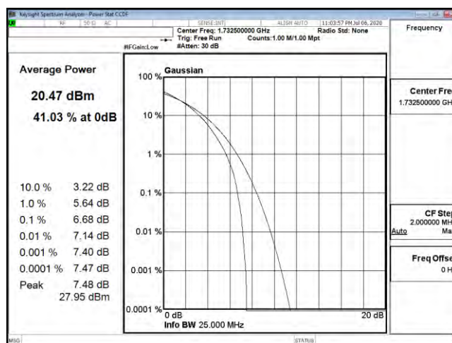
PTAR B4 15M CH20175 64QAM
