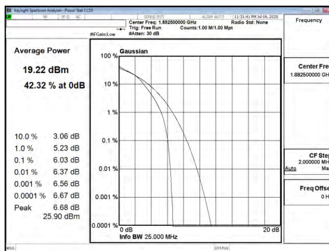
PTAR B25 15M CH26365 16QAM
