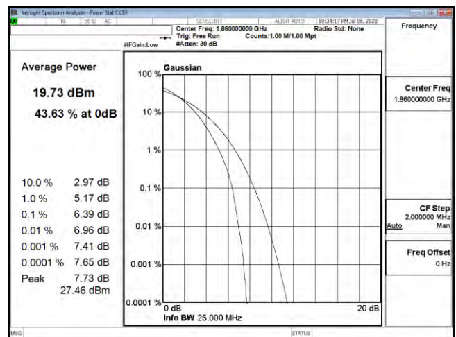
PTAR B25 20M CH26140 64QAM
