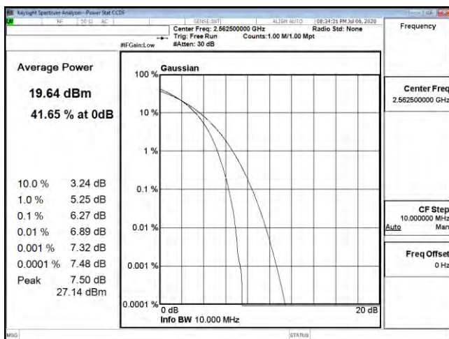
PTAR B7 15M CH21375 64QAM
