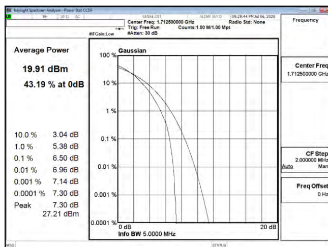
PTAR B4 5M CH19975 64QAM
