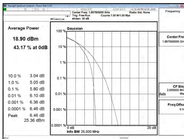
PTAR B25 15M CH26115 16QAM
