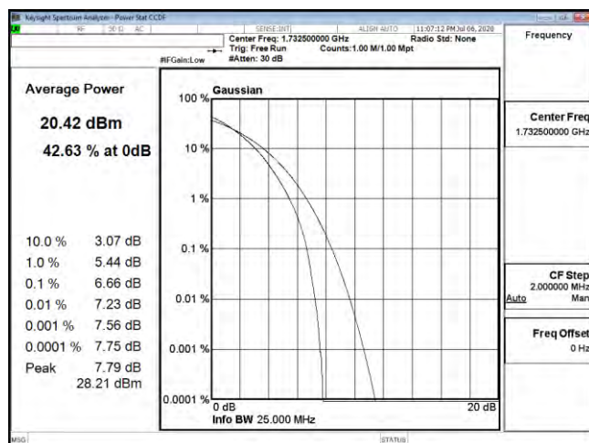
PTAR B4 20M CH20175 64QAM
