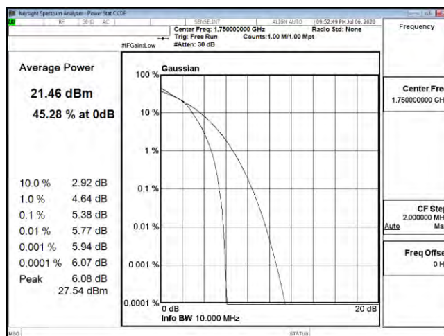
PTAR B4 10M CH20350 16QAM
