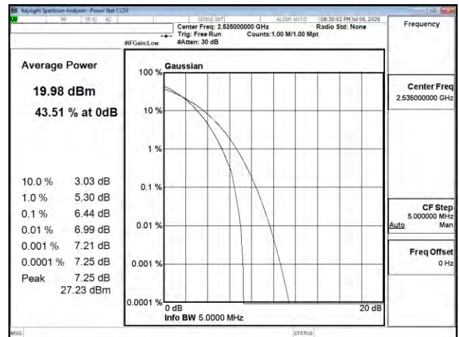
PTAR B7 5M CH21100 64QAM
