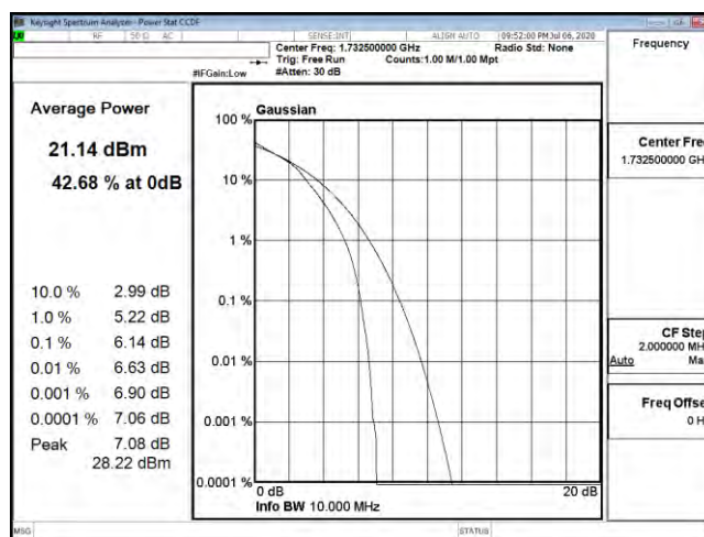
PTAR B4 10M CH20175 16QAM
