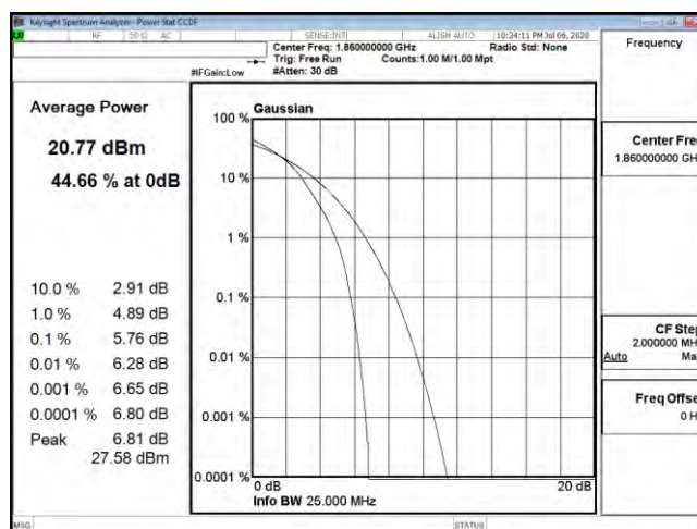
PTAR B25 20M CH26140 16QAM
