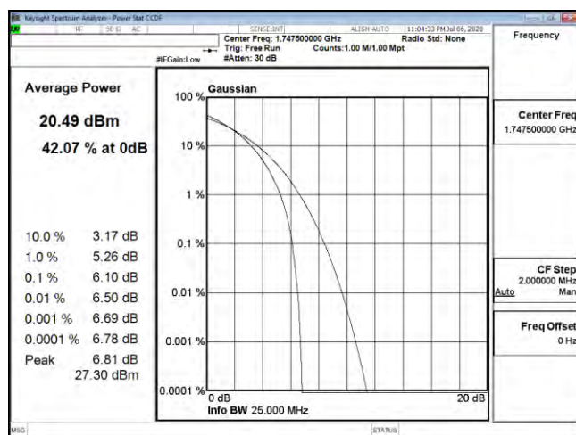
PTAR B4 15M CH20325 64QAM
