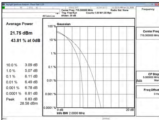
PTAR B12 1.4M CH23173 64QAM
