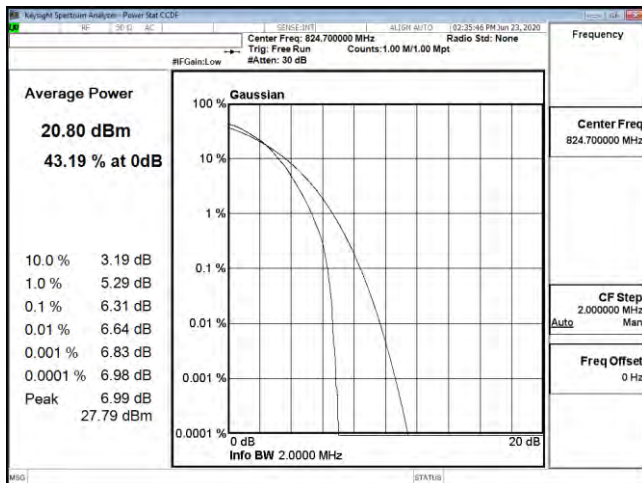
PTAR B26 1.4M CH26797 64QAM
