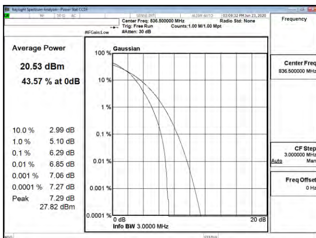
PTAR B26 3M CH26915 64QAM
