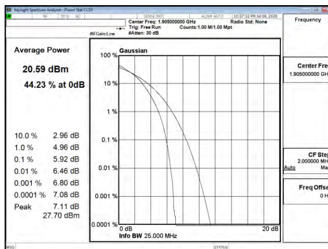
PTAR B25 20M CH26590 16QAM
