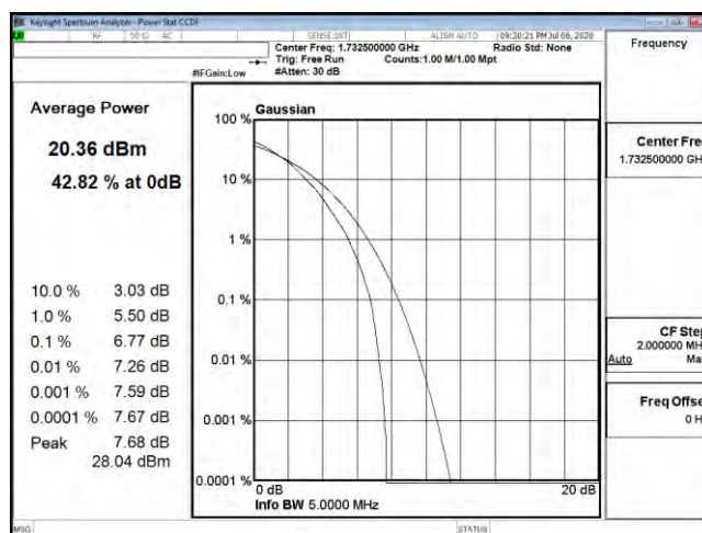
PTAR B4 5M CH20175 64QAM
