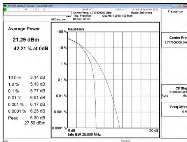
PTAR B4 15M CH20025 16QAM
