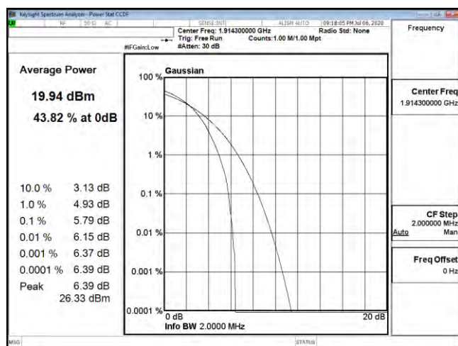
PTAR B25 1.4M CH26683 64QAM
