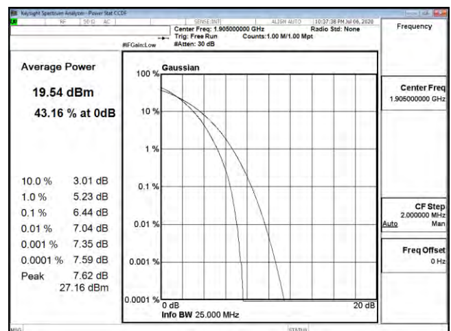
PTAR B25 20M CH26590 64QAM
