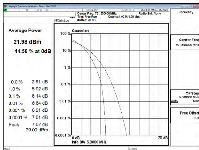
PTAR B12 5M CH23035 64QAM
