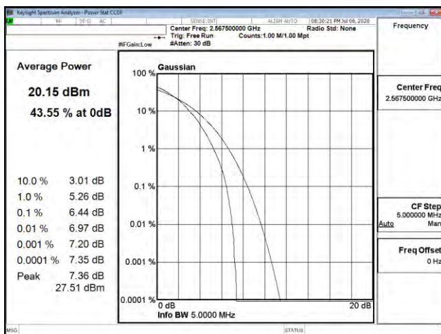
PTAR B7 5M CH21425 64QAM
