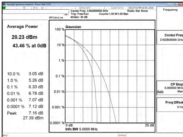
PTAR B7 5M CH20775 64QAM
