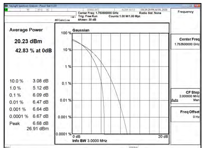
PTAR B4 3M CH20385 64QAM
