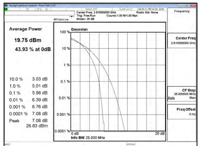
PTAR B7 20M CH20850 64QAM
