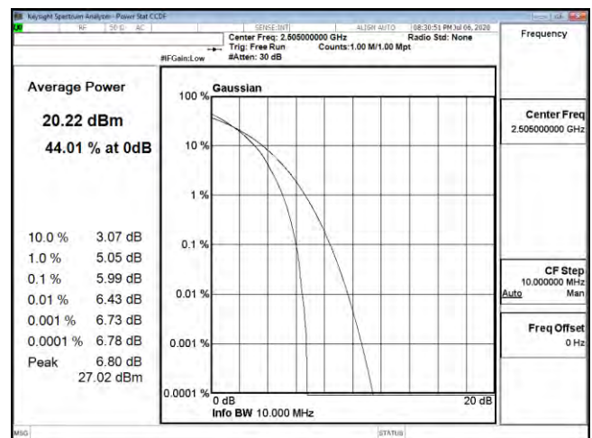
PTAR B7 10M CH20800 64QAM
