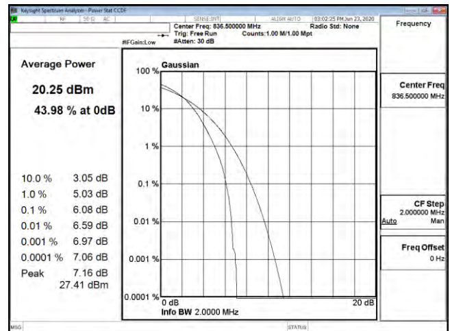
PTAR B26 1.4M CH26915 64QAM
