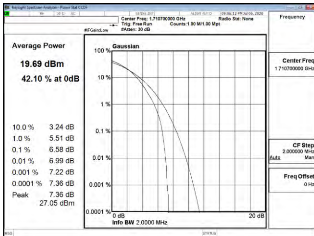
PTAR B4 1.4M CH19957 64QAM
