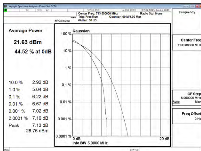
PTAR B12 5M CH23155 64QAM
