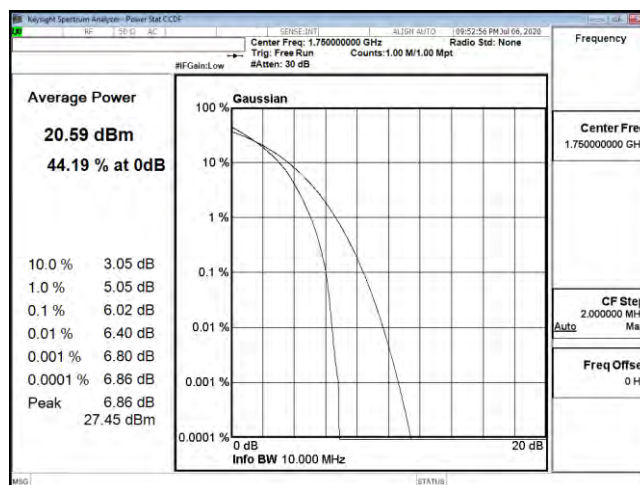
PTAR B4 10M CH20350 64QAM
