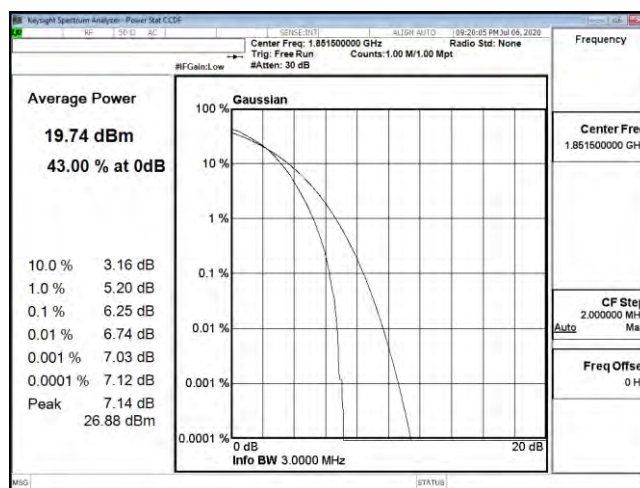
PTAR B25 3M CH26055 64QAM
