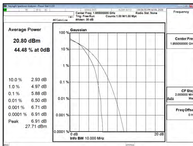
PTAR B25 10M CH26090 16QAM
