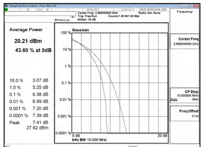
PTAR B7 10M CH21400 64QAM
