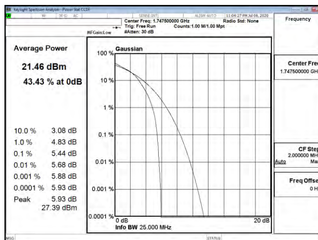
PTAR B4 15M CH20325 16QAM
