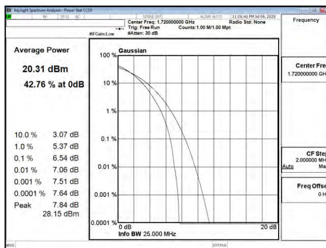
PTAR B4 20M CH20050 64QAM
