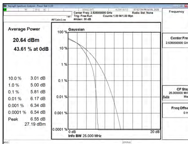
PTAR B7 15M CH21100 16QAM
