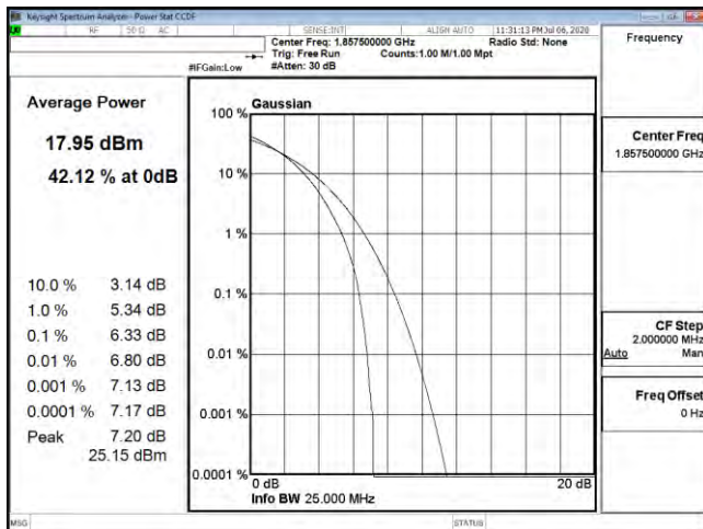
PTAR B25 15M CH26115 64QAM
