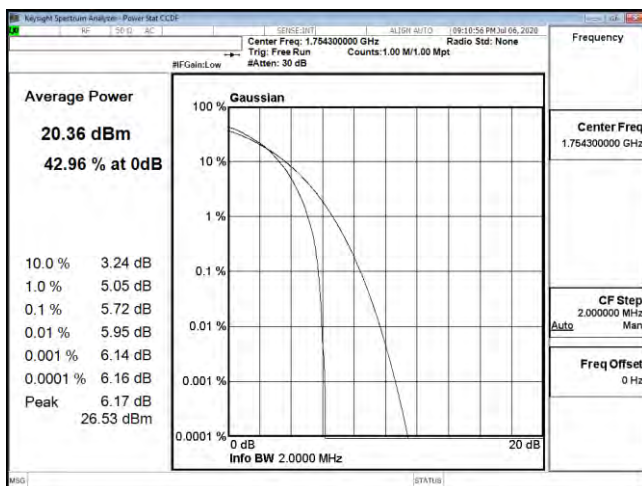
PTAR B4 1.4M CH20393 64QAM
