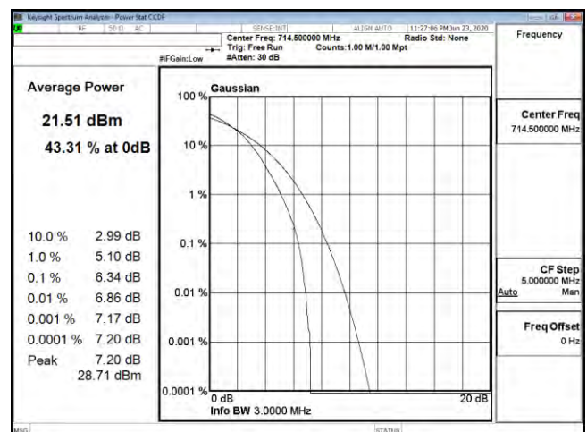
PTAR B12 3M CH23165 64QAM
