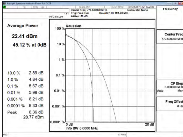
PTAR B13 5M CH23205 16QAM
