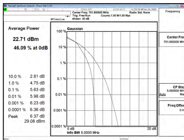
PTAR B12 5M CH23035 16QAM
