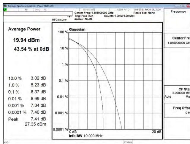
PTAR B25 10M CH26090 64QAM
