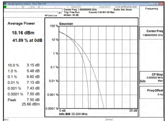
PTAR B25 15M CH26365 64QAM
