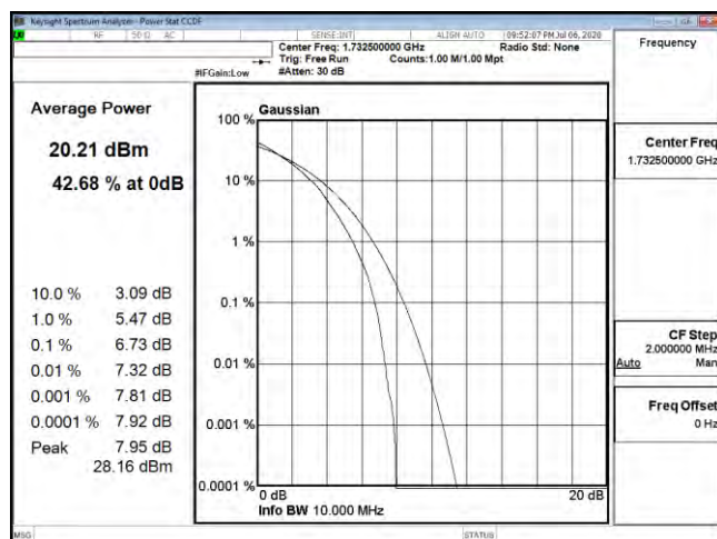
PTAR B4 10M CH20175 64QAM
