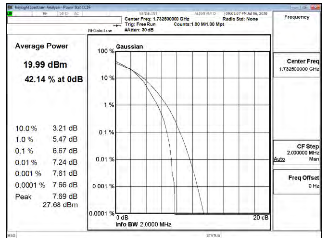
PTAR B4 1.4M CH20175 64QAM
