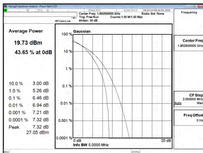
PTAR B25 5M CH26065 64QAM
