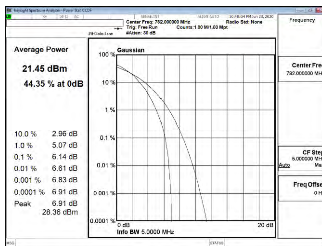
PTAR B13 5M CH23230 64QAM
