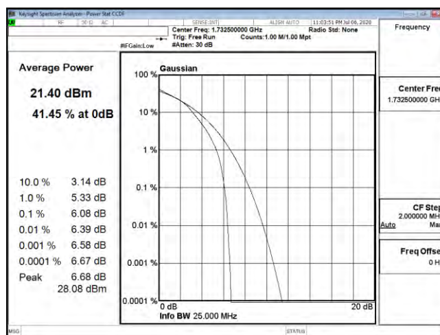
PTAR B4 15M CH20175 16QAM
