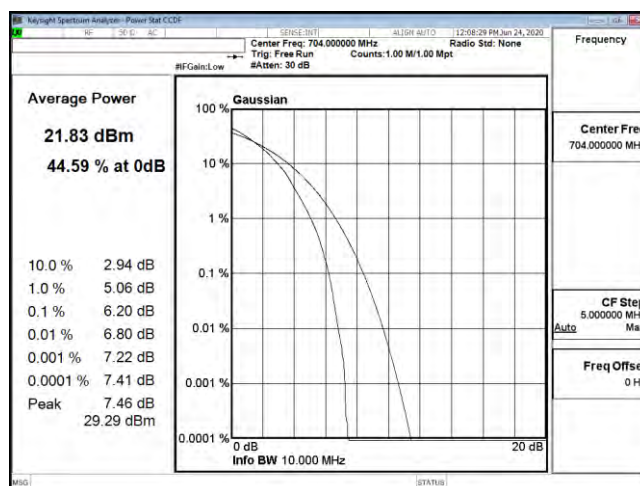
PTAR B12 10M CH23060 64QAM
