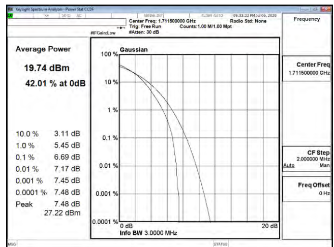
PTAR B4 3M CH19965 64QAM
