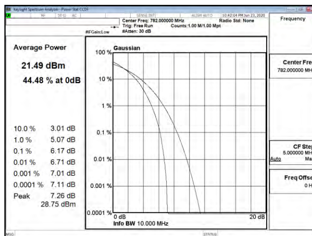
PTAR B13 10M CH23230 64QAM
