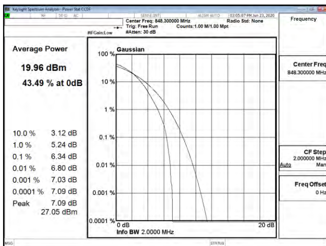
PTAR B26 1.4M CH27033 64QAM
