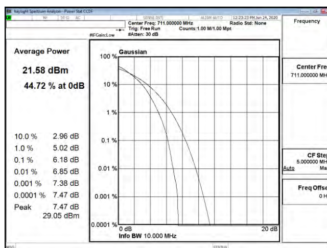
PTAR B12 10M CH23130 64QAM
