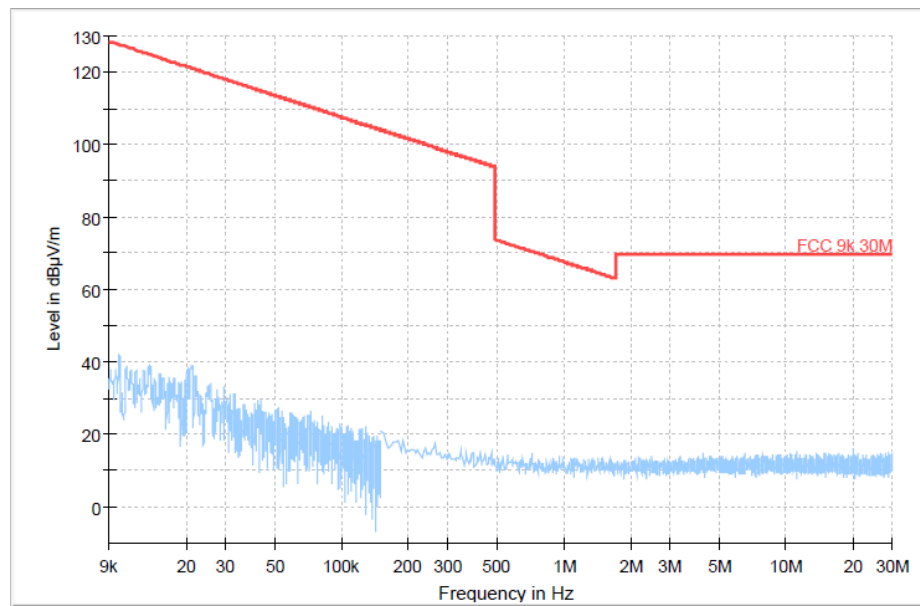
Fig.22 Radiated Spurious Emission (Ch19, 9 kHz - 30 MHz), 1M
