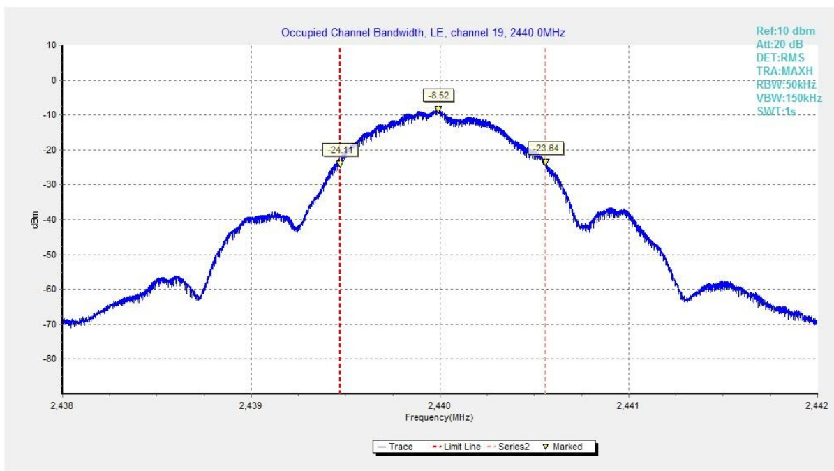
Fig.36 Occupied Bandwidth (Ch 19), 1M
