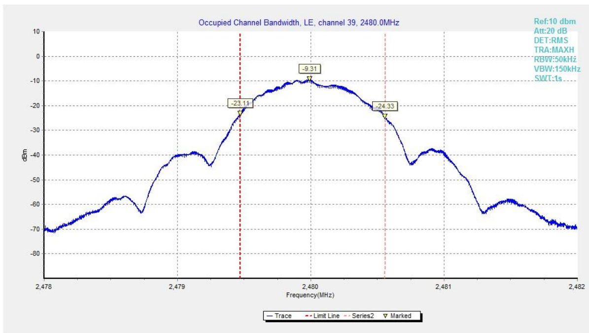
Fig.37 Occupied Bandwidth (Ch 39), 1M
