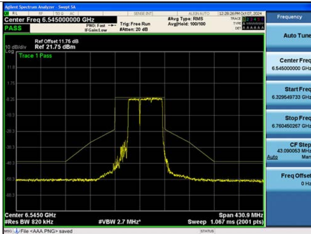
802.11be EHT80M Ch.119(6545 MHz) 484T+242T RU90
