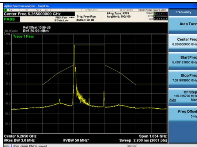
Bandwidth 320M, Ch. 63(6265 MHz) 242 Tones 61 RU
