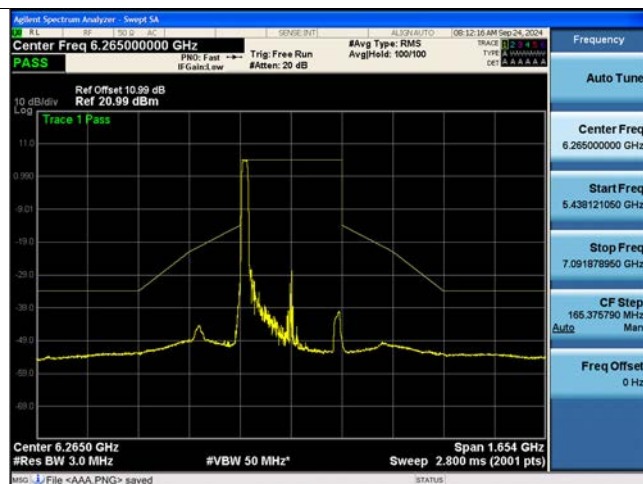
Bandwidth 320M, Ch. 63(6265 MHz) 996 Tones 67 RU
