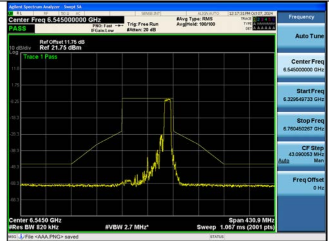
802.11be EHT80M Ch.119(6545 MHz) 106T+26T RU89
