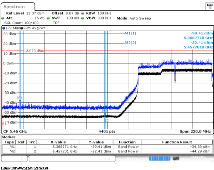
BE-R-LOW, MIMO-B, 802.11ac160-VHT0, Ch114
