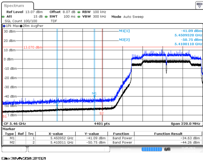
BE-R-LOW, MIMO-B, 802.11ac80-VHT0, Ch106
