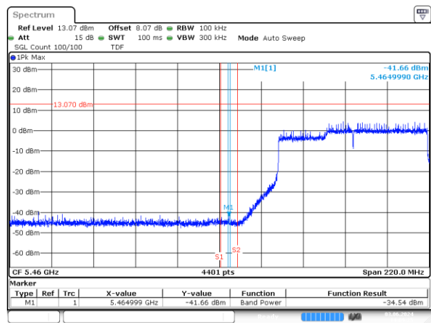
BE-NR-LOW, MIMO-B, 802.11ax/be160-MCS0, Ch114
