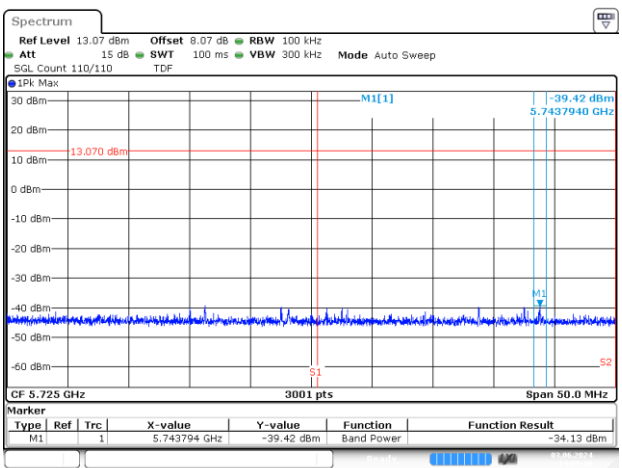
BE-NR-HIGH, MIMO-B, 802.11ax/be160-MCS0, Ch114
