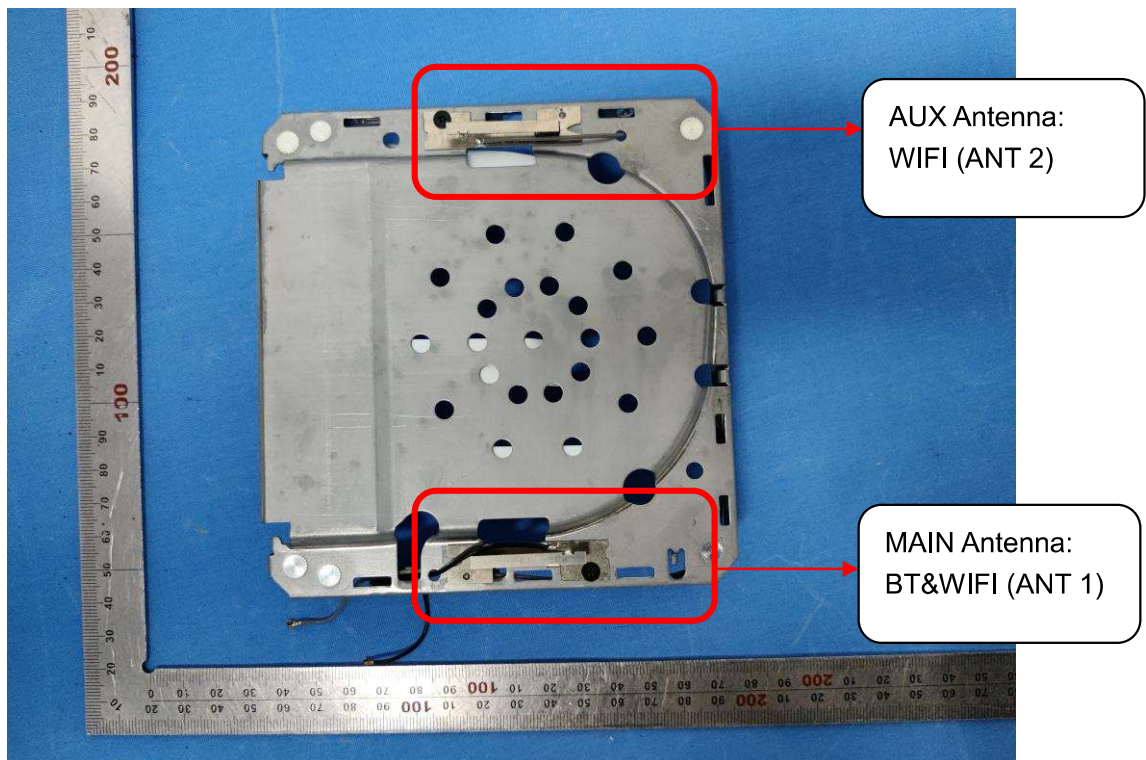
INTERNAL VIEW-10 OF EUT
