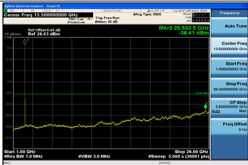
Band7-15MHz-16QAM-20825-1RB#0-1000~26000MHz
