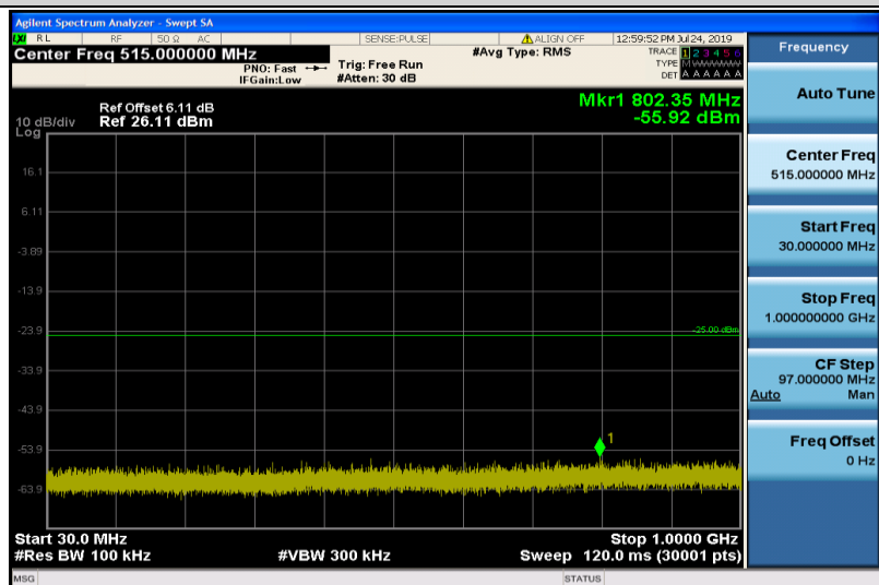
Band7-20MHz-16QAM-21100-1RB#0-30~1000MHz
