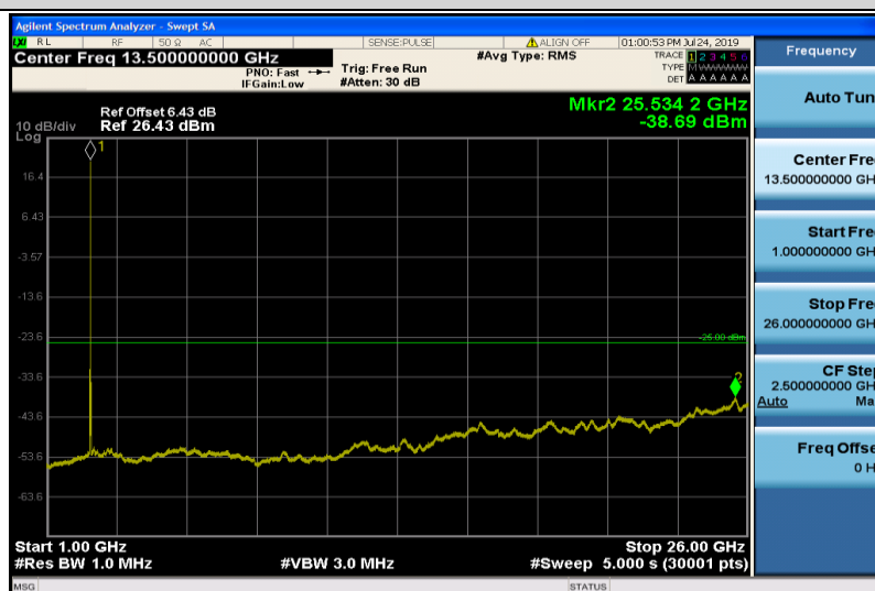
Band7-20MHz-QPSK-21350-1RB#0-1000~26000MHz
