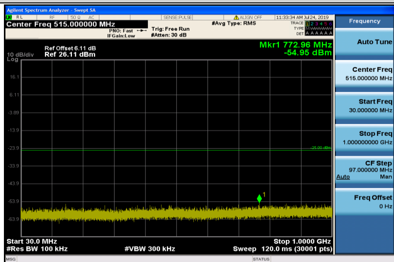
Band7-15MHz-16QAM-21100-1RB#0-30~1000MHz
