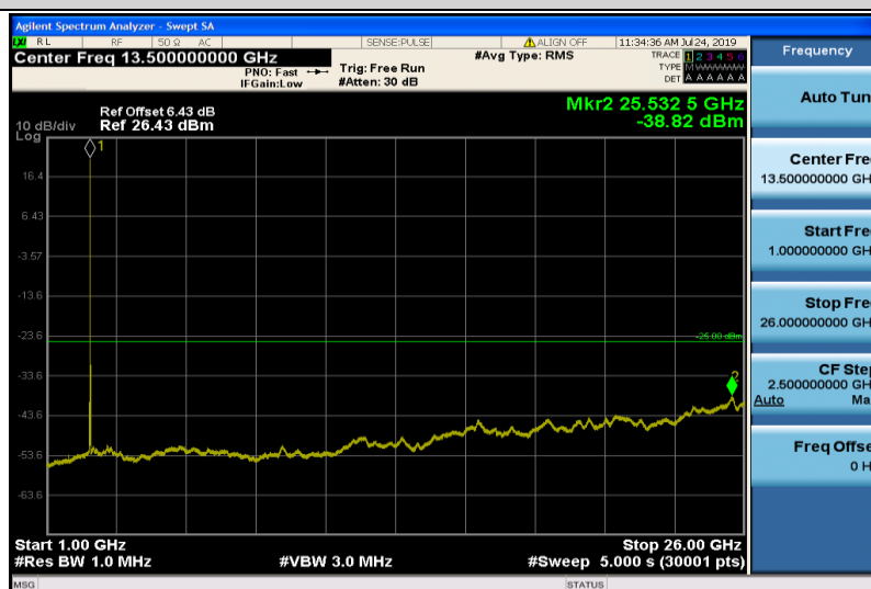
Band7-15MHz-QPSK-21375-1RB#0-1000~26000MHz
