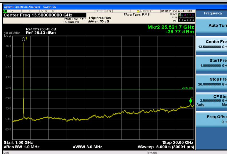
Band7-20MHz-16QAM-21350-1RB#0-1000~26000MHz
