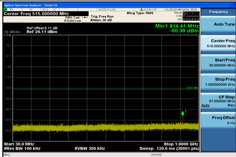
Band7-15MHz-16QAM-20825-1RB#0-30~1000MHz
