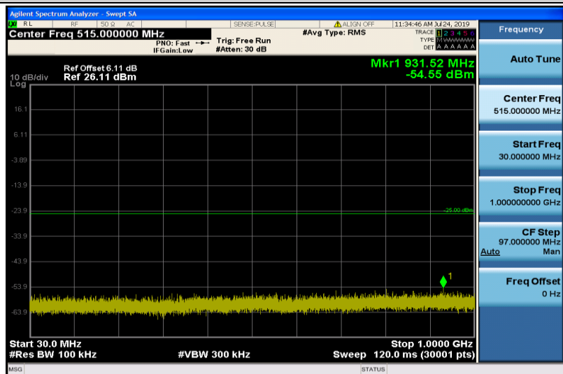
Band7-15MHz-16QAM-21375-1RB#0-30~1000MHz
