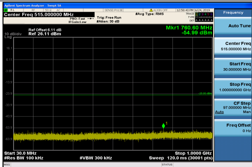
Band7-20MHz-16QAM-20850-1RB#0-30~1000MHz
