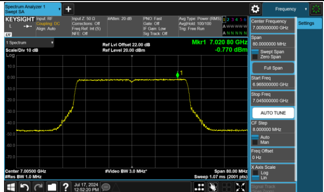
Channel 211 (7005MHz)
