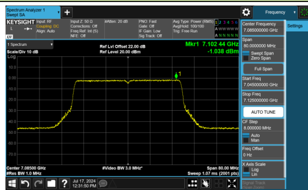
Channel 227 (7085MHz)
