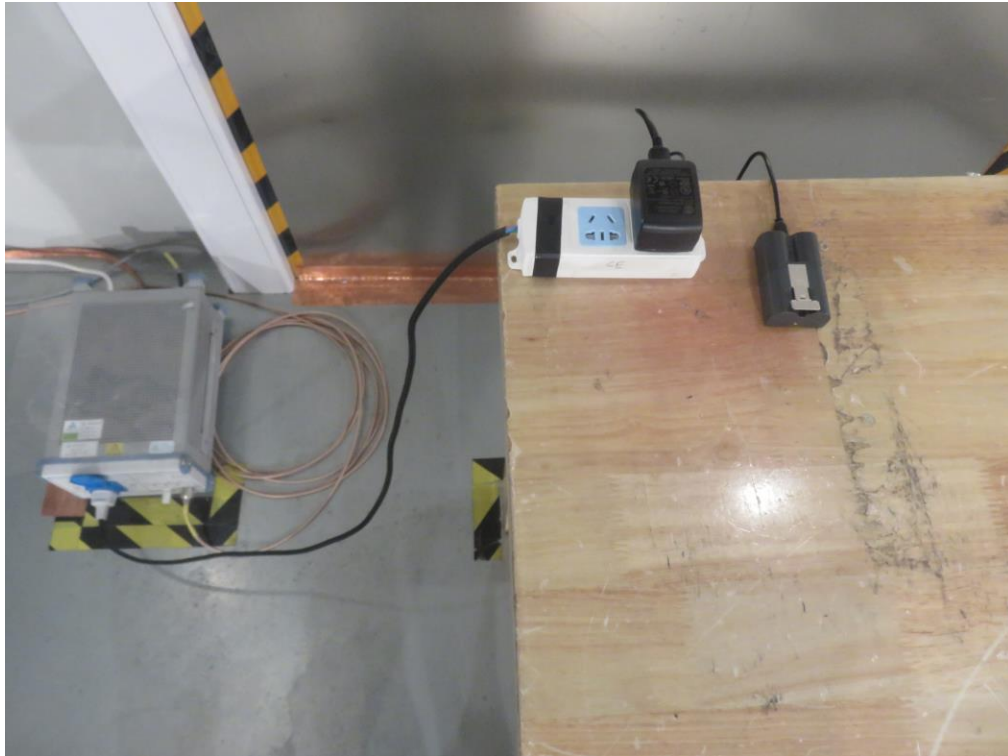
Photograph 3: Set-up for Conducted Emission, battery charging
