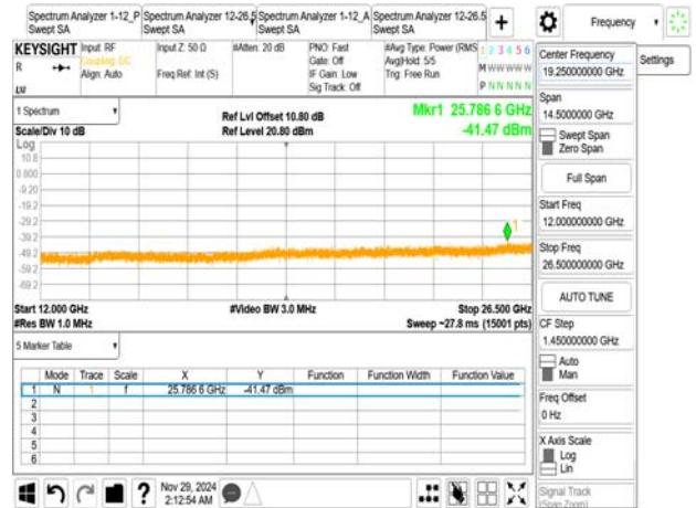
802.11ax_40MHz_2462MHz_RU242_62
