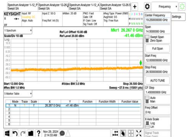
802.11ax_40MHz_2462MHz_RU484
