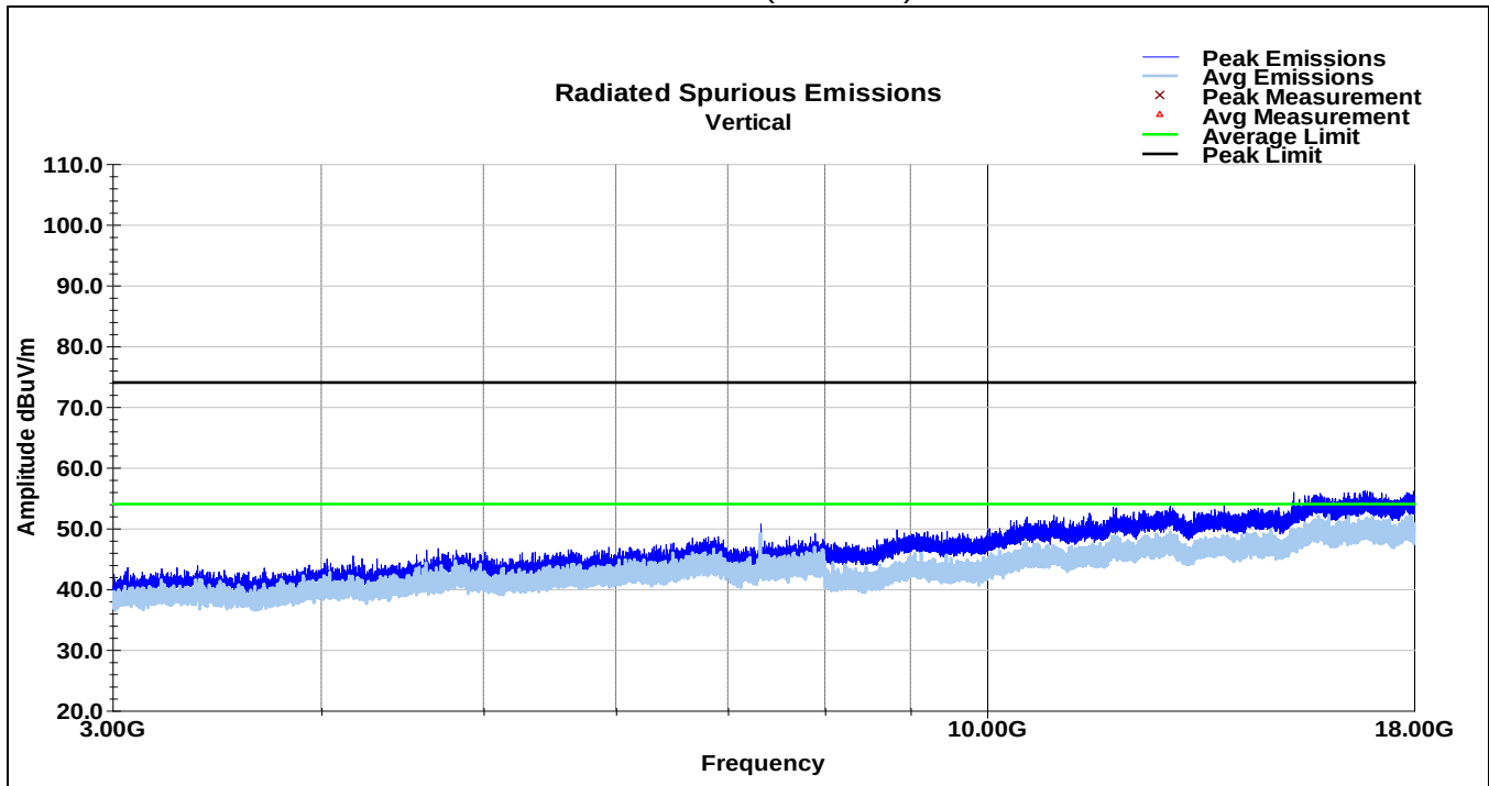
BLE Channel 19 Vertical Plot (3-18GHz)
