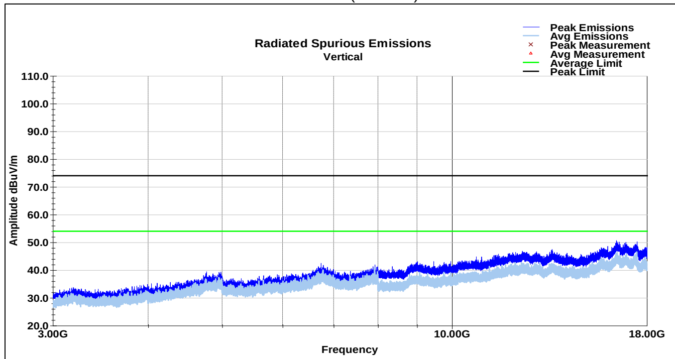
BLE Channel 0 Vertical Plot (3-18GHz)
