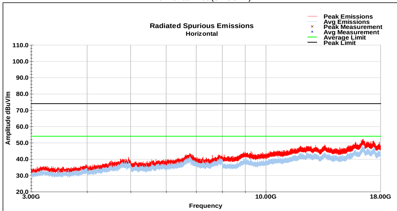
BLE Channel 0 Horizontal Plot (3-18GHz)
