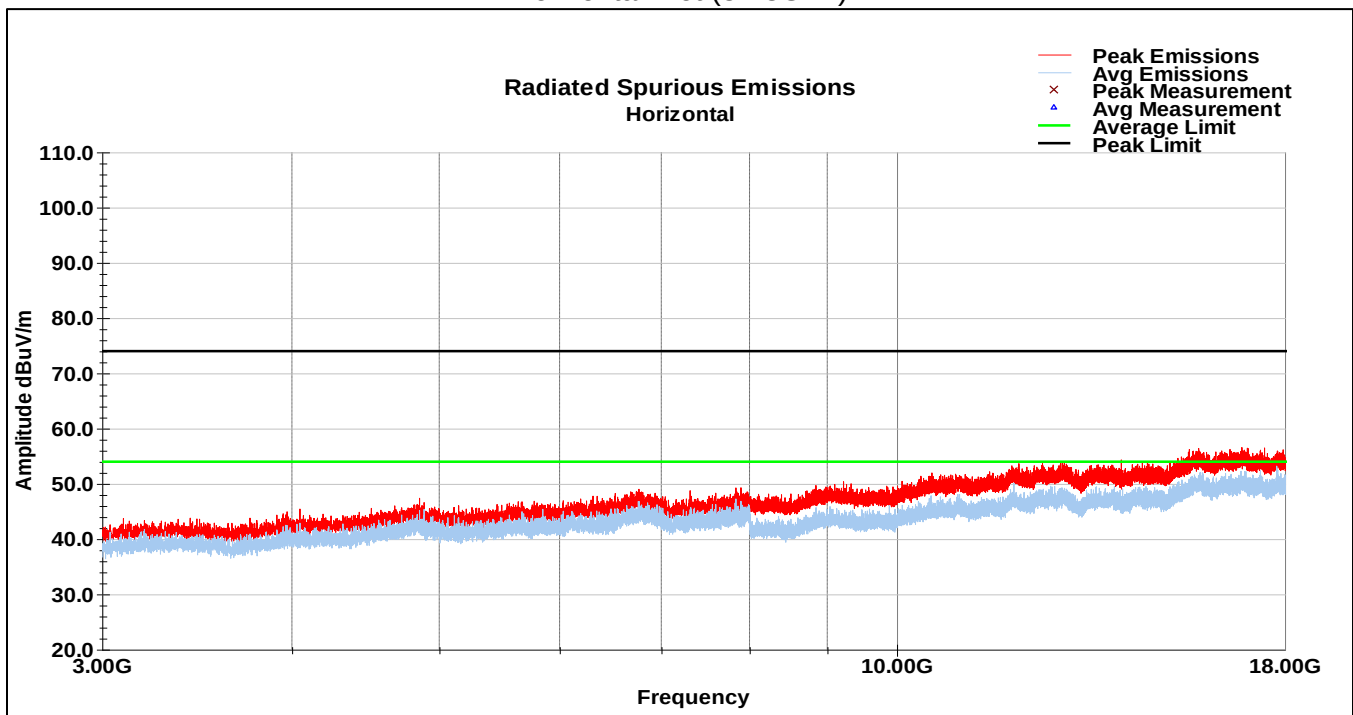
BLE Channel 19 Horizontal Plot (3-18GHz)
