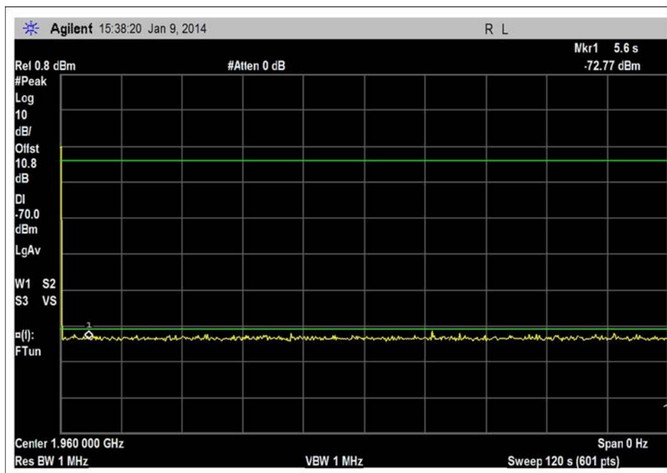
DL_1930-1995MHz_single_120sec
