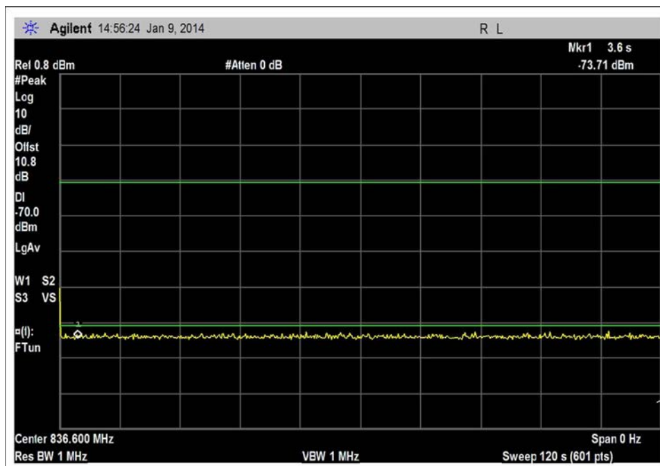
UL_824-849MHz_single_120sec
