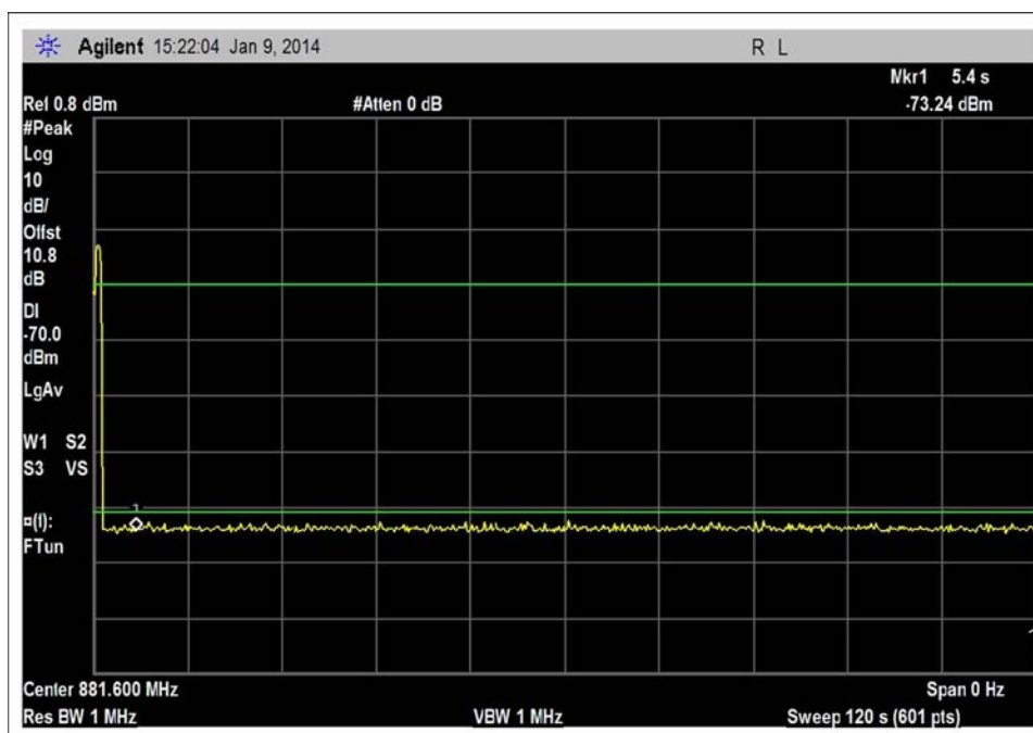
DL_869-894MHz_single_120sec
