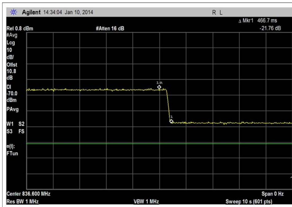
UL time_824-849MHz
