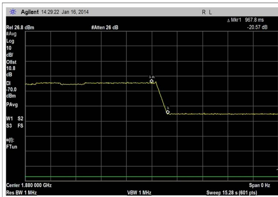
UL time_1850-1915MHz_011614
