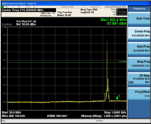
Band5_10MHz_16QAM_20600_1RB#0_30~1000_30~1000
