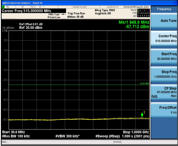
Band7_15MHz_16QAM_20825_1RB#0_30~1000_30~1000
