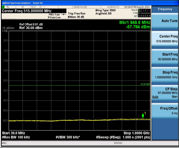
Band7_5MHz_16QAM_20775_1RB#0_30~1000_30~1000
