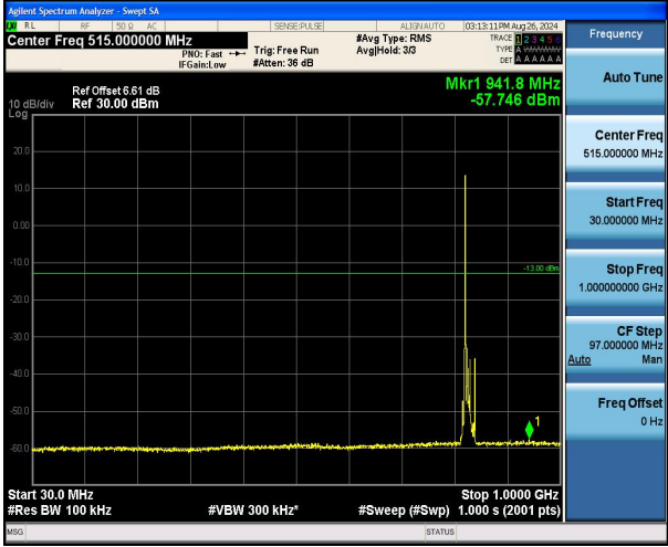
Band5_10MHz_16QAM_20450_1RB#0_30~1000_30~1000
