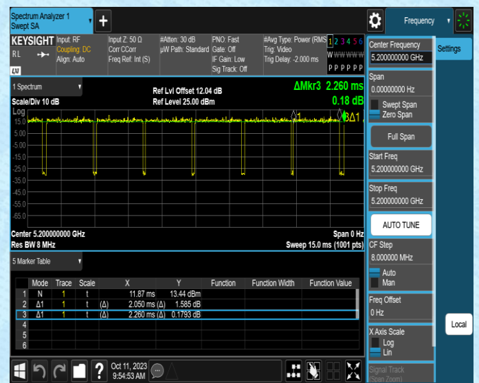
NTNV-11A-Ant2-5200
