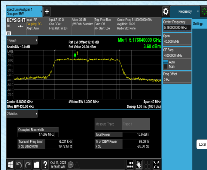
11AC20SISO-Ant1-5180
