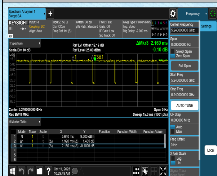
NTNV-11AC20MIMO-Ant1-5240
