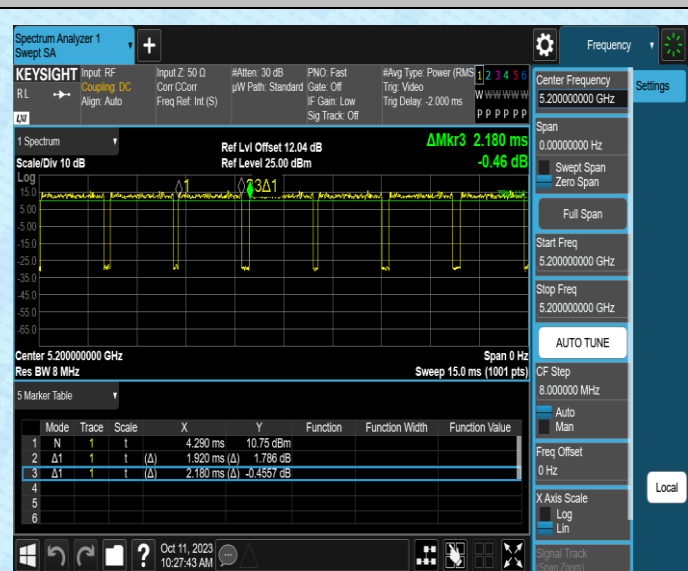
NTNV-11AC20MIMO-Ant2-5200
