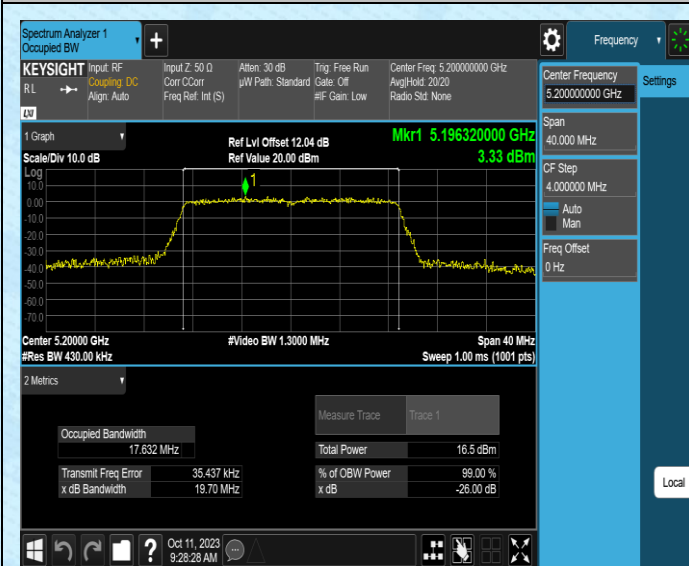
11AC20SISO-Ant1-5200
