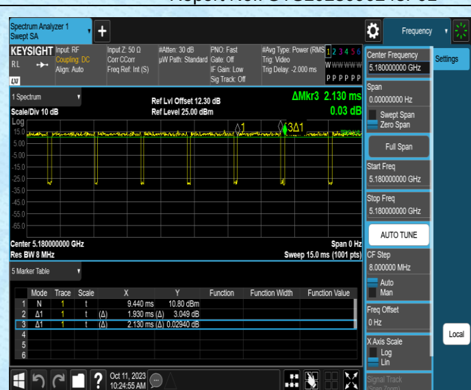
NTNV-11AC20MIMO-Ant2-5180
