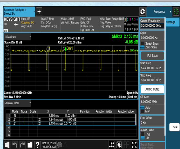
NTNV-11AC20MIMO-Ant2-5240
