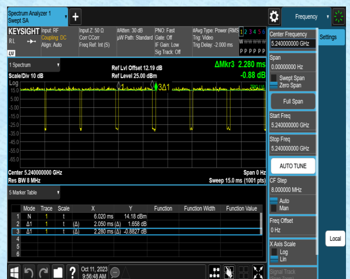
NTNV-11A-Ant2-5240
