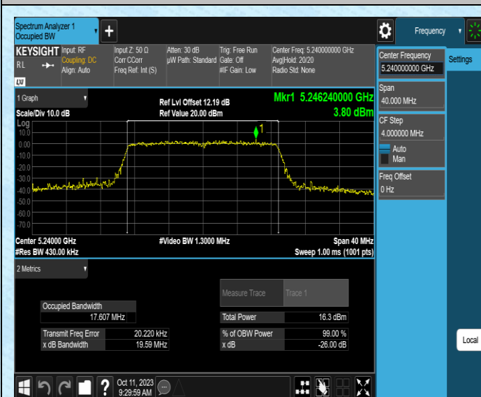
11AC20SISO-Ant1-5240
