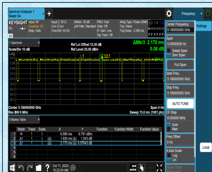
NTNV-11AC20MIMO-Ant1-5180
