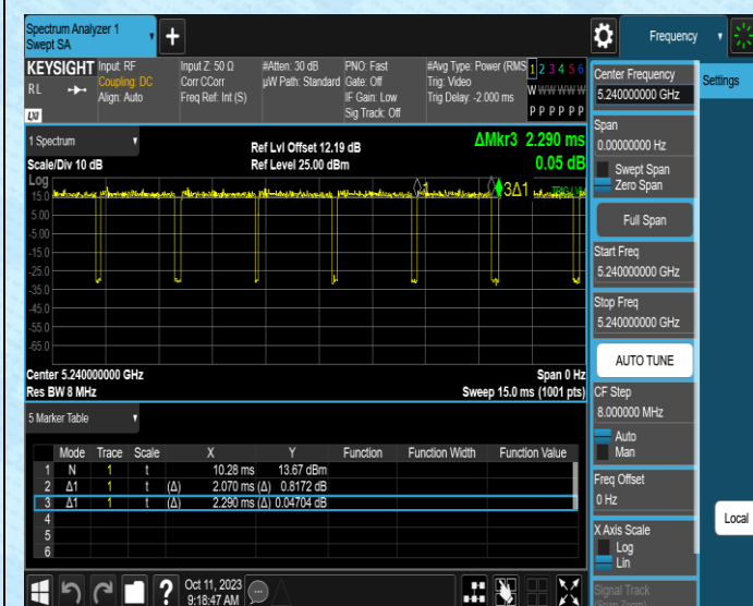
NTNV-11A-Ant1-5240
