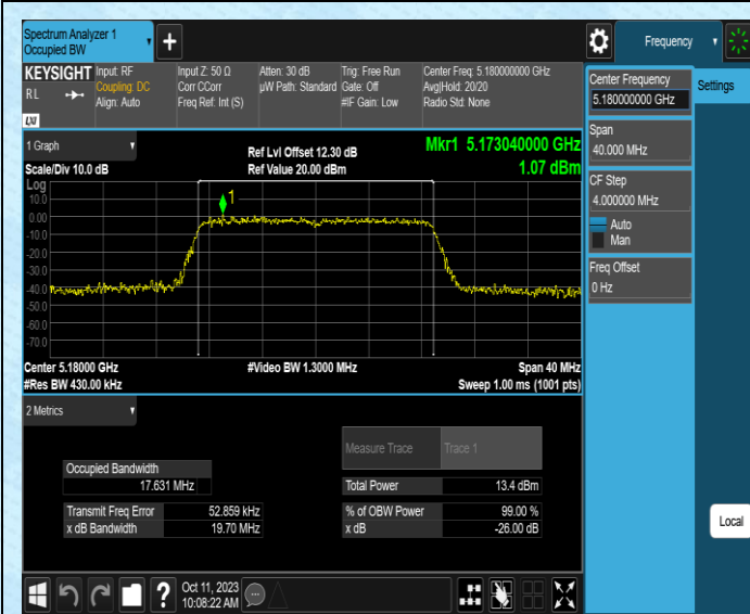
11N20MIMO-Ant1-5180
