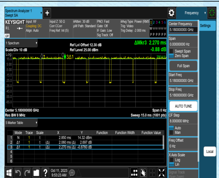
NTNV-11A-Ant2-5180
